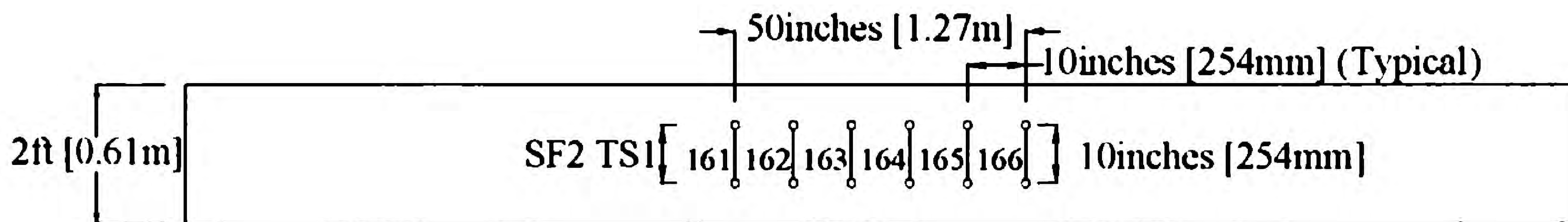
(a) Transverse Strain Locations on Small Face 2
