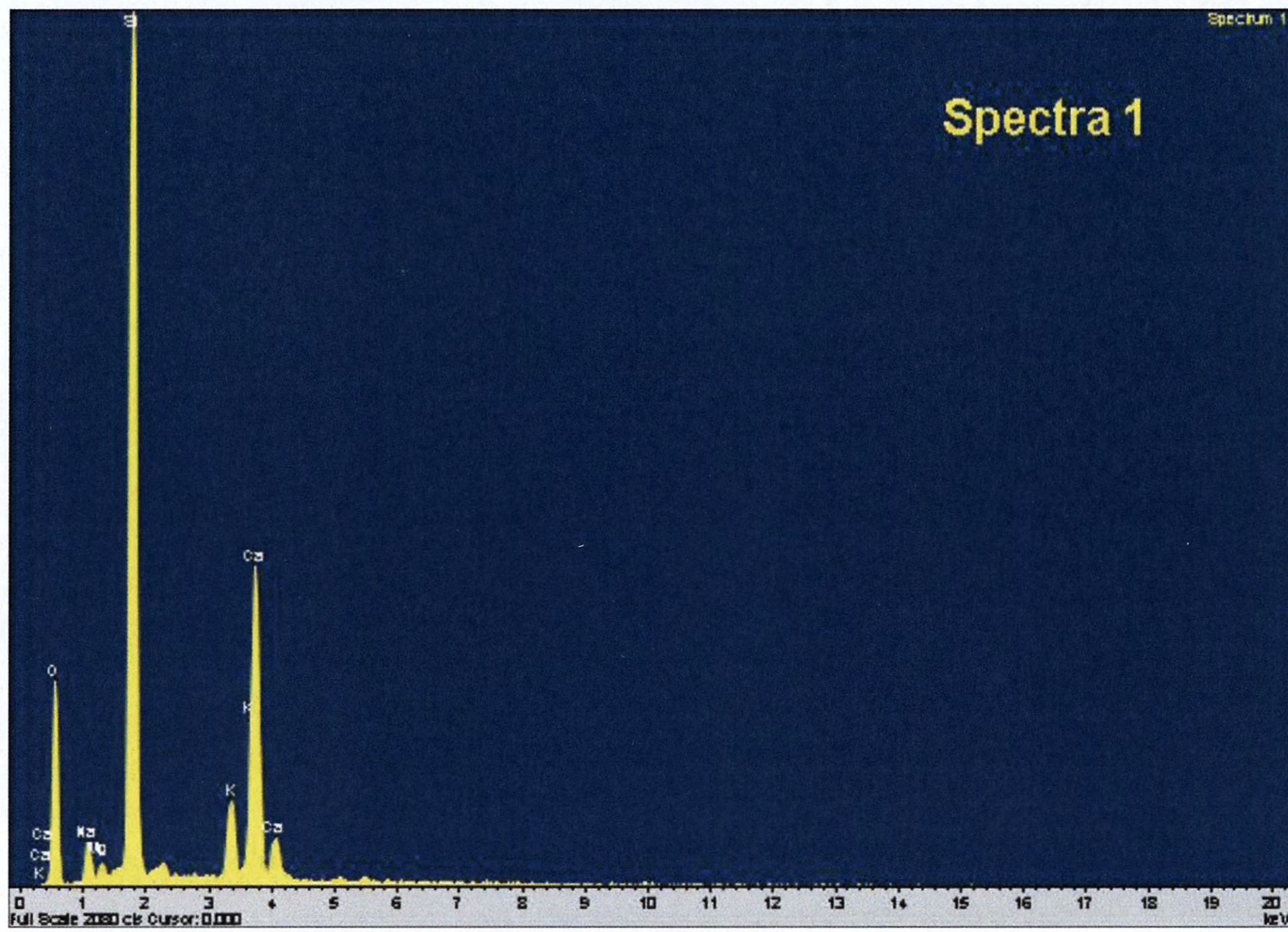
Spectra from previous BS image illustrating ASR gel chemistry
