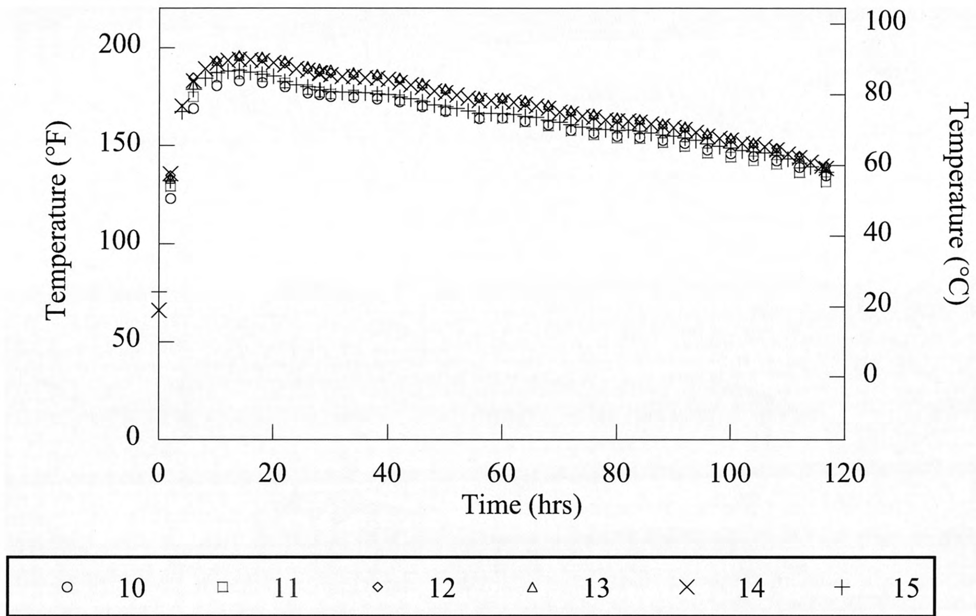
(a) Horizontal Thermocouple Measurements
