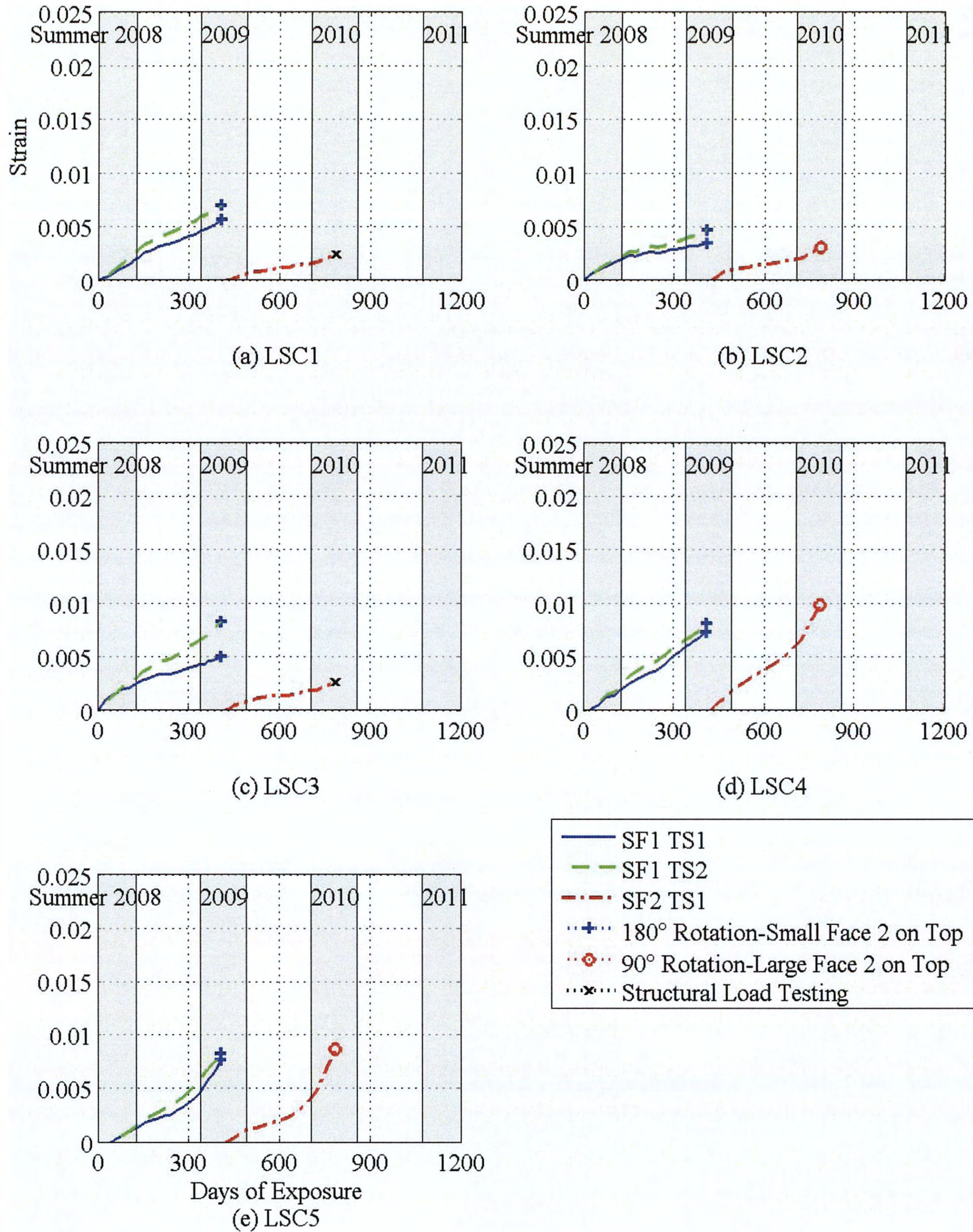
Figure 3-11. Transverse Surface Strains on the LSC Specimens' Small Face 1 and Small Face 2.
