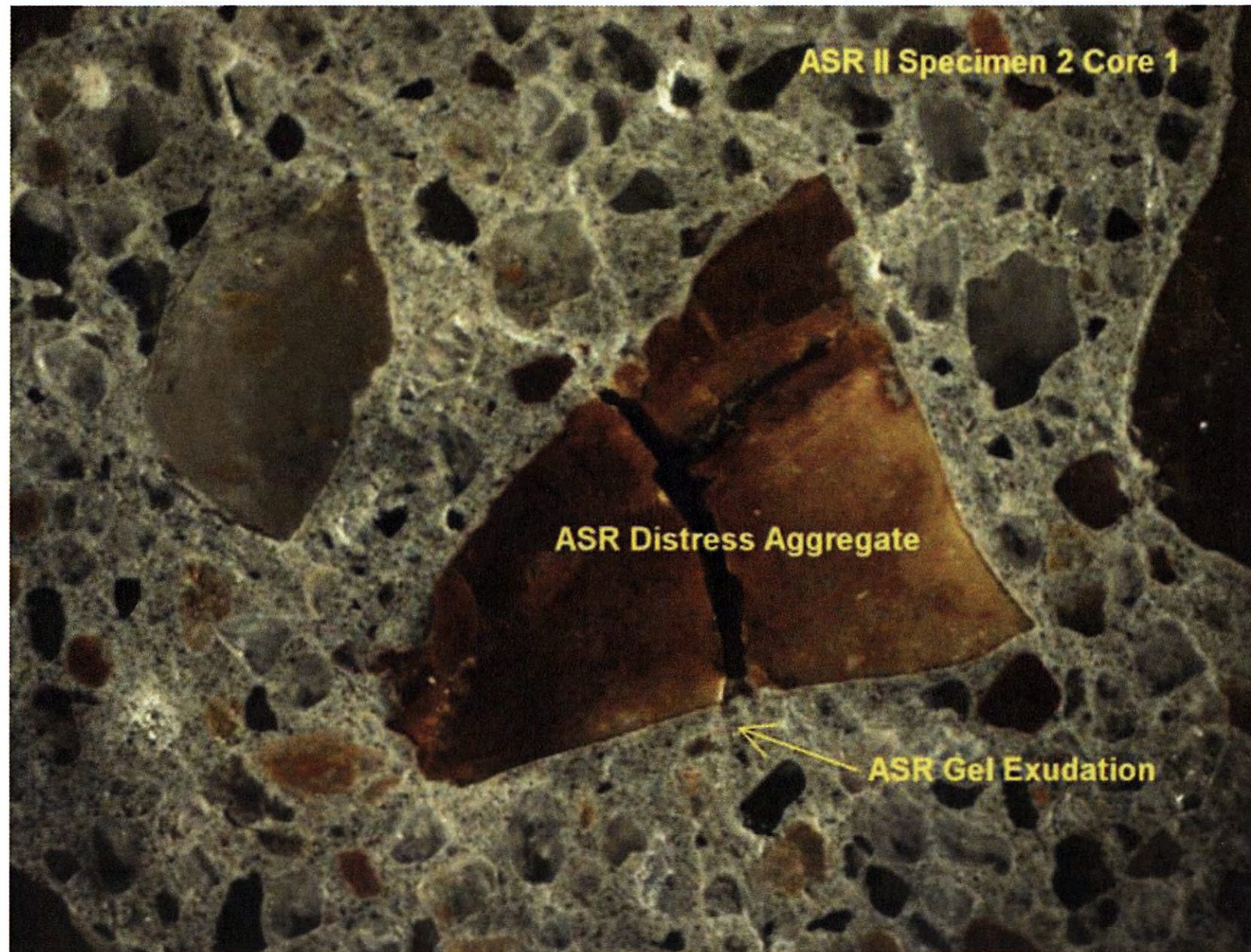
ASR Gel Exudation Noted from Reactive Aggregate Particle
