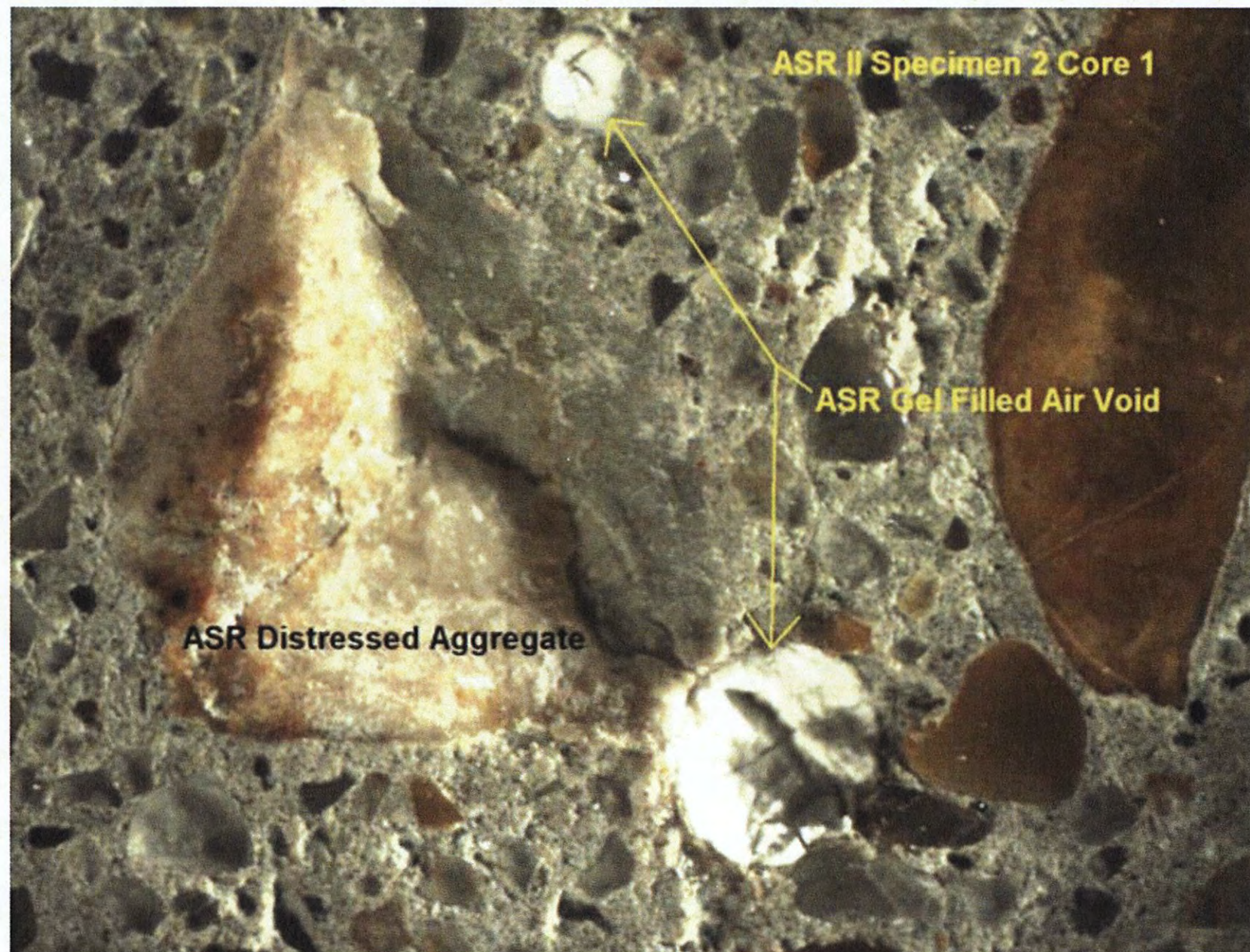
ASR Filled Air Voids Adjacent To Reactive Particle
