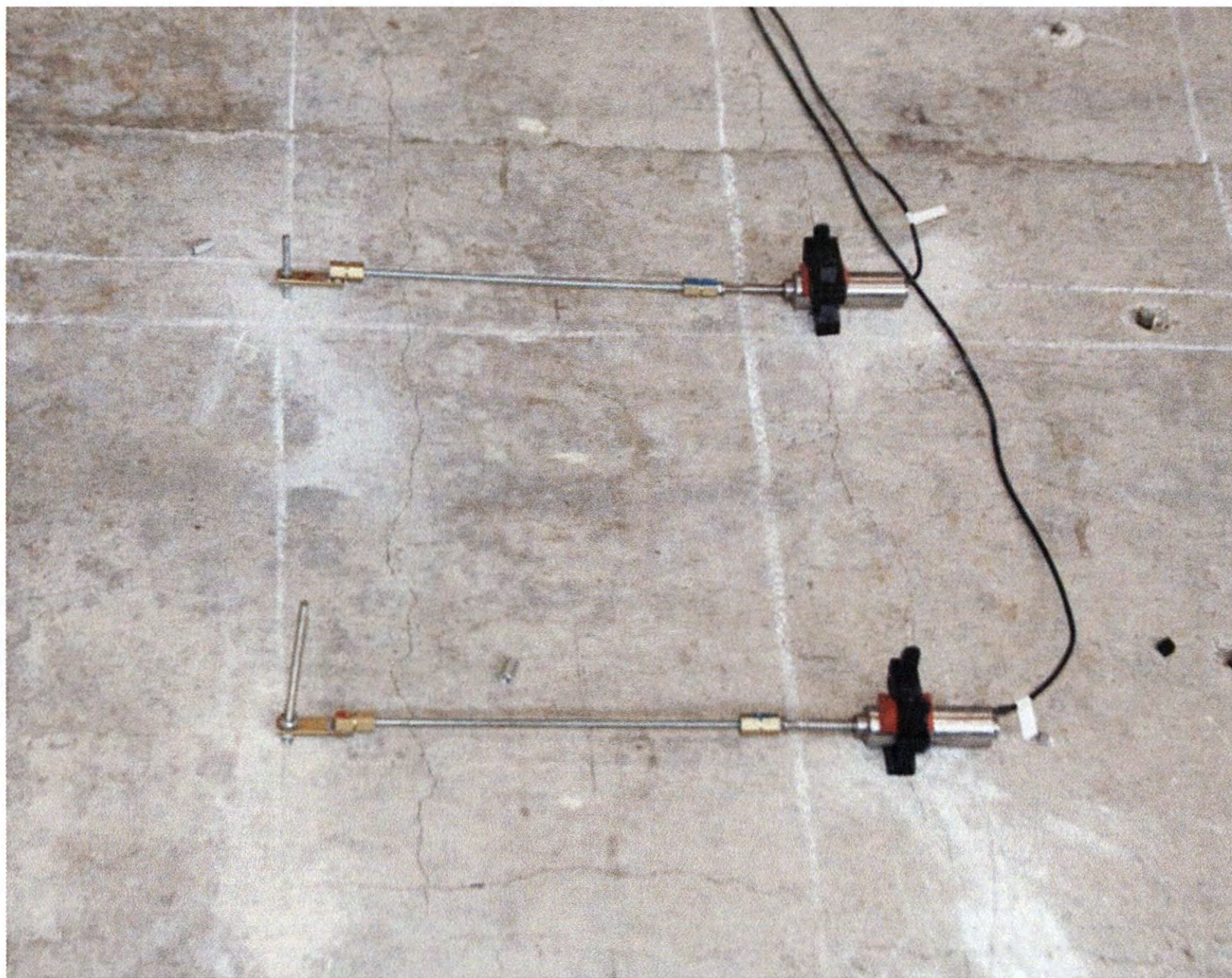
Figure 5-7. LVDT Installation prior to Testing.
