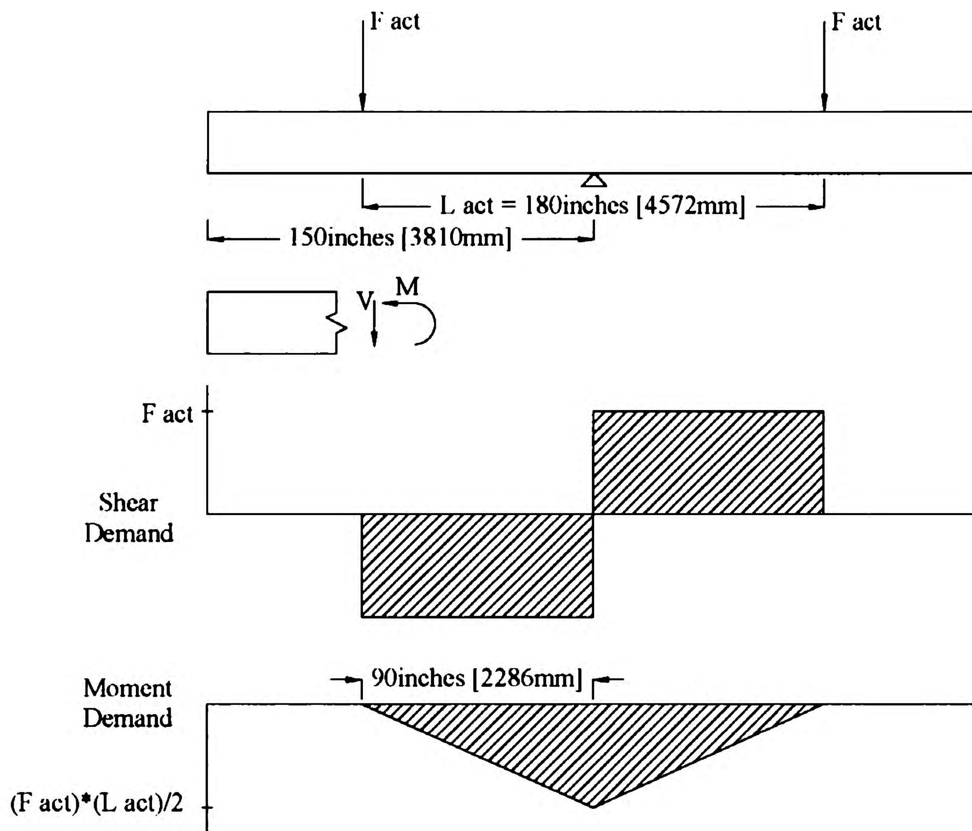
Figure 4-18. Three-Point Test Shear and Moment Diagram.
