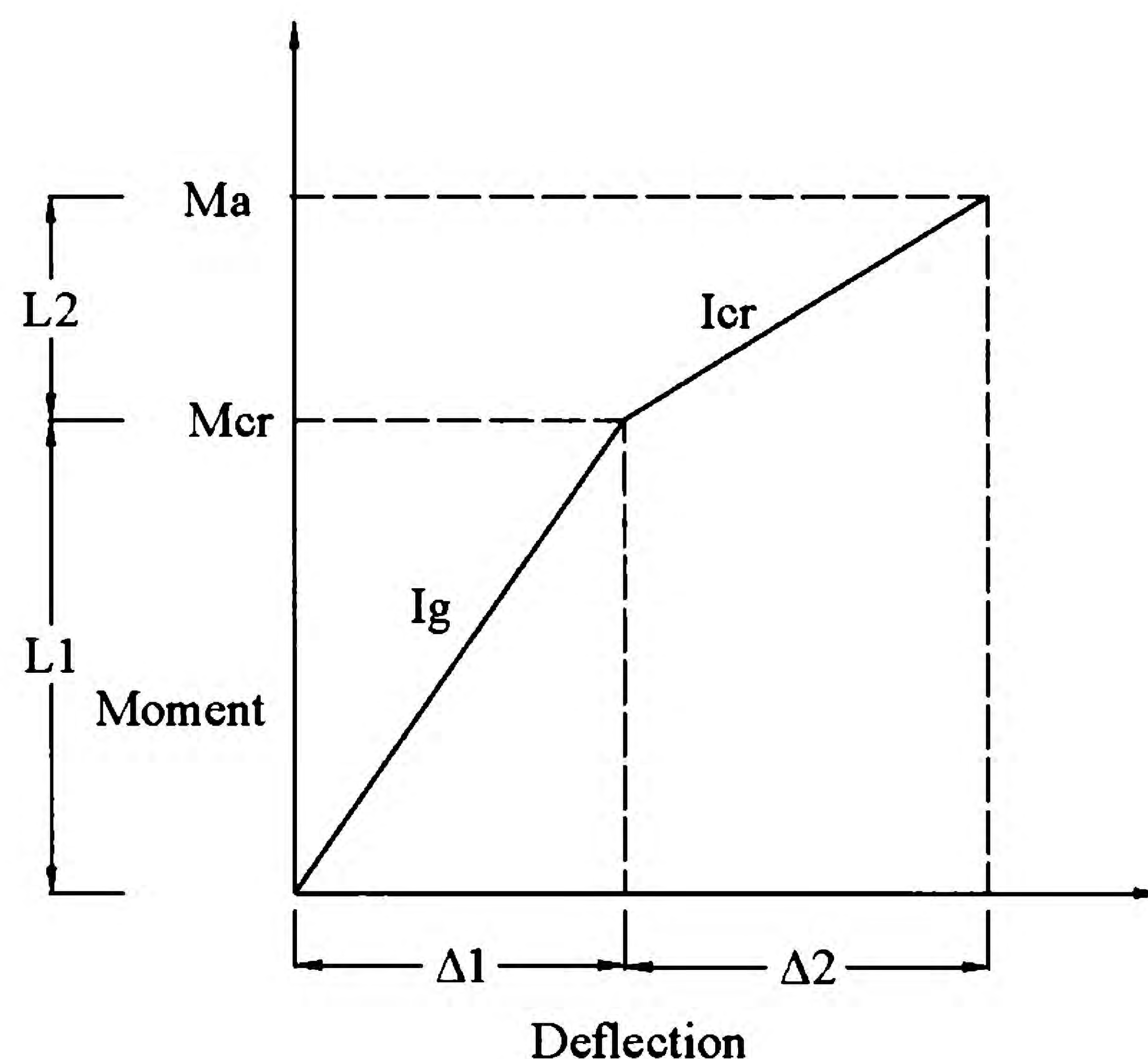
Figure 4-15. Bilinear Moment vs. Deflection Relation (Naaman 2004).
