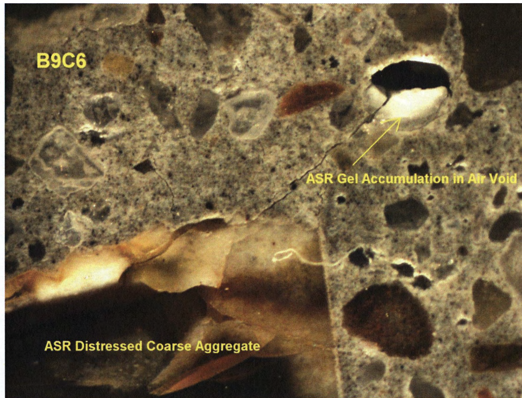
Figure 3-32. ASR Gel Accumulation and Distressed Coarse Aggregate.
