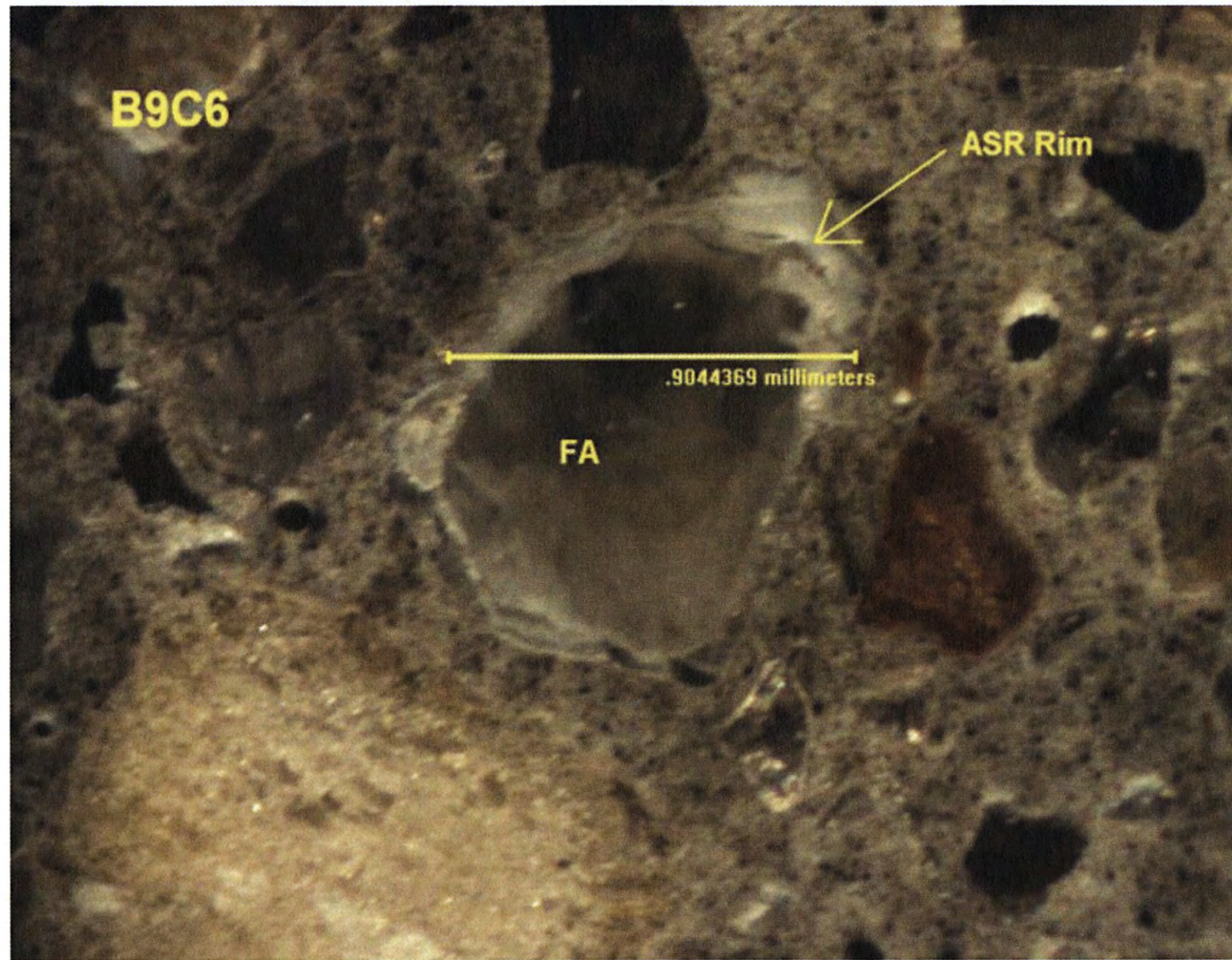
ASR gel rim observed around fine aggregate
