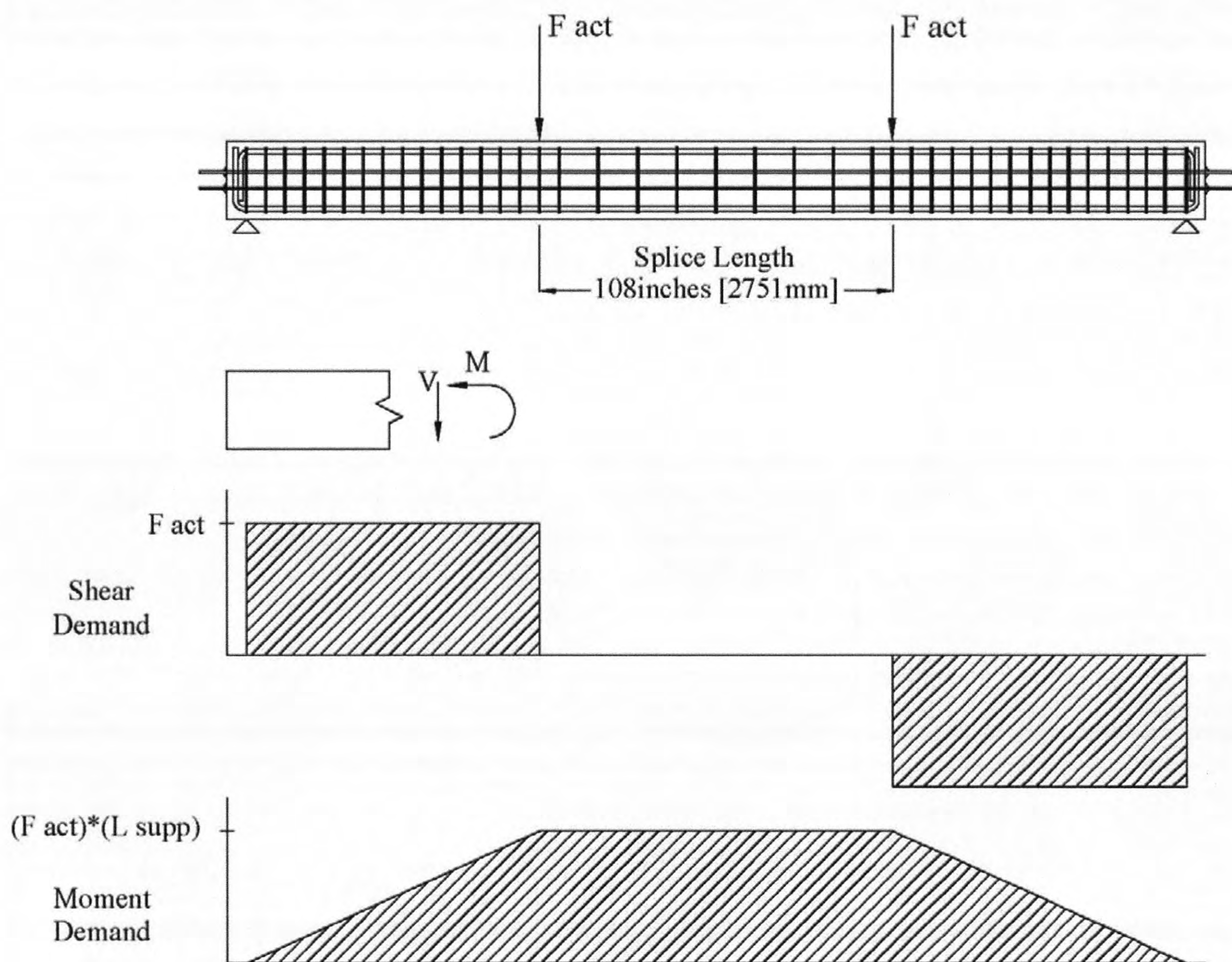
Figure 5-1. Four-Point Load Test Setup and Demand Loading.
