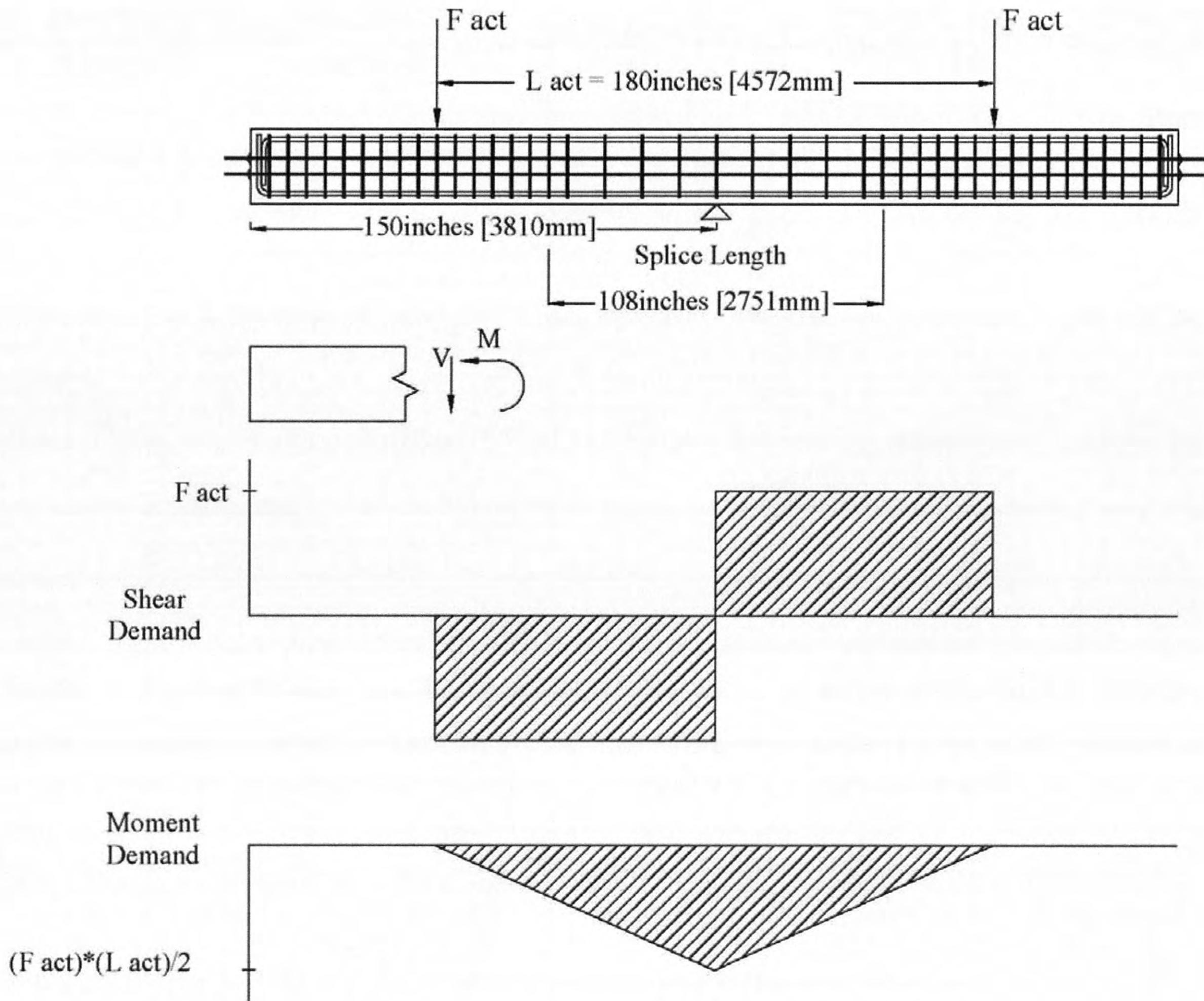
Figure 2-6. Three-Point Load Test.
