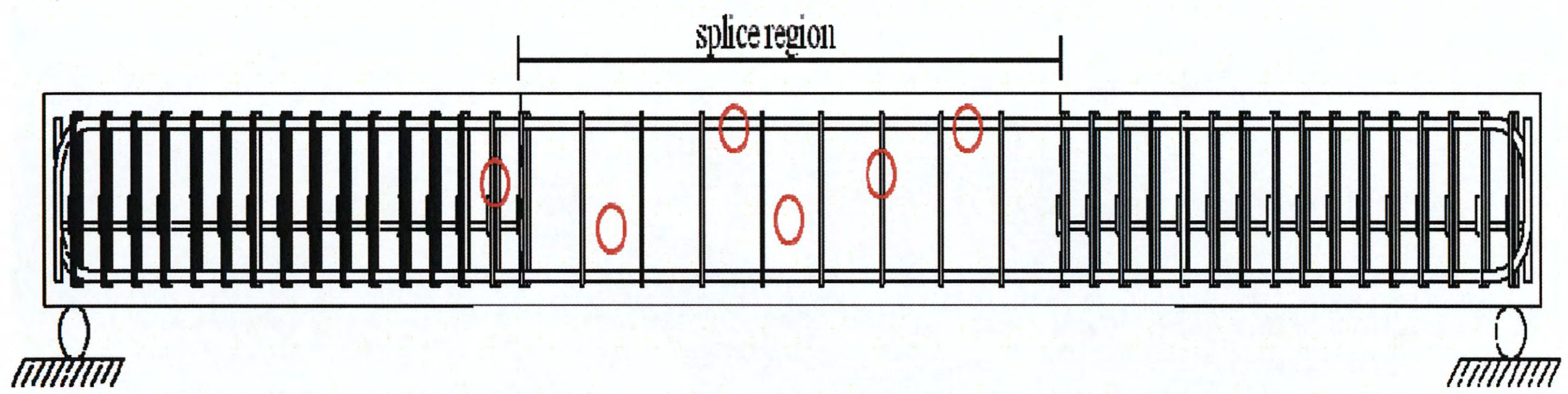
Figure 3-28. Typical Coring Locations.
