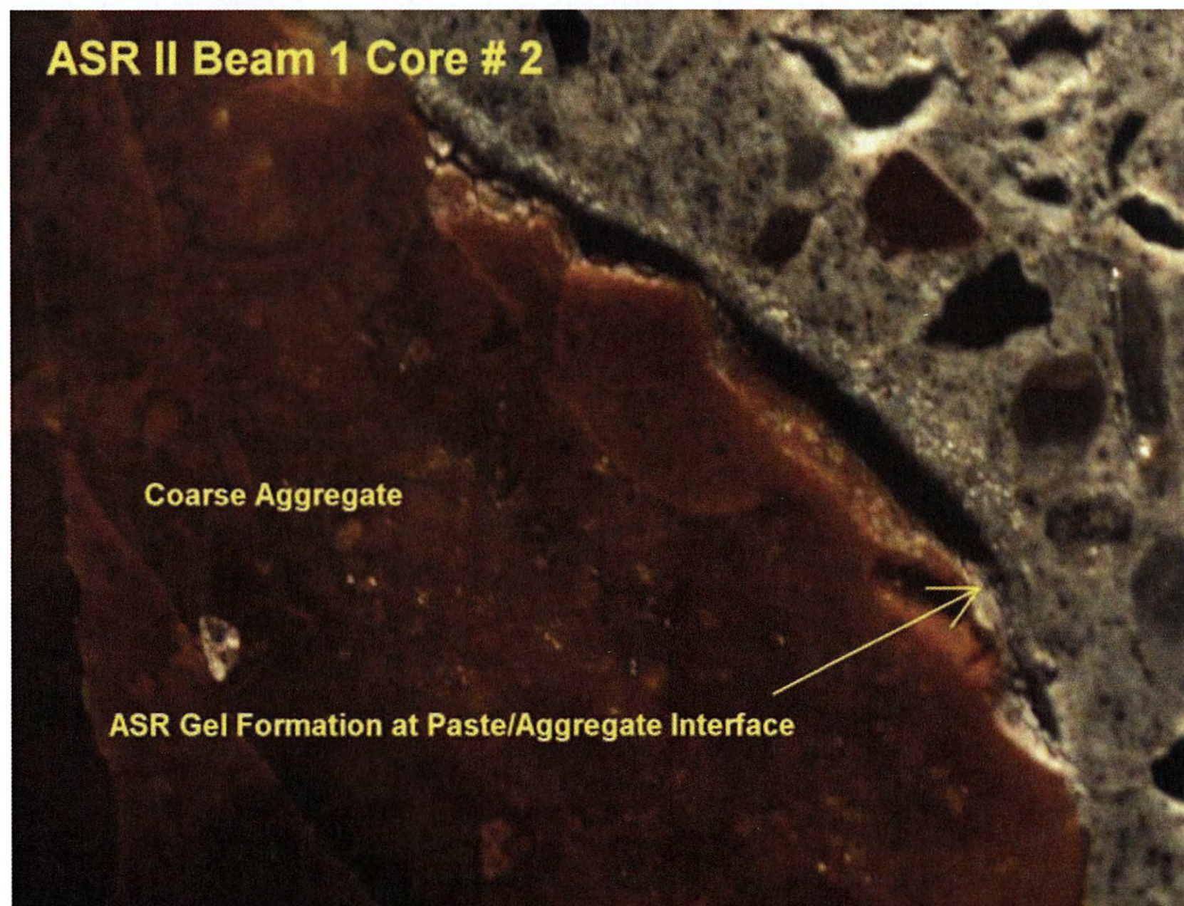
Small accumulation of ASR gel near paste/aggregate interface
