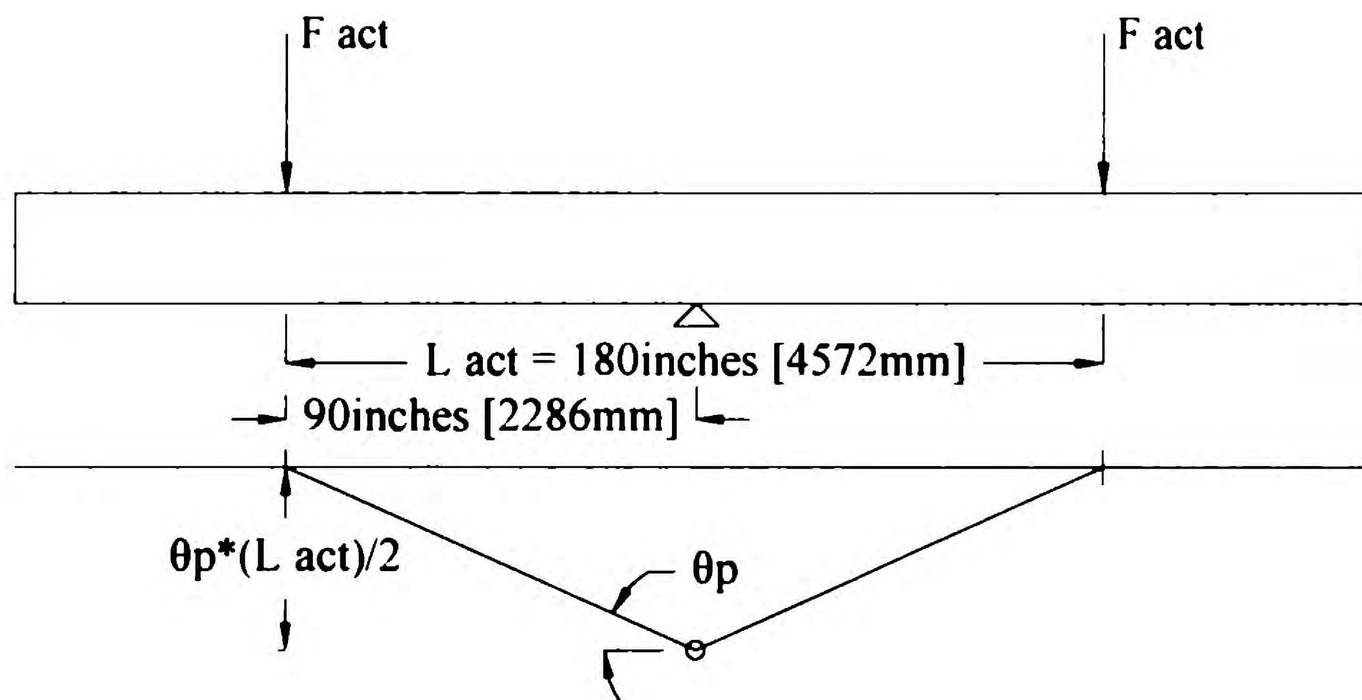
Figure 4-24. Plastic Hinge Rotation for the Three-Point Setup.
