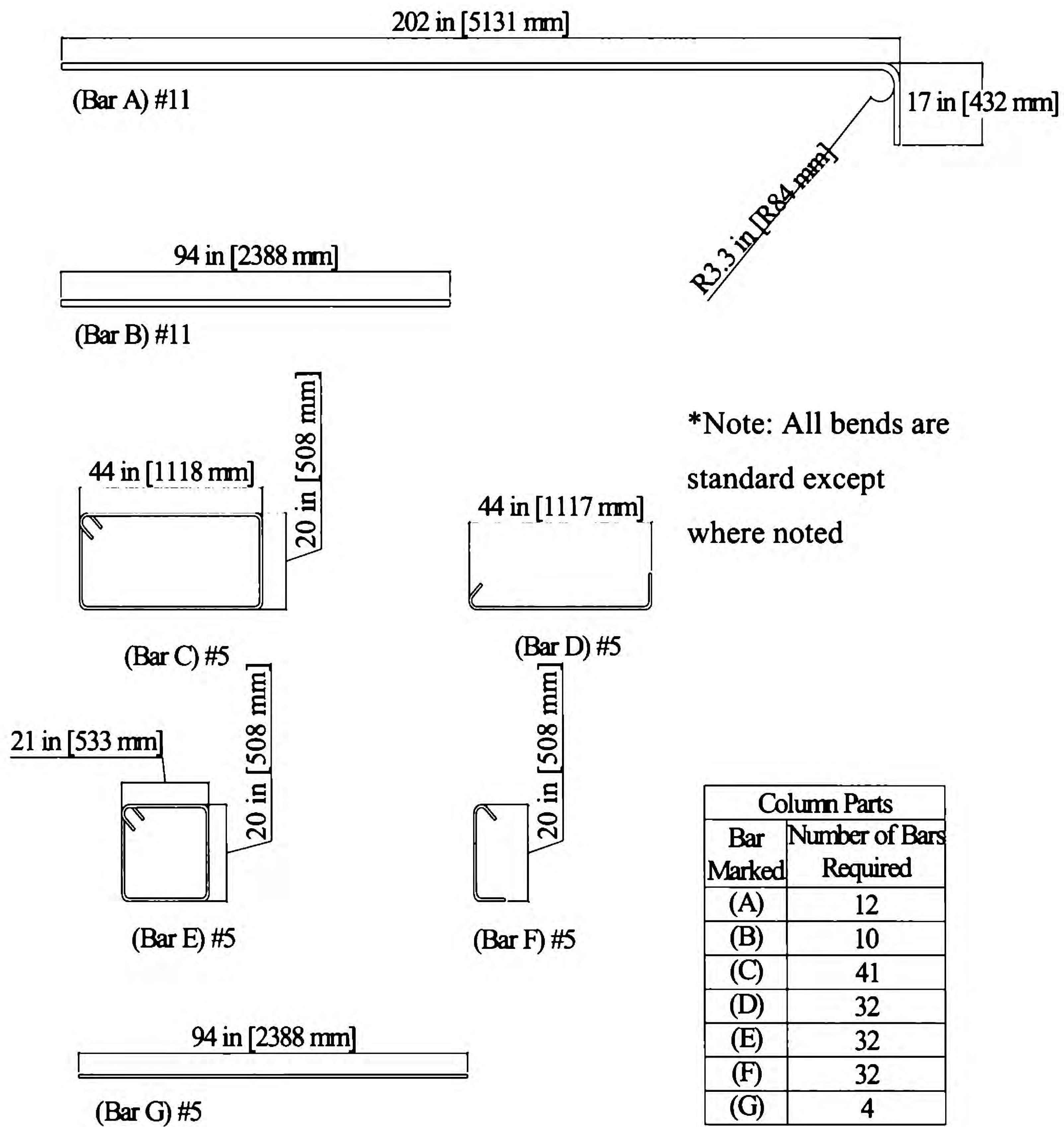
Figure 2-12. Reinforcement Types, Quantities, and Dimensions.
