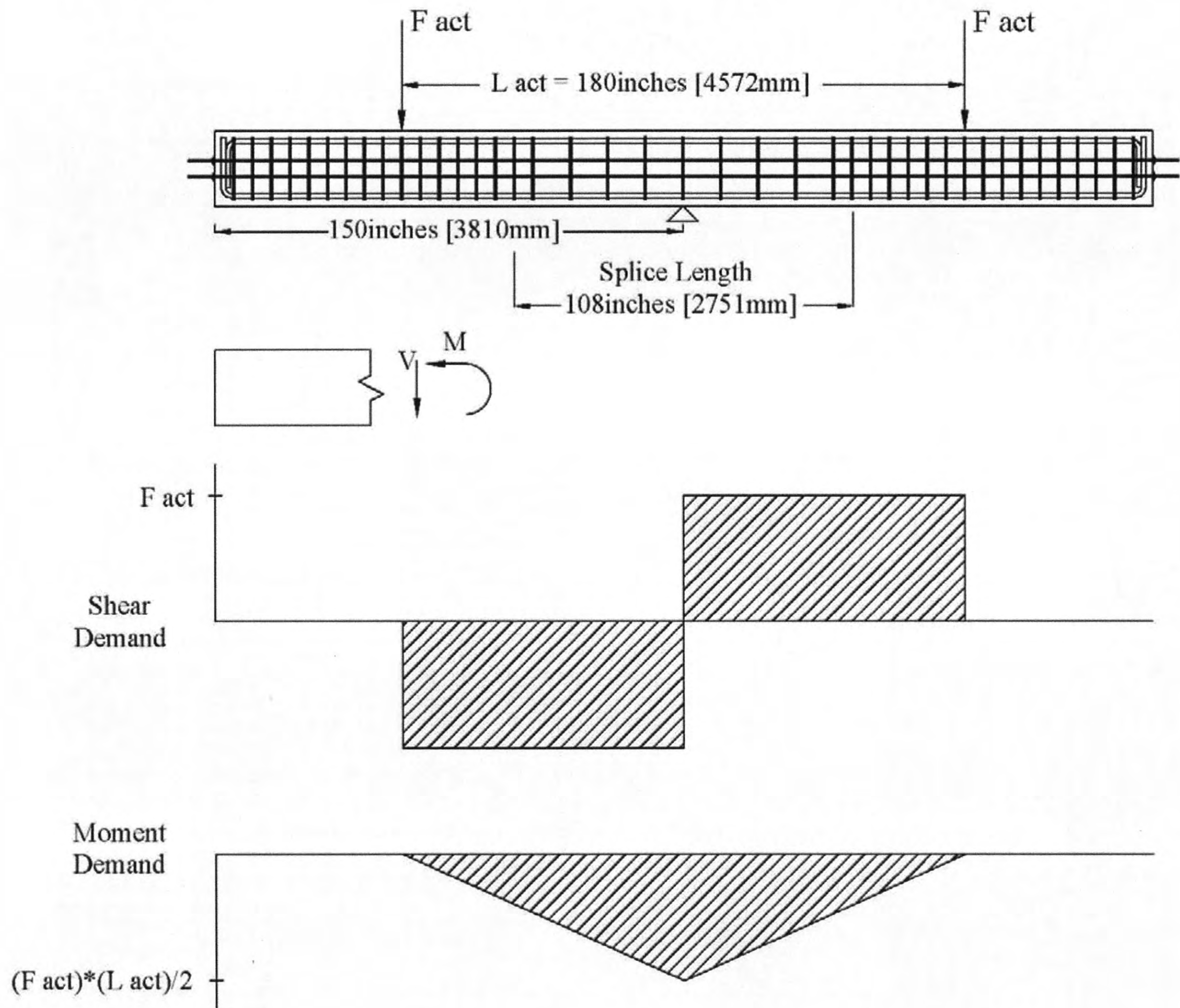
Figure 5-12. Three-Point Load Test Setup and Demand Loading.
