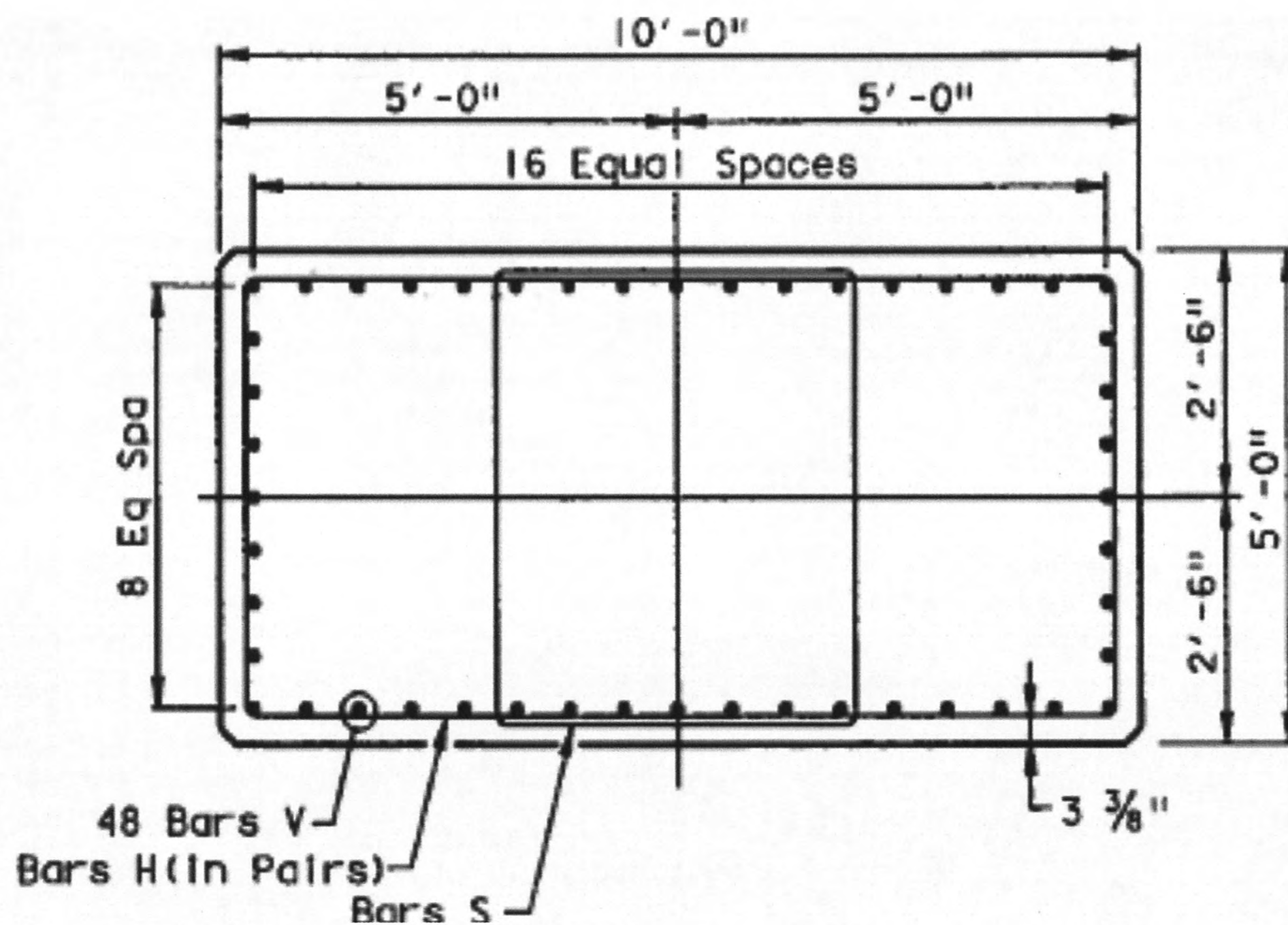
Figure 2-2. Section B-B of the Sample Column.
