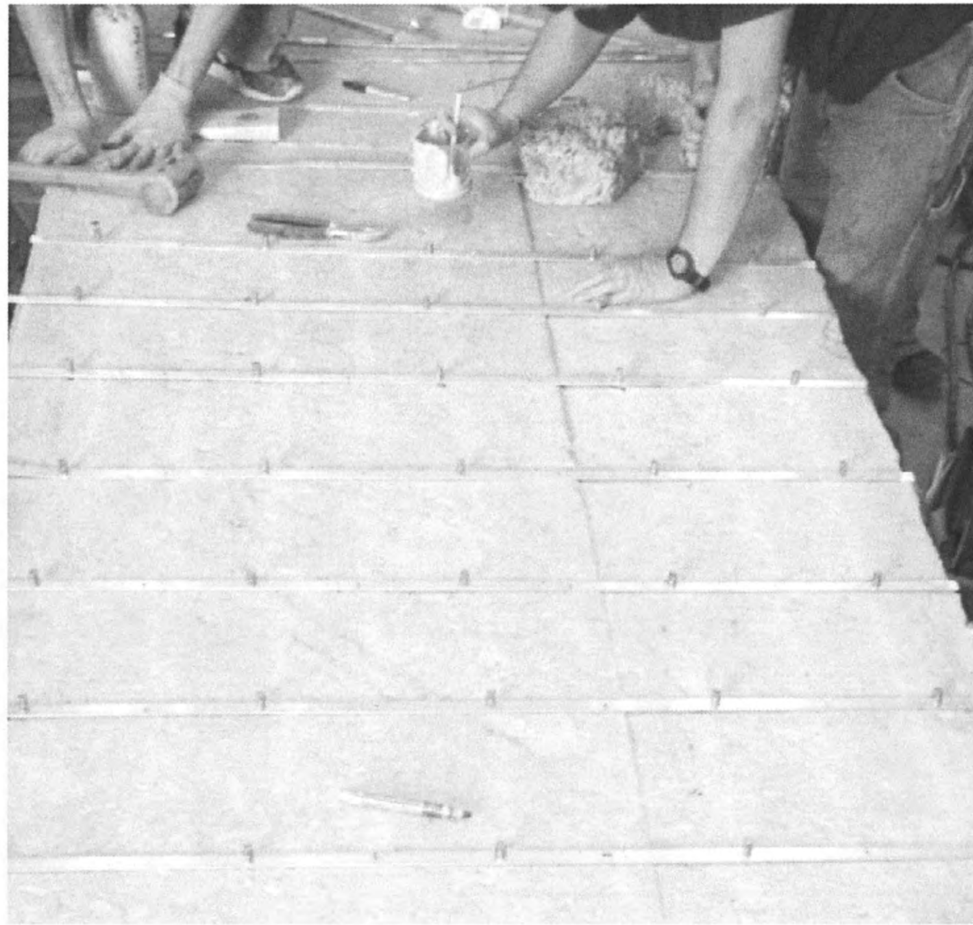
Figure 2-26. DEMEC Installation on the LSC Specimen's Large Face 1.
