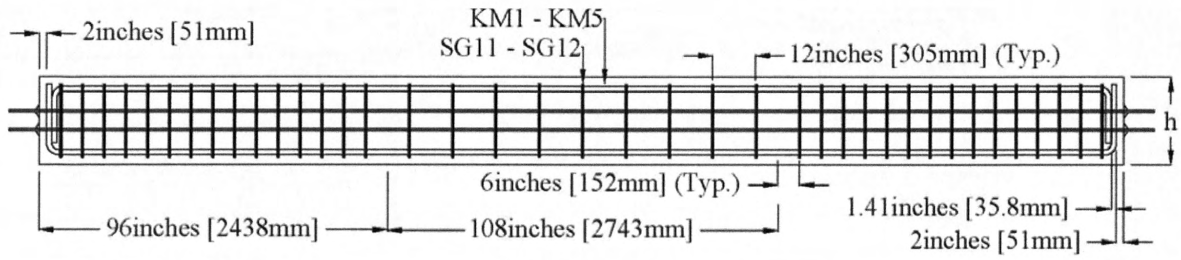
Elevation View
