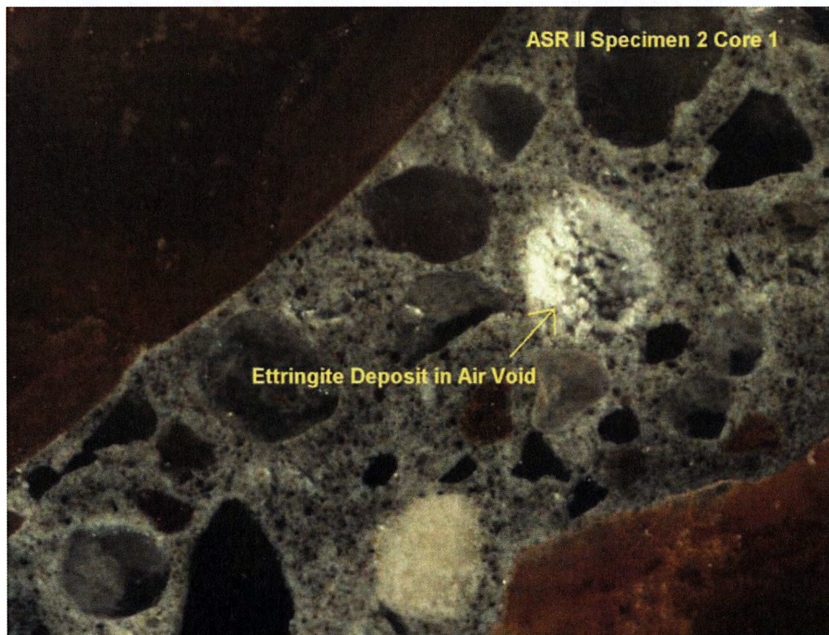
Accumulation of Ettringite in Air Void
