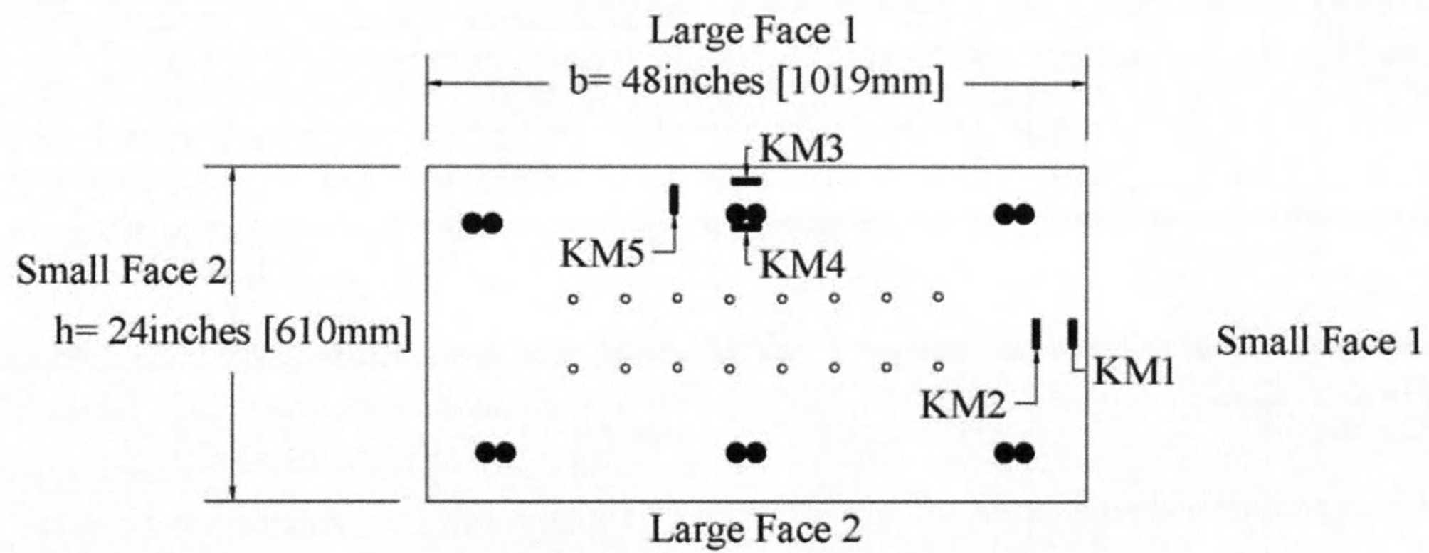
(c) Cross Section with KM1-KM5
