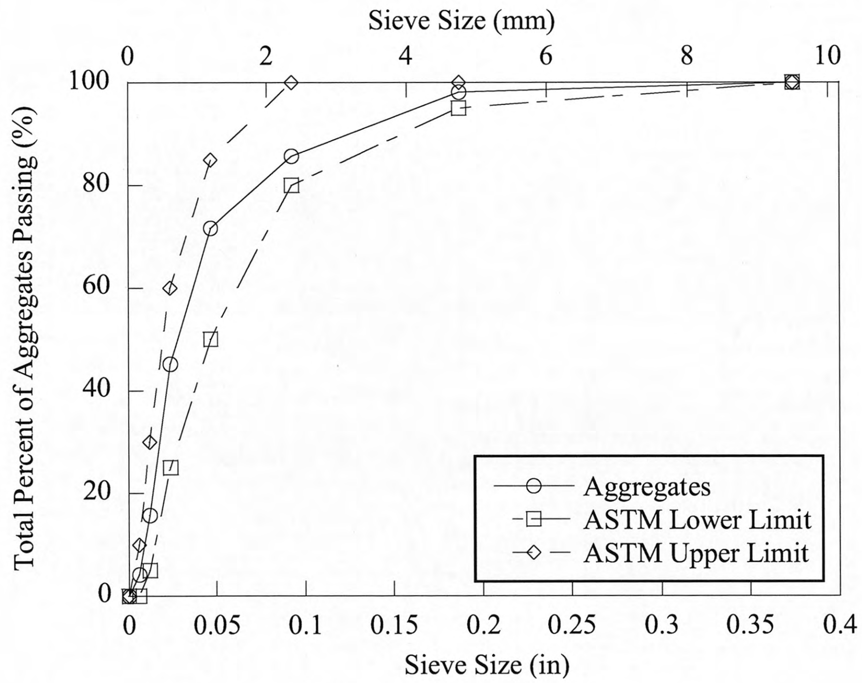
Figure 2-10. Gradation of the Fine Aggregates.
