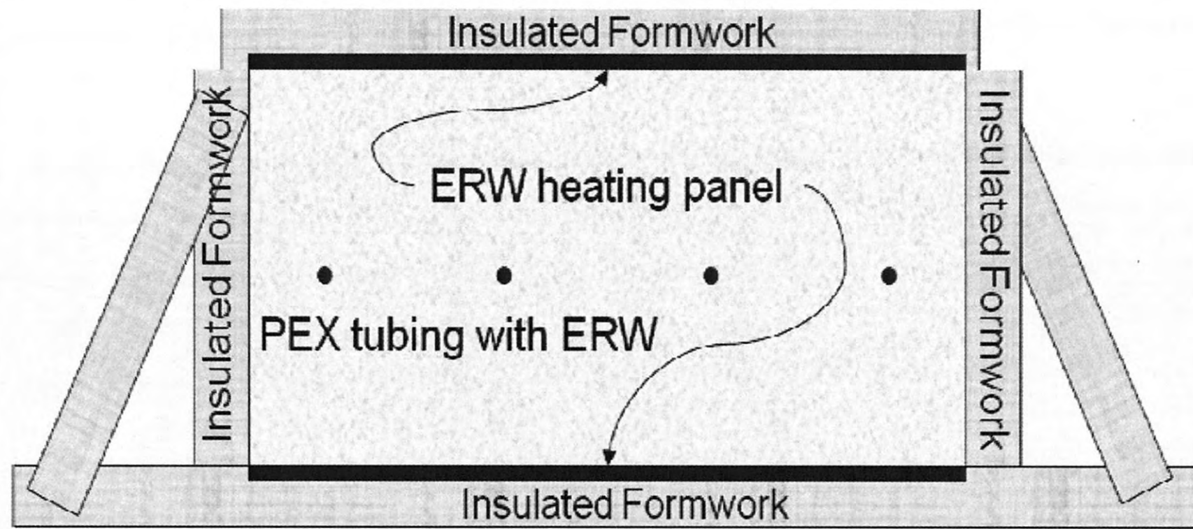
End-View of Heated Formwork
