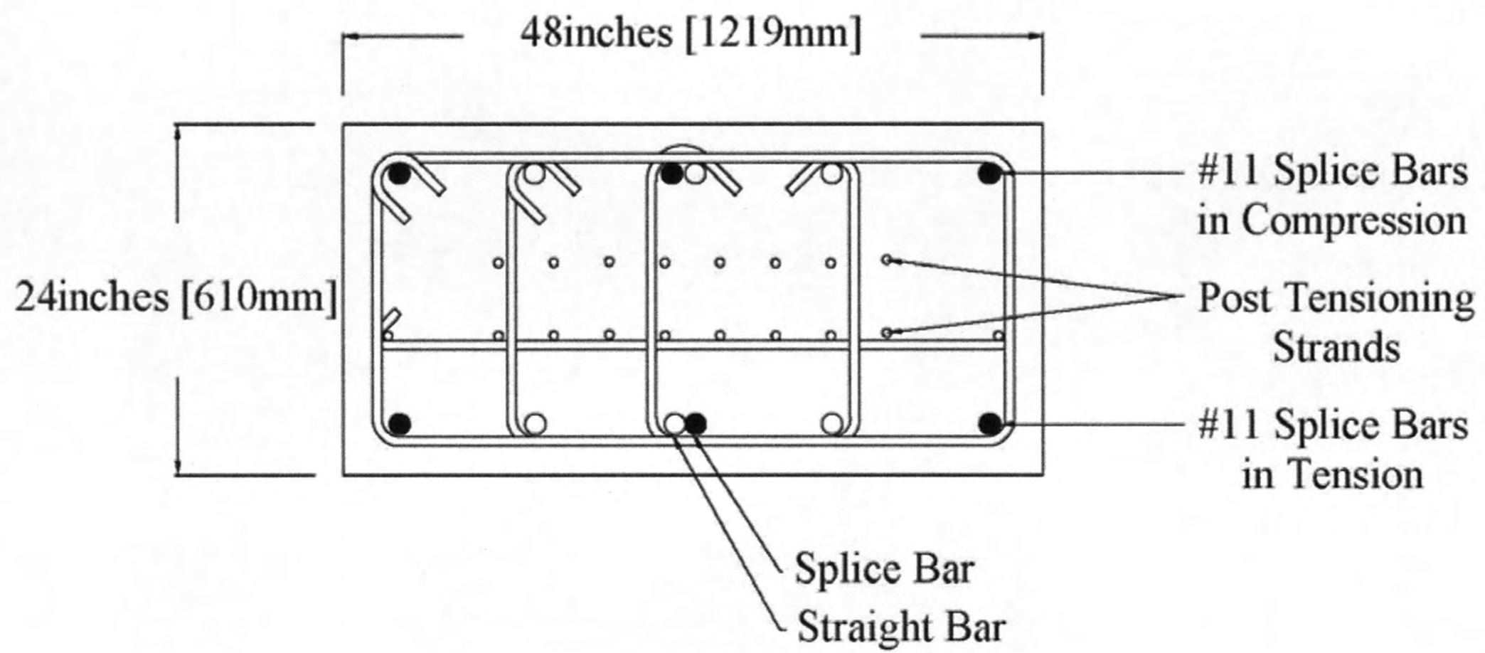
Figure 4-4. Cross Section at End Region.
