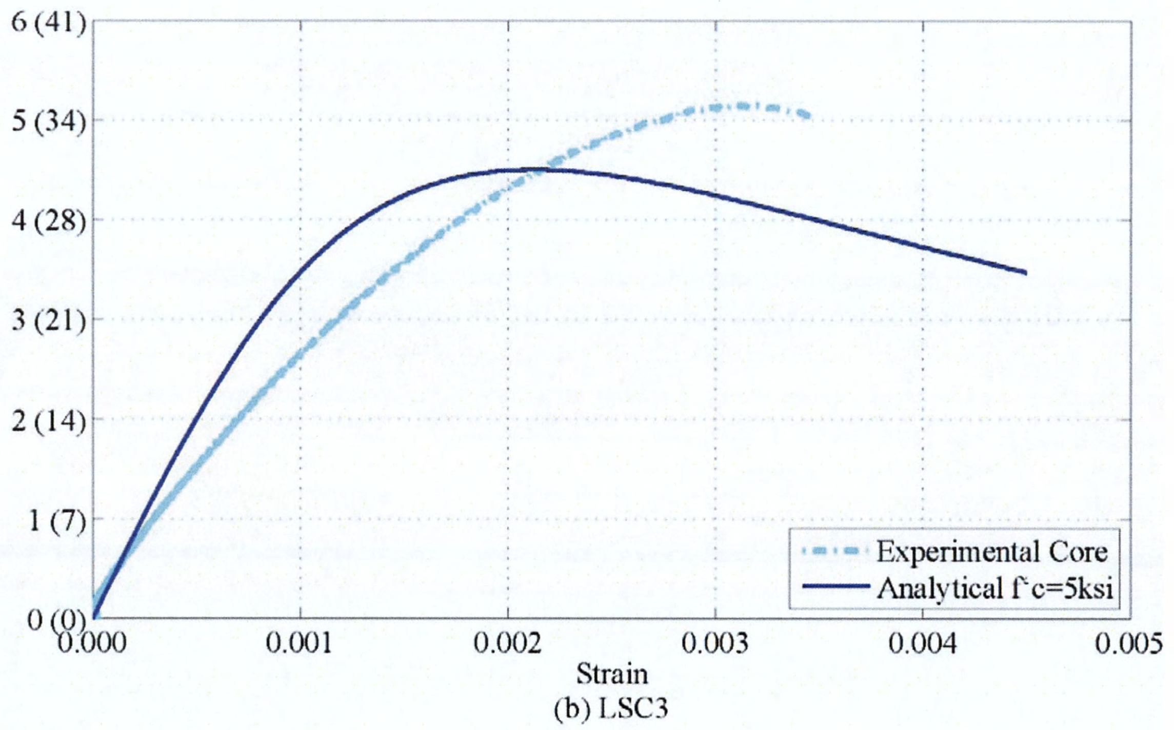
Figure 5-18. Compression Stress-Strain Response for LSC1 and LSC3 Cores.
