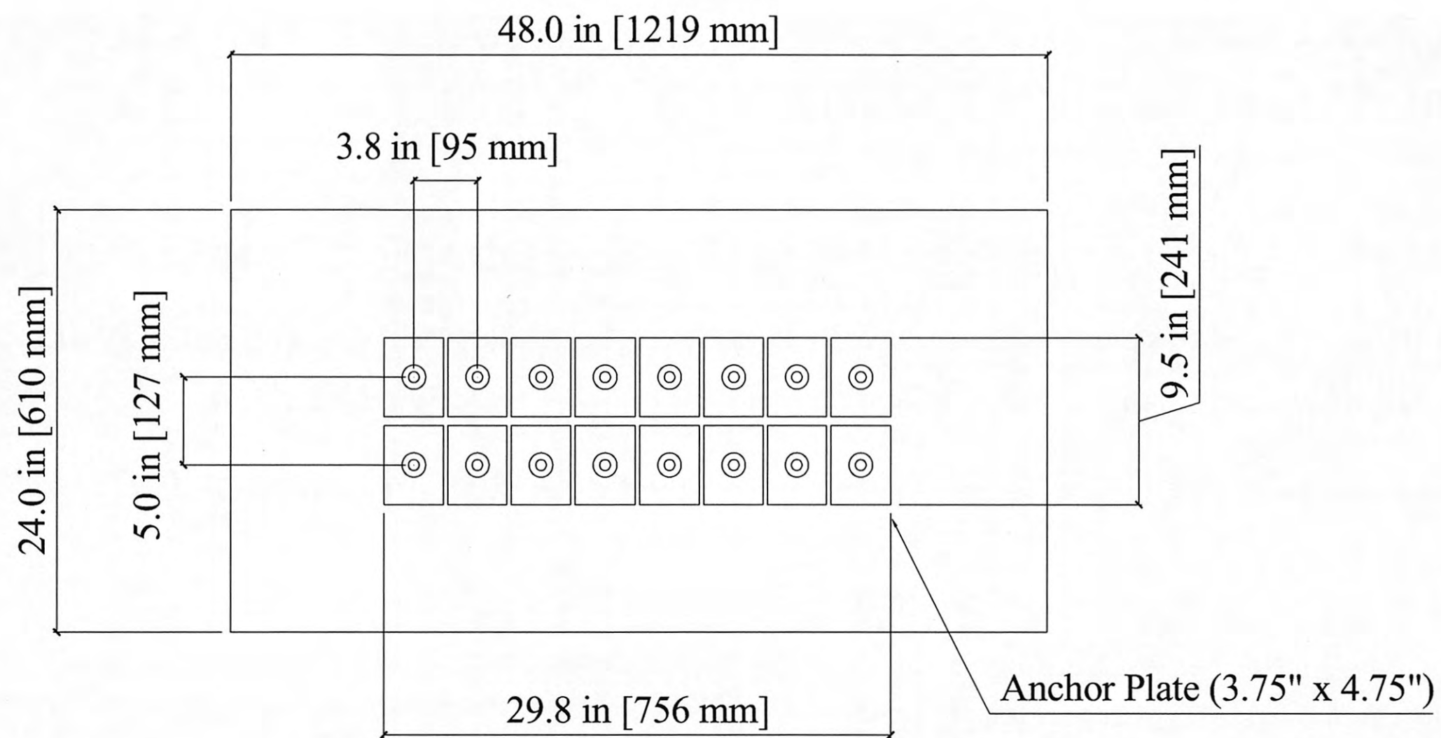
Figure 2-7. Strand Layout (End View).
