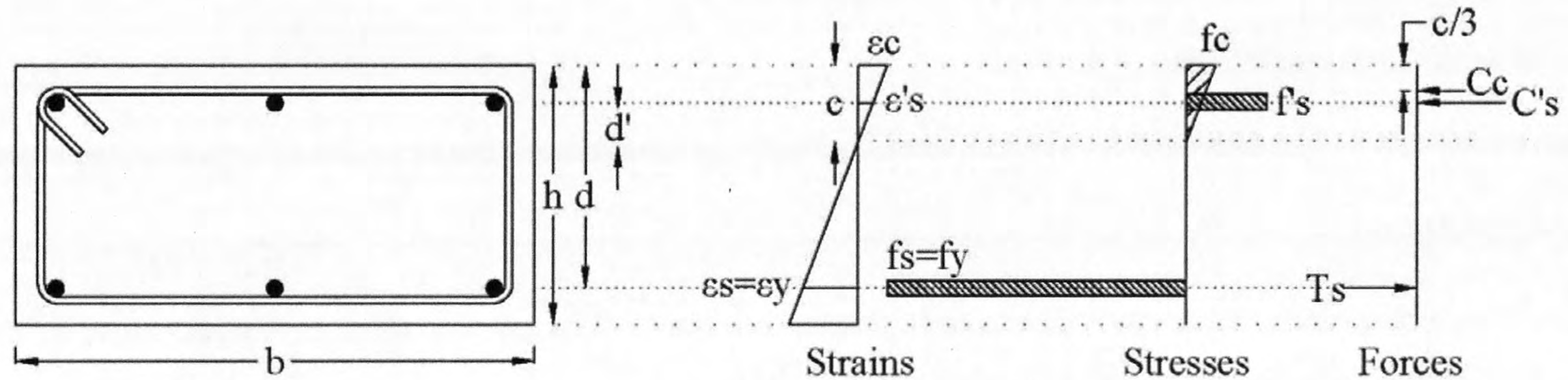
First Yielding of Reinforcing Steel
