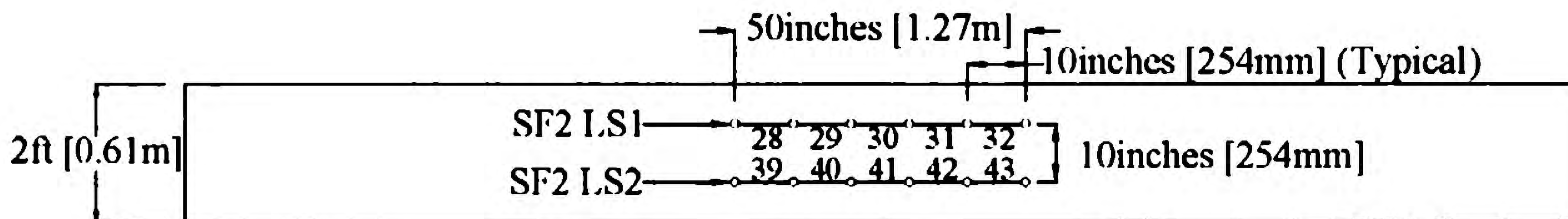
(b) Longitudinal Strain Locations on Small Face 2
