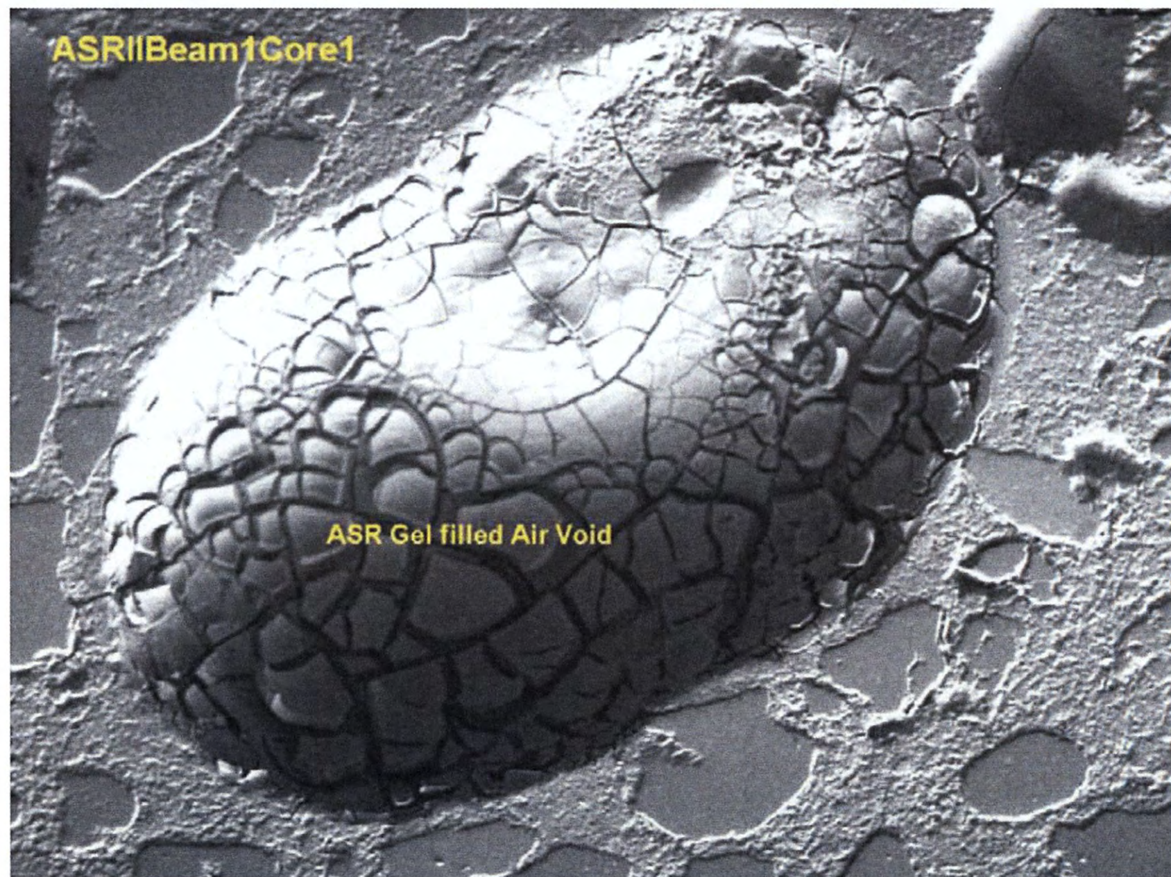
ASR gel accumulation in elongated air void
