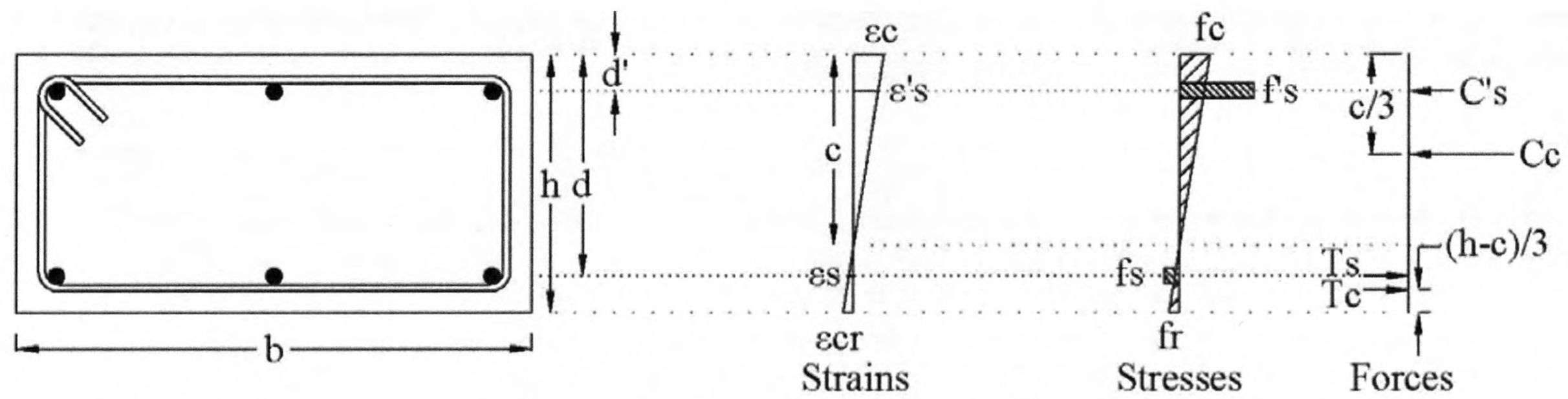
First Cracking of Concrete in Tension
