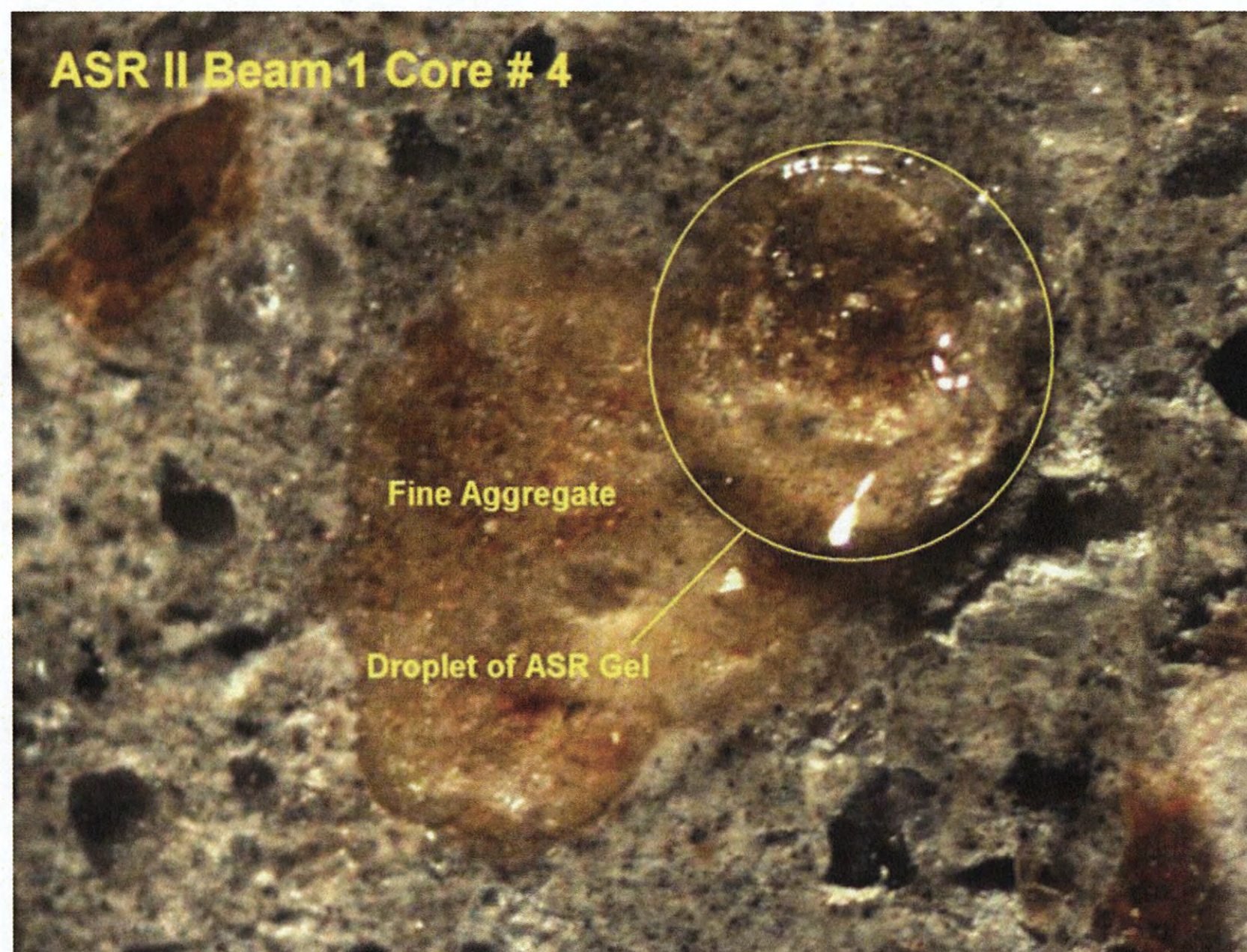
Small droplet of ASR gel which oozed out of fine aggregate
