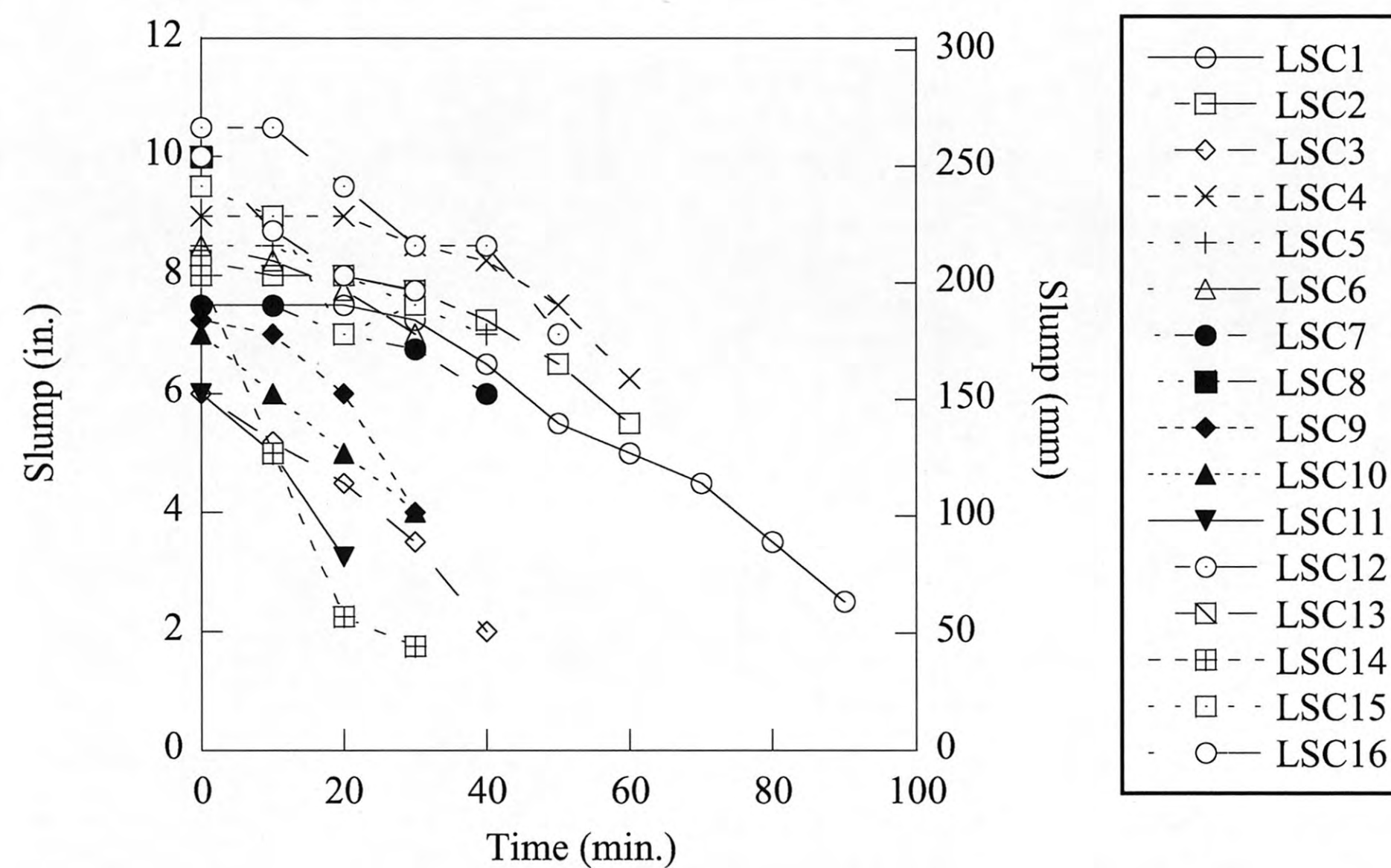
Figure 2-20. Slump versus Time.
