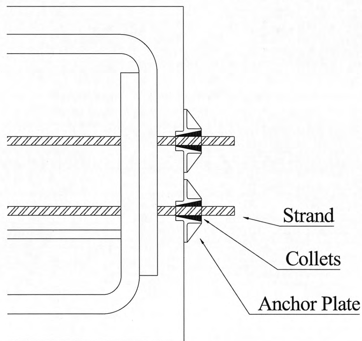
Figure 2-8. Strand End Termination.
