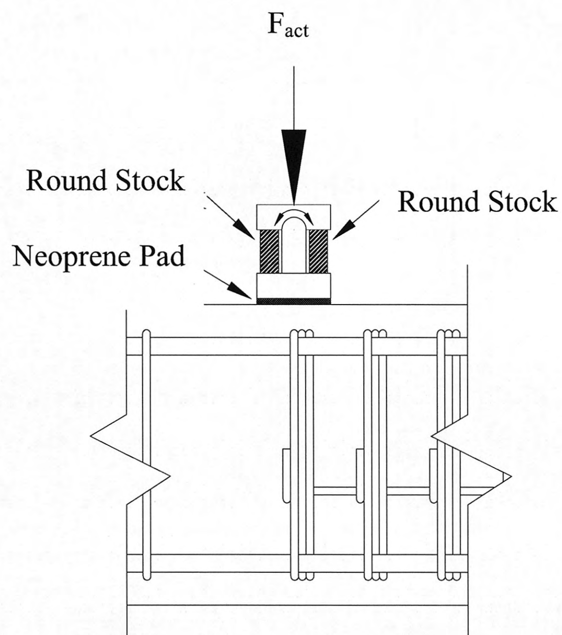
Figure 5-3. "Fixed" Support Setup.
