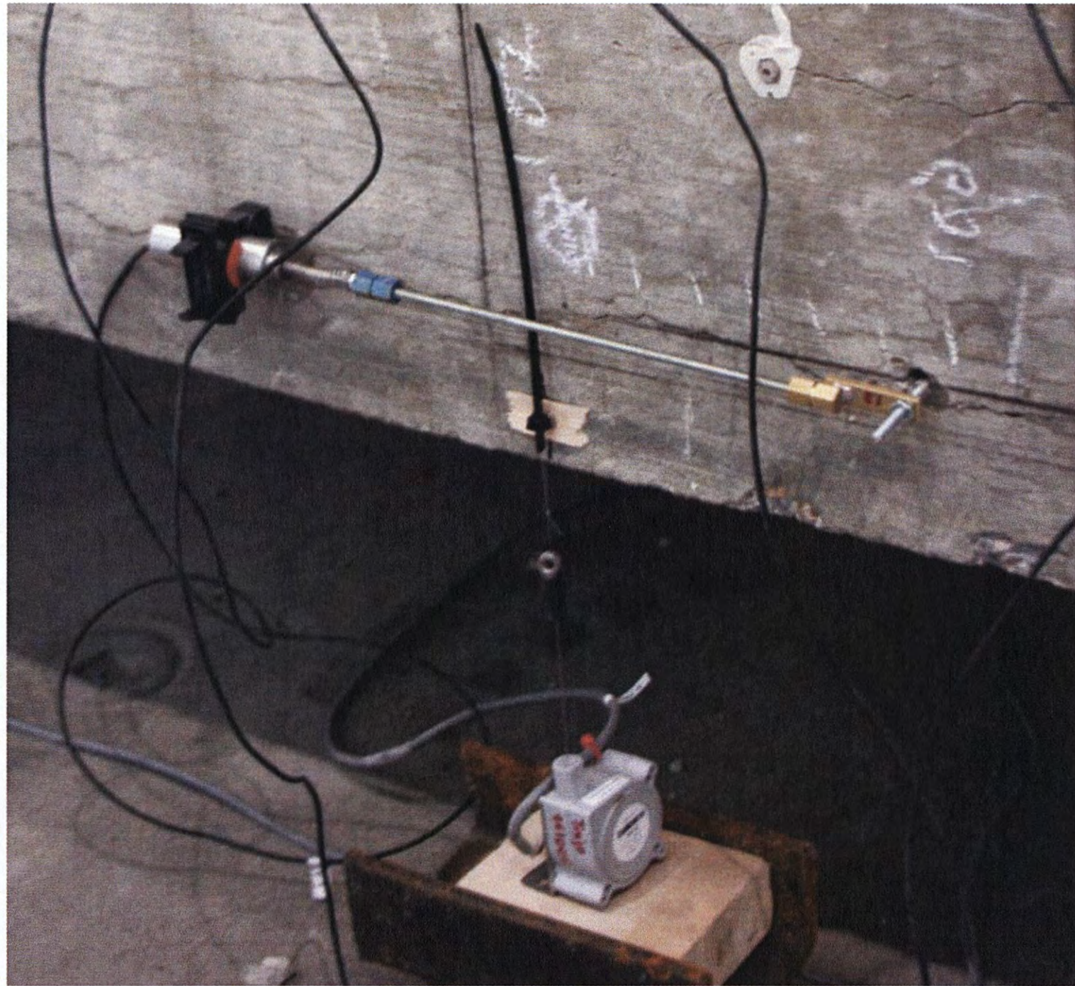
Figure 5-5. STR Installation Prior to Testing.
