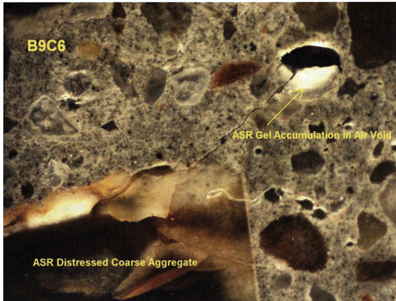
Distress and gel accumulation observed from chert coarse aggregate
