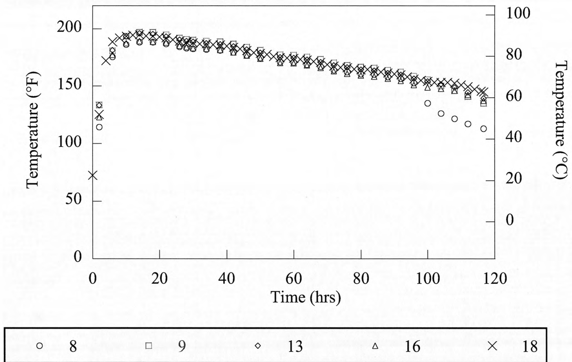
(b) Vertical Thermocouple Measurements
