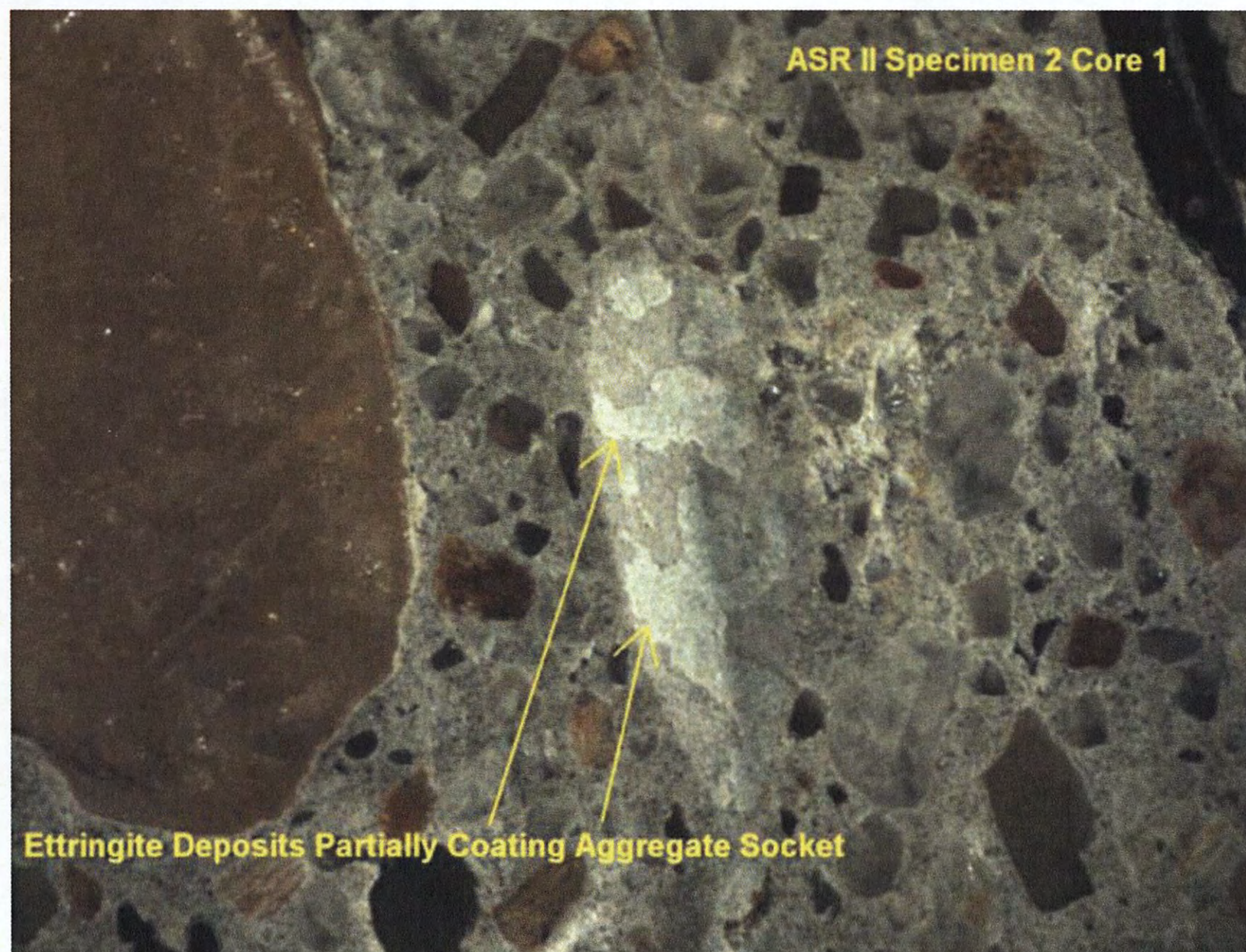
Partial Coating of Ettringite within Aggregate Socket
