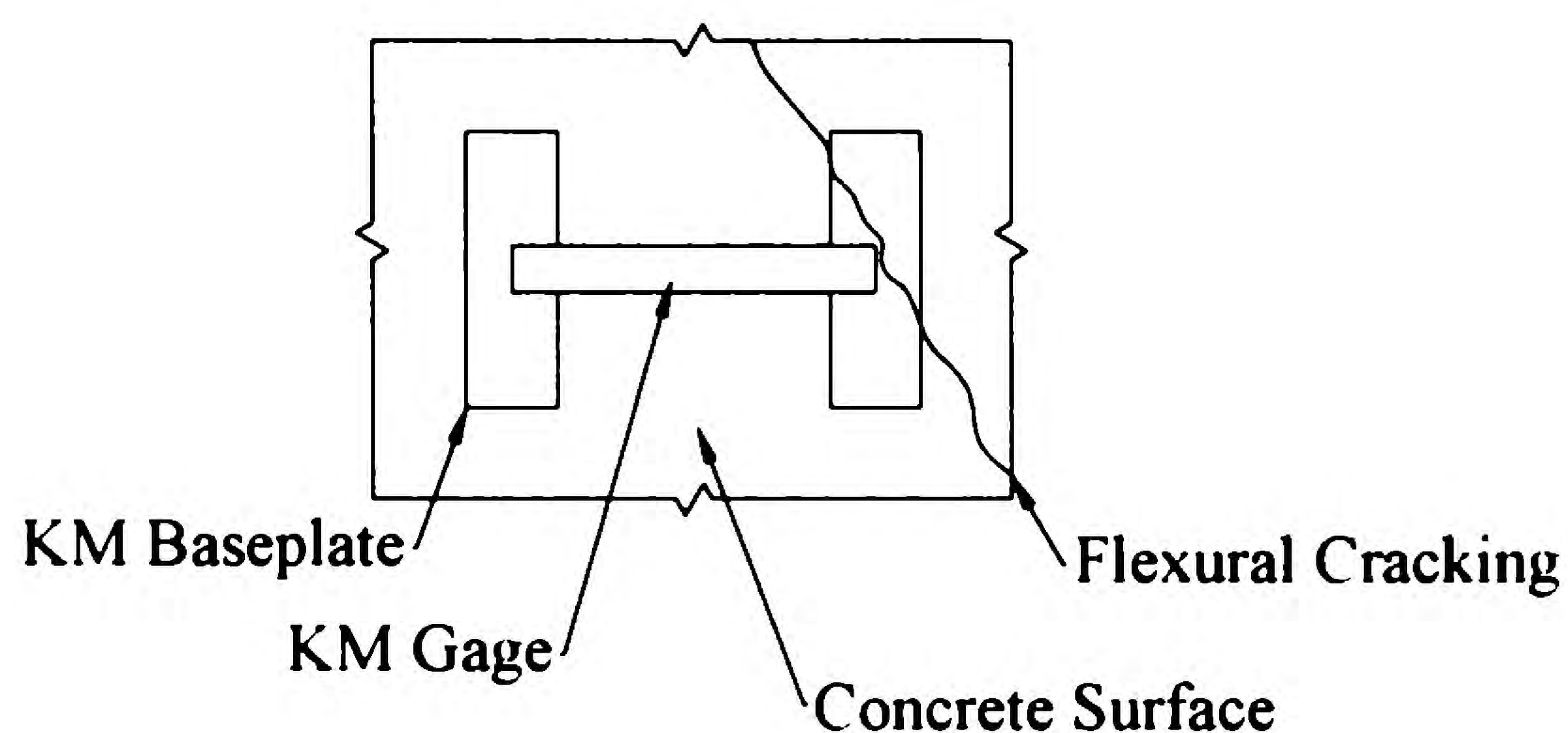
Figure 5-10. KM Gage Detail.
