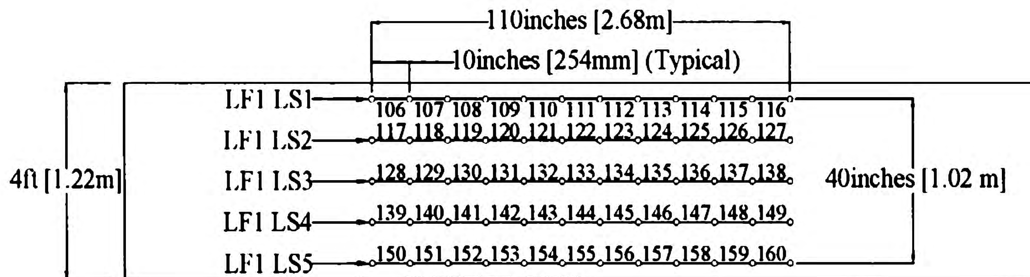
(d) Longitudinal Strain Locations on Large Face 1
