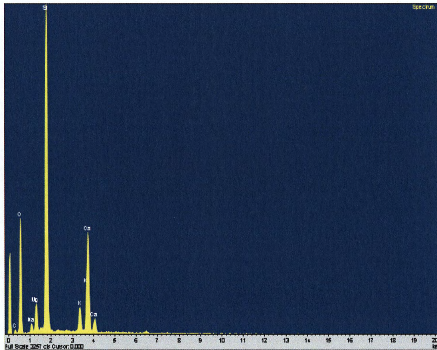
SEM/EDS spectra of ASR gel exudation
