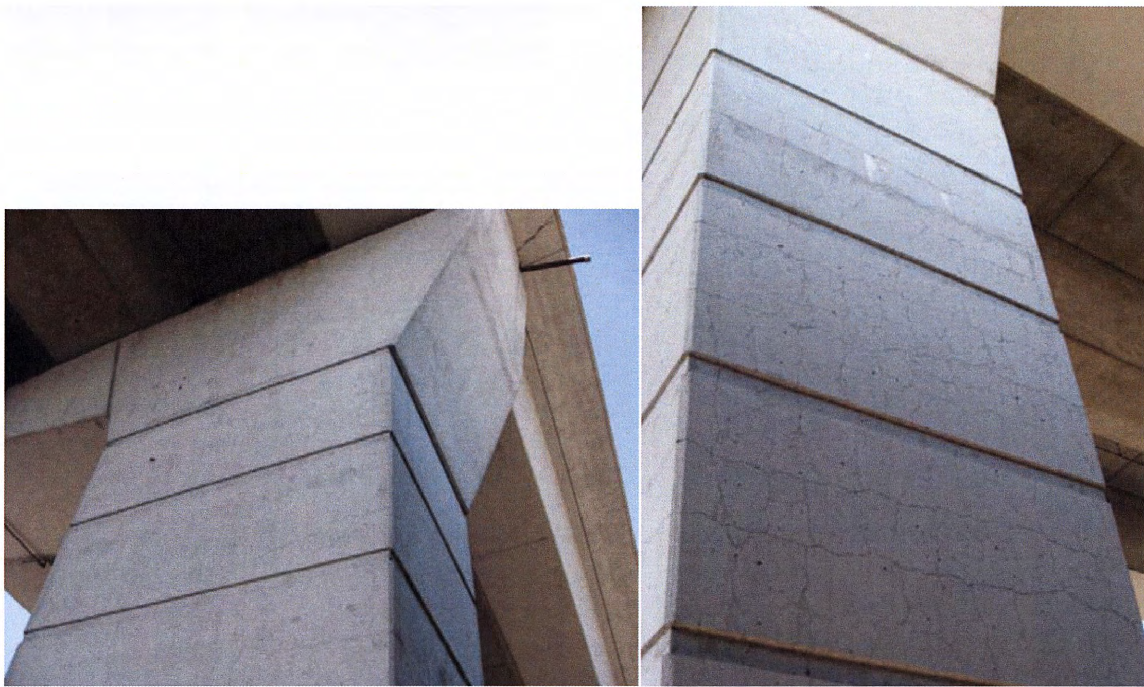
(a) Elevation View and Typical Cracking on Tension Face (Houston, TX)
