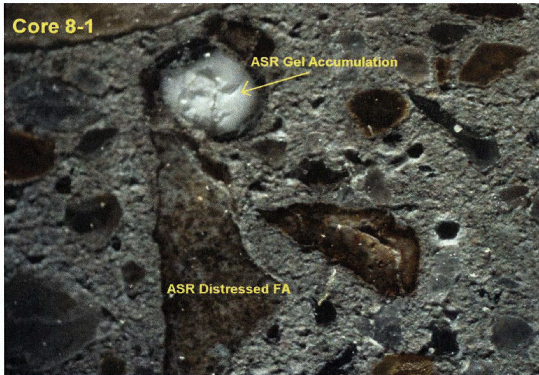
Image illustrating ASR gel accumulation in air void adjacent to reactive particle
