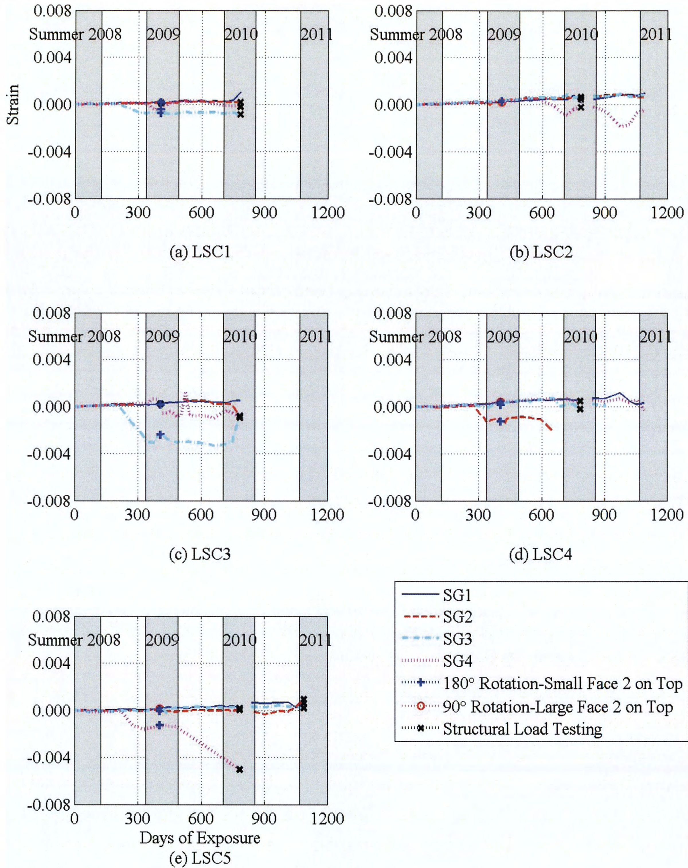
Figure 3-20. Internal Strain Gages (SG1-SG4) along Large Face 1 Tension Steel of the Splice Region.
