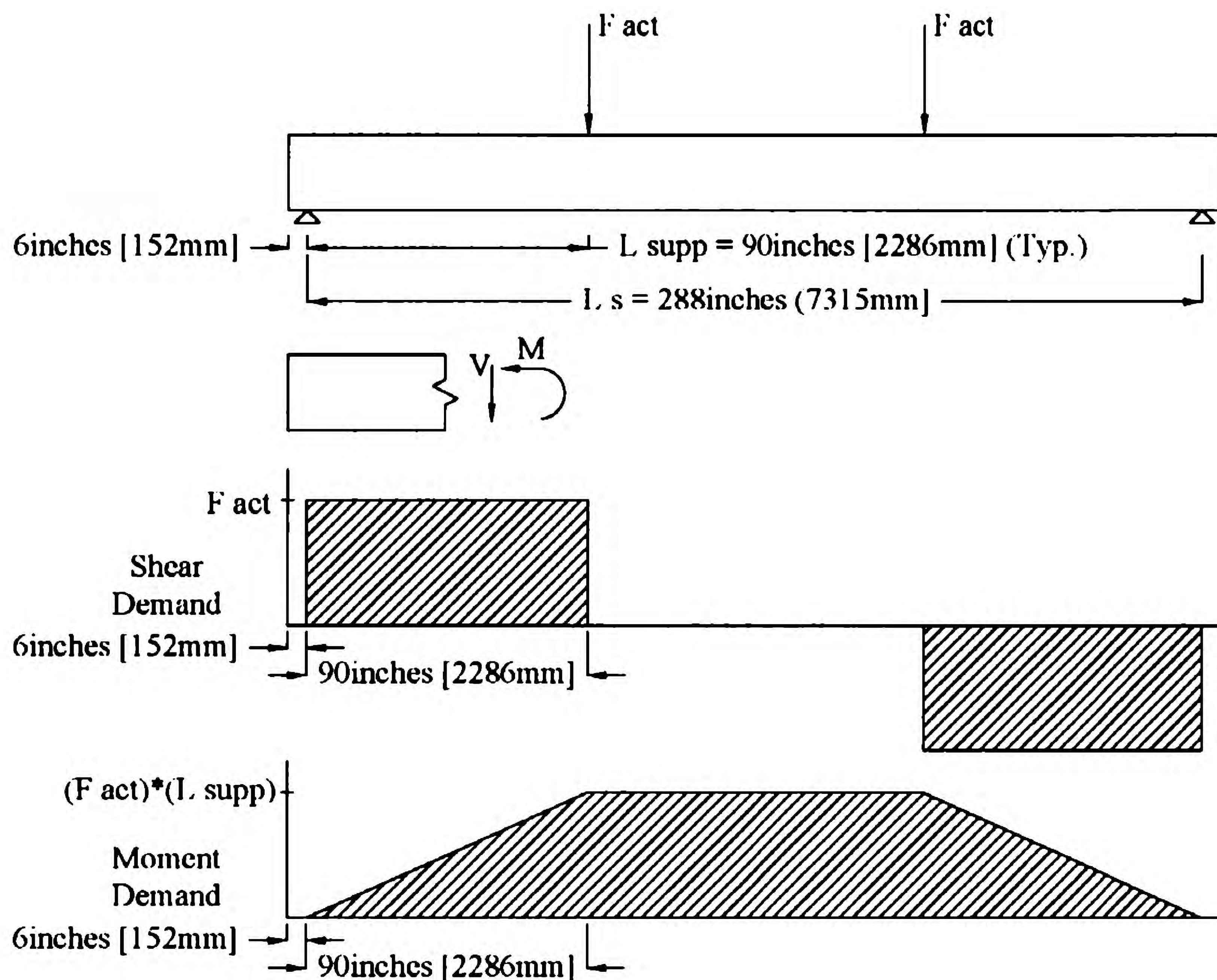
Figure 4-11. Four-Point Test Shear and Moment Diagram.
