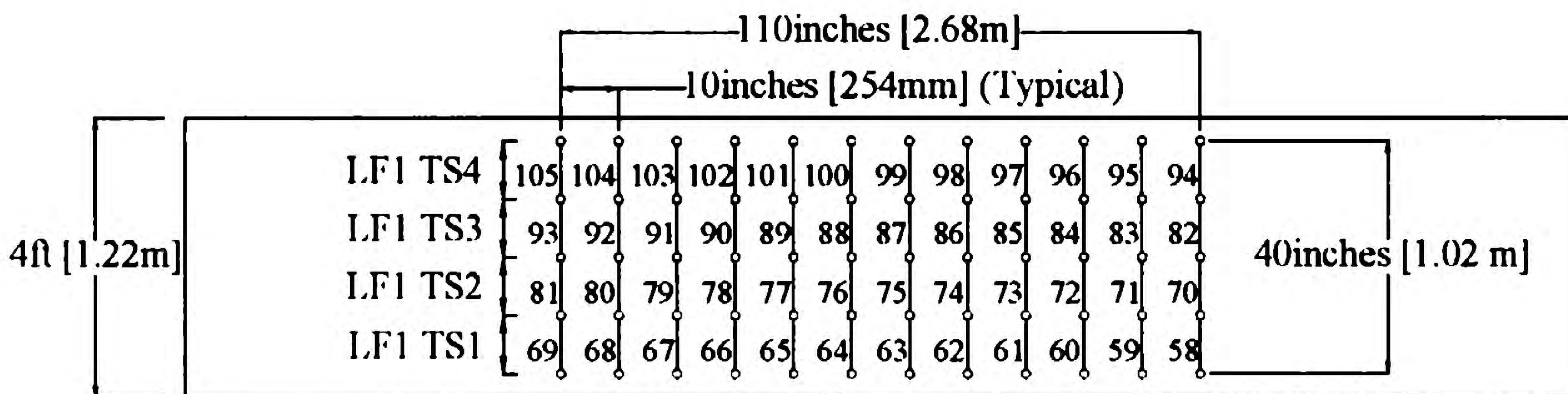
(c) Transverse Strain Locations on Large Face 1
