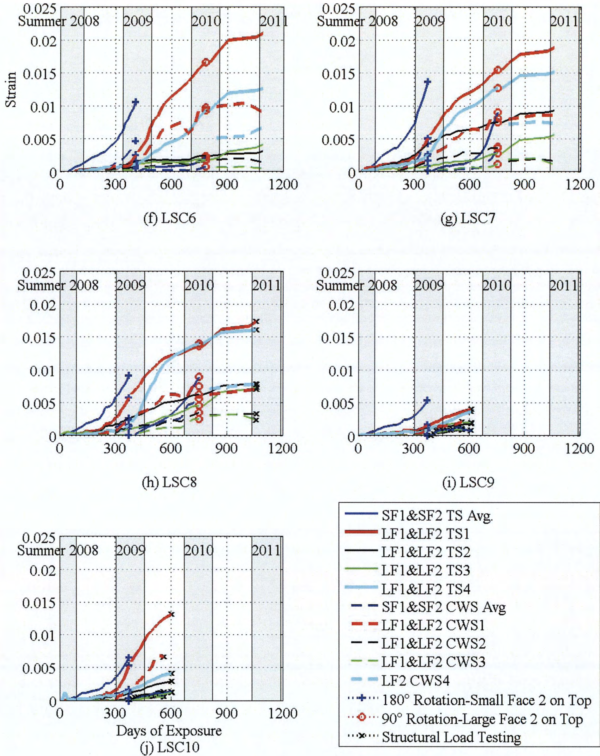
Figure 3-18. Transverse Surface Strains from DEMECs and Crack Width Measurements on All Faces. (Continued)
