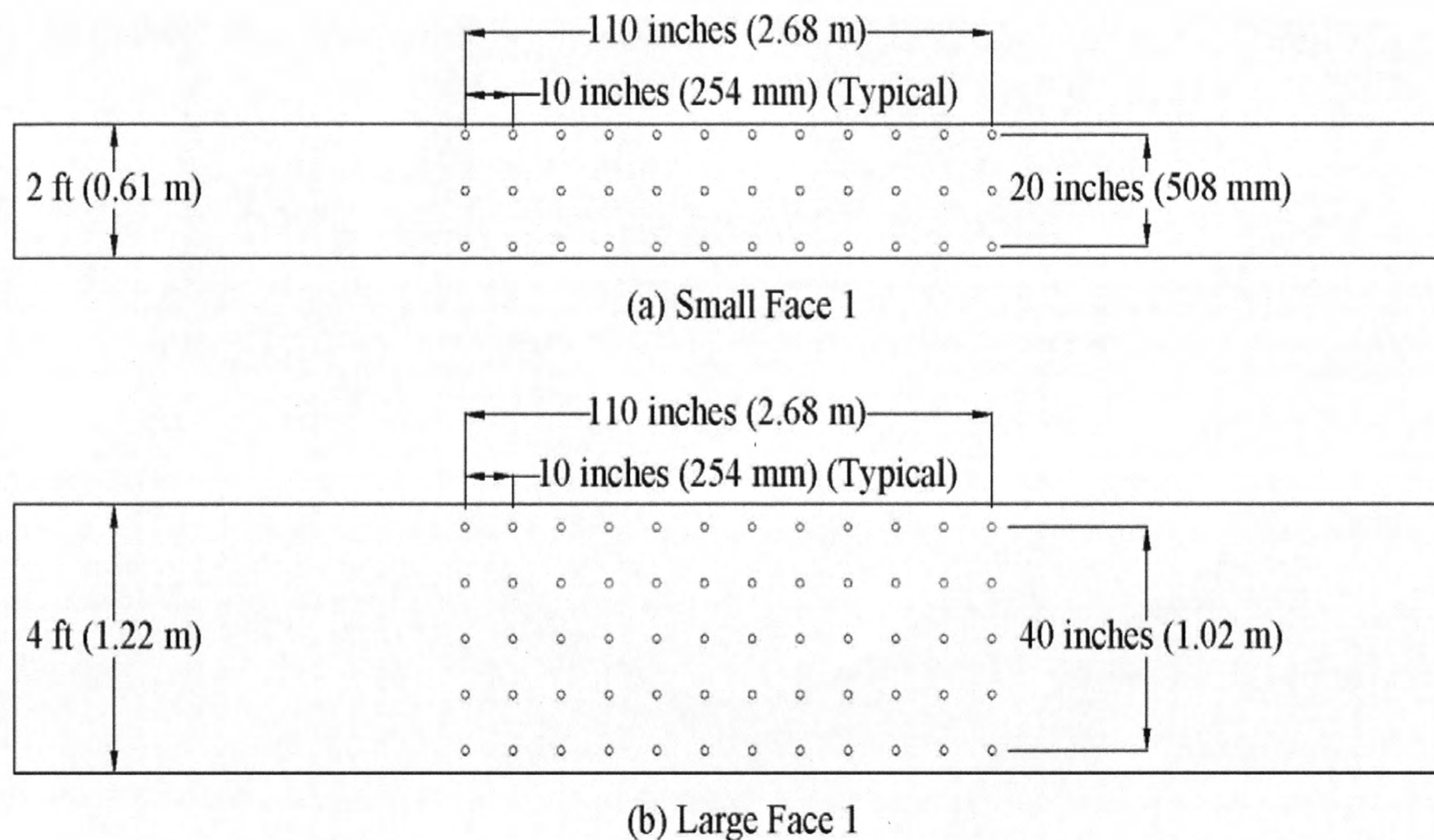
Figure 2-25. DEMEC Layout in the Splice Region.
