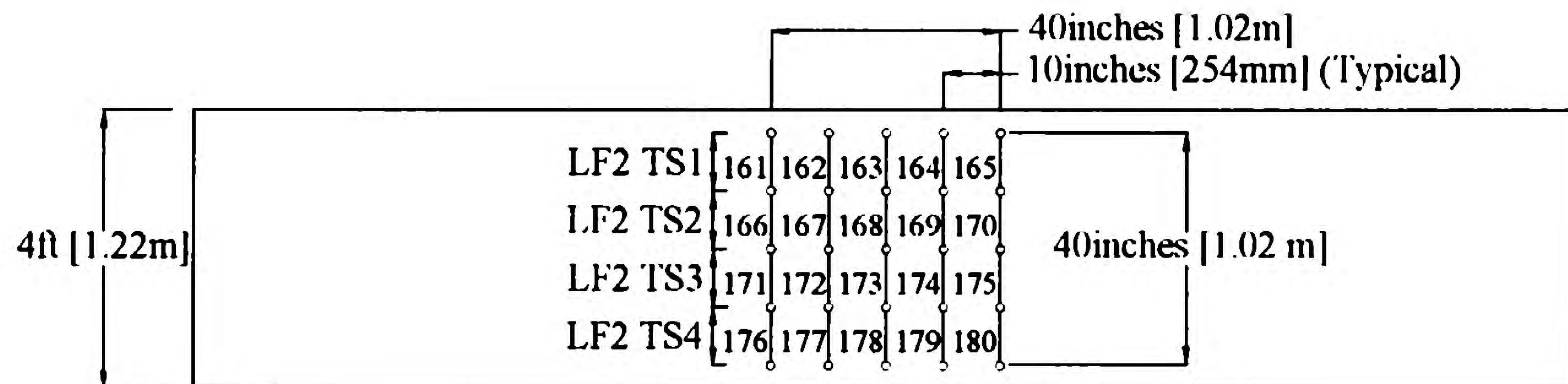
(a) Transverse Strain Locations on Large Face 2
