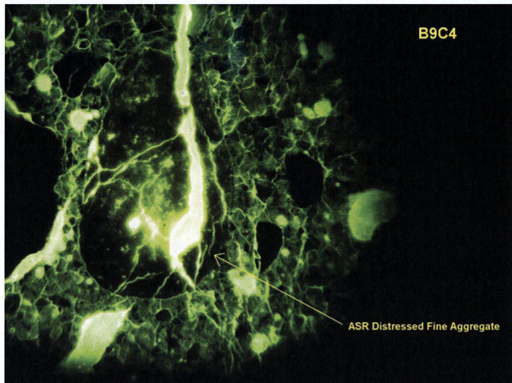
Fluorescent image illustrating numerous ASR distress cracking
