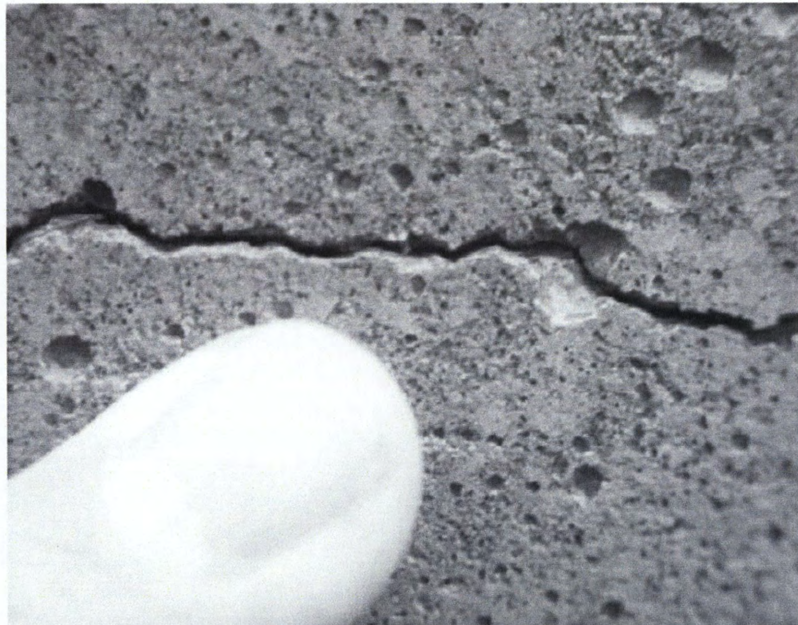
Figure 3-16. Longitudinal Crack Width.
