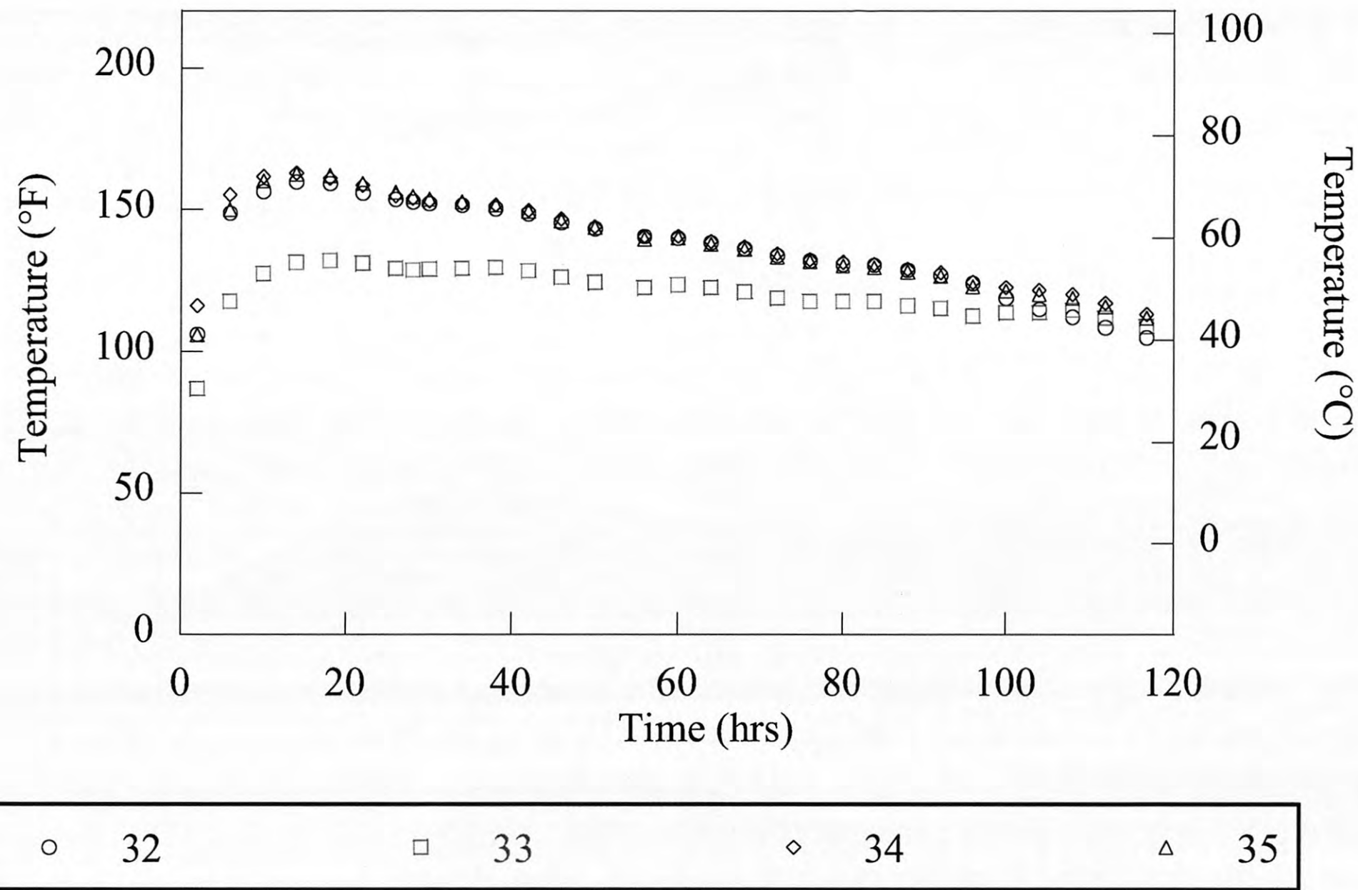
Figure 2-17. Typical Temperature History at End-Span Section.
