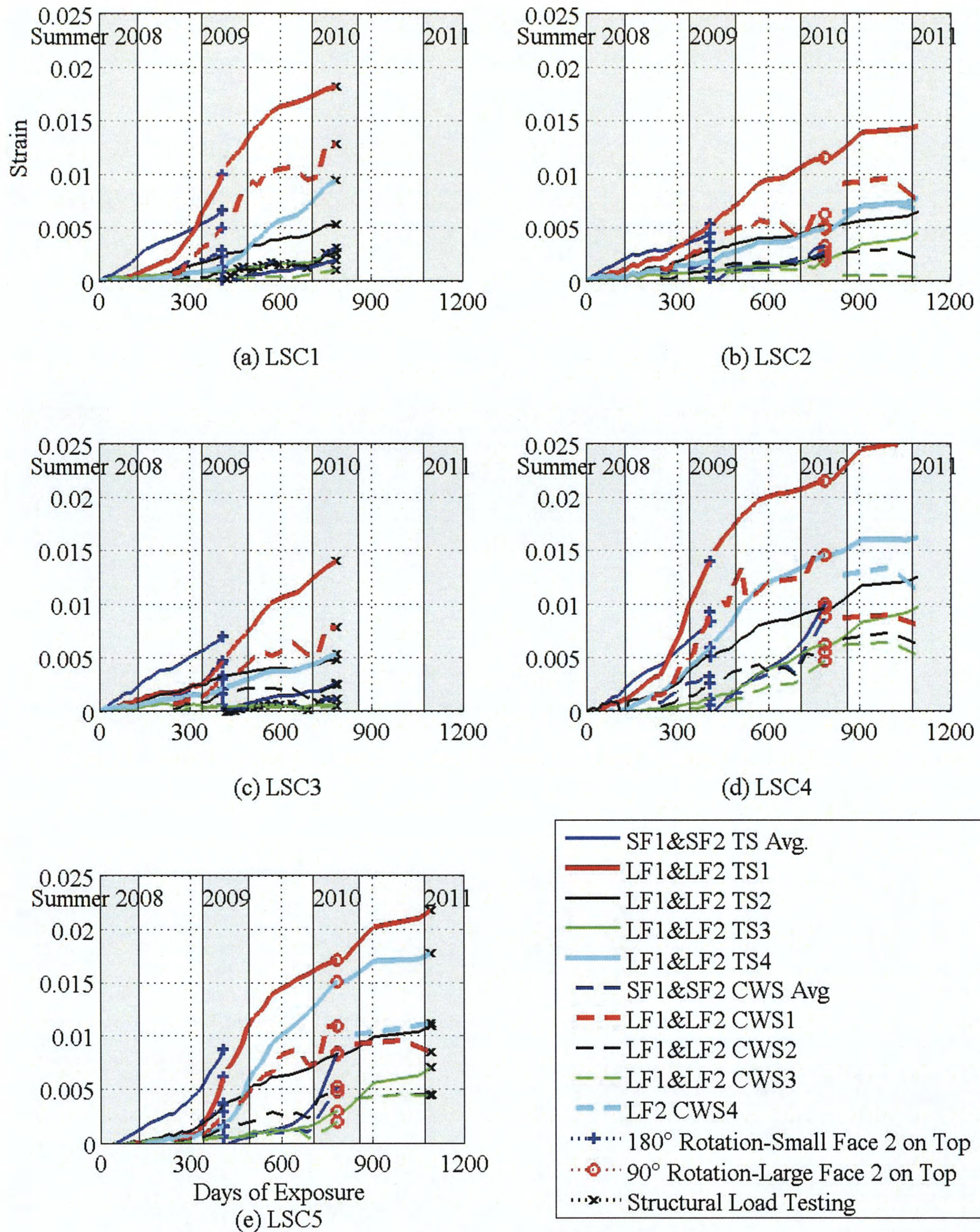
Figure 3-18. Transverse Surface Strains from DEMECs and Crack Width Measurements on All Faces.
