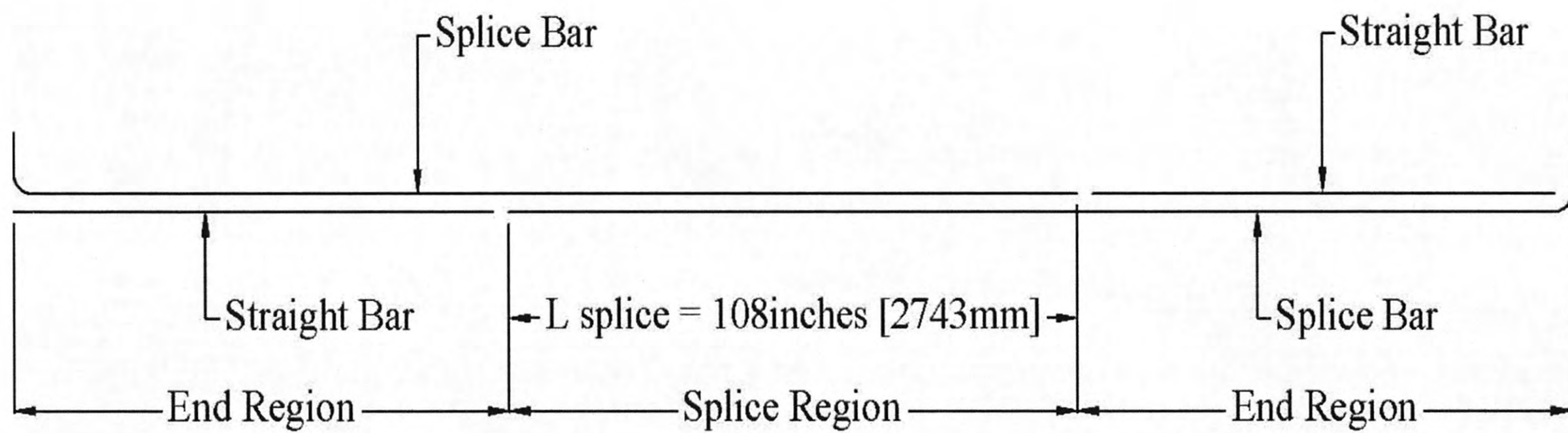
Figure 4-5. Longitudinal Section of Tension Reinforcing Steel.
