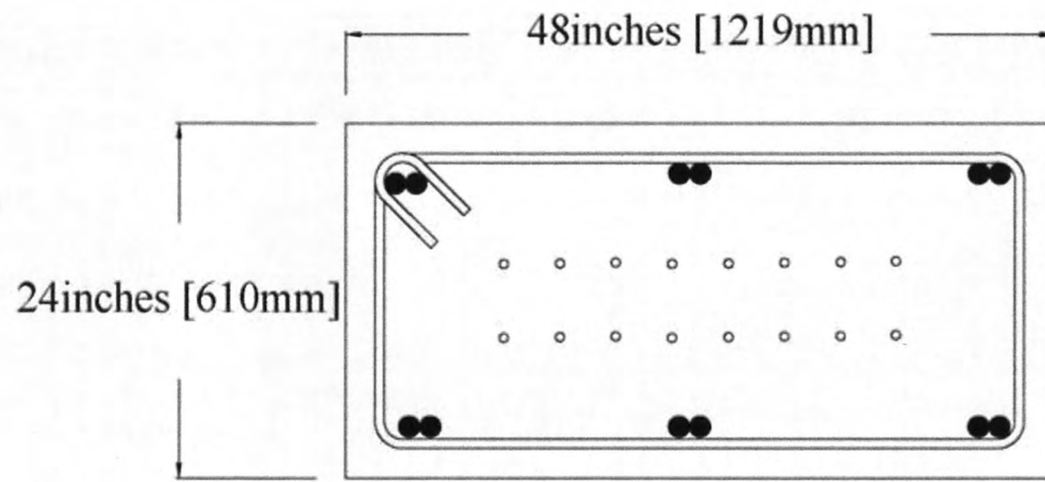
Section A-A Splice Region
