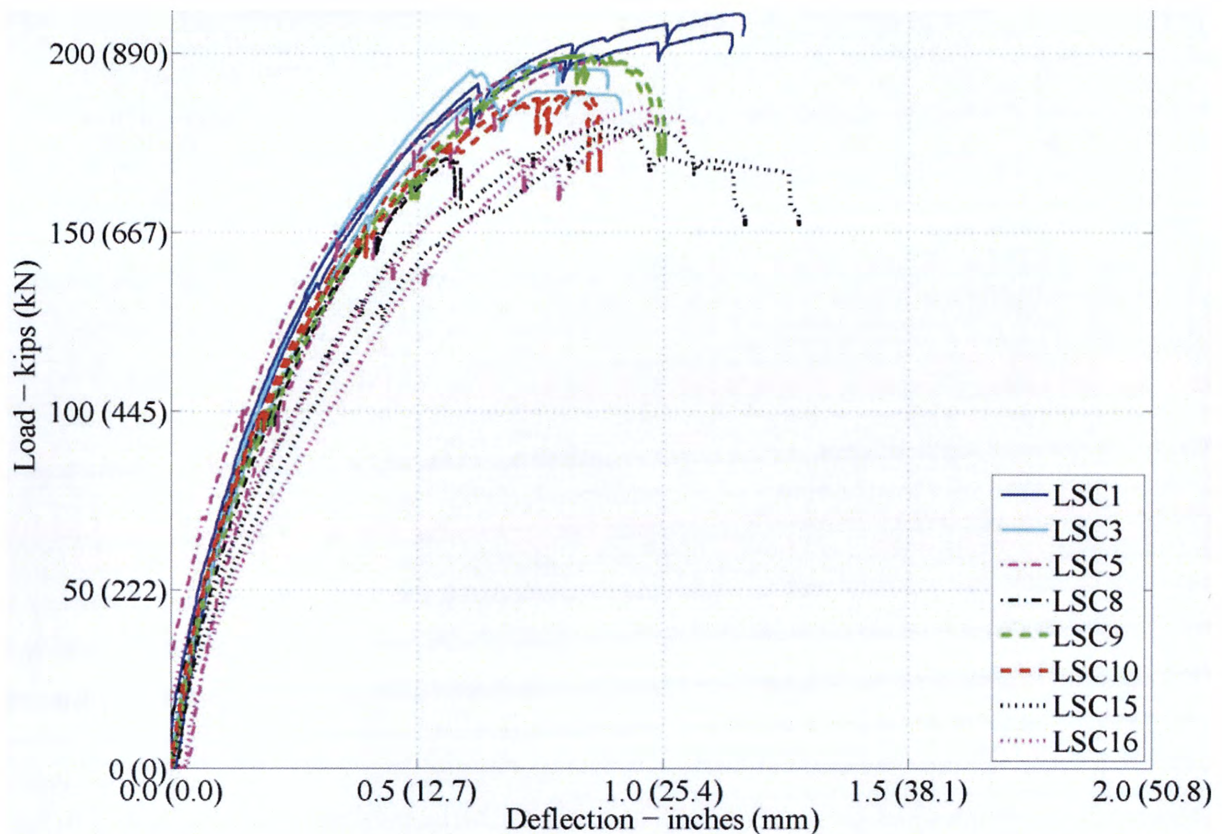
Figure 5-36. Experimental Load vs. Deflection during the Three-Point Test: All Tested Specimens at the Actuator Load Point.
