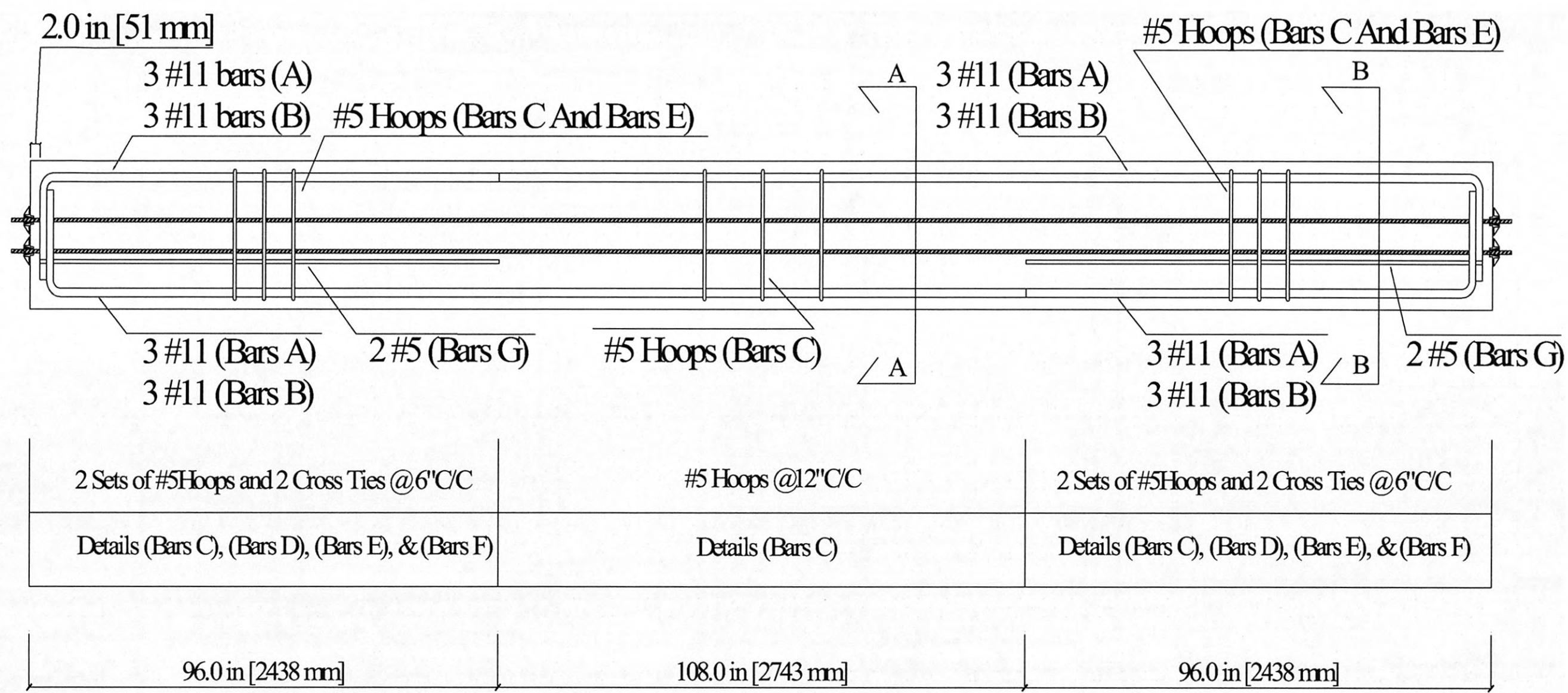
Figure 2-3. Reinforcement Layout.
