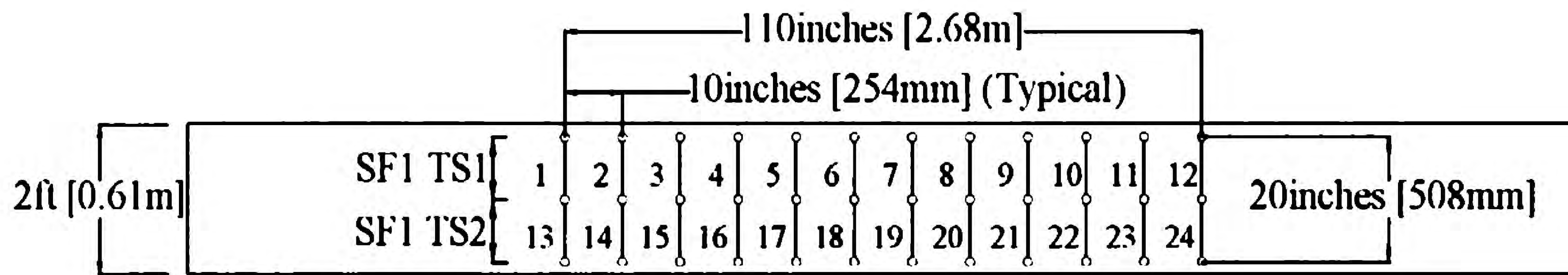
(a) Transverse Strain Locations on Small Face 1
