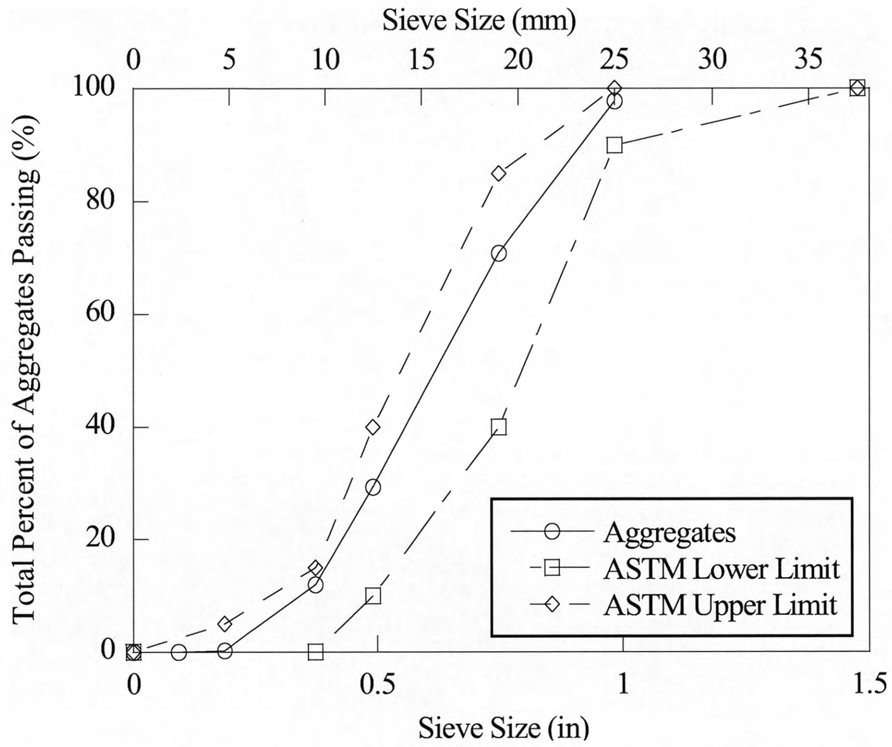
Figure 2-9. Gradation of the Coarse Aggregates.
