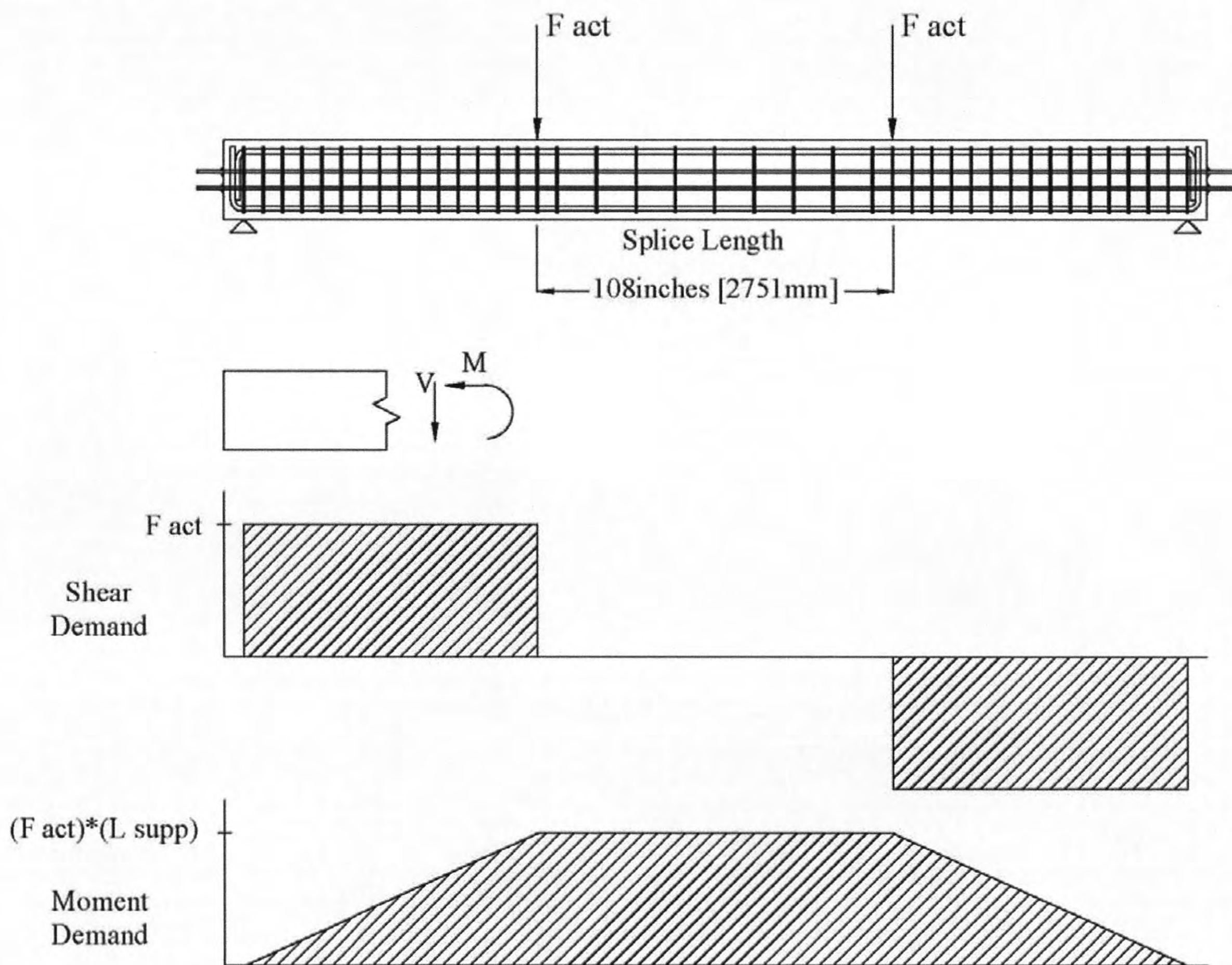
Figure 2-5. Four-Point Load Test.
