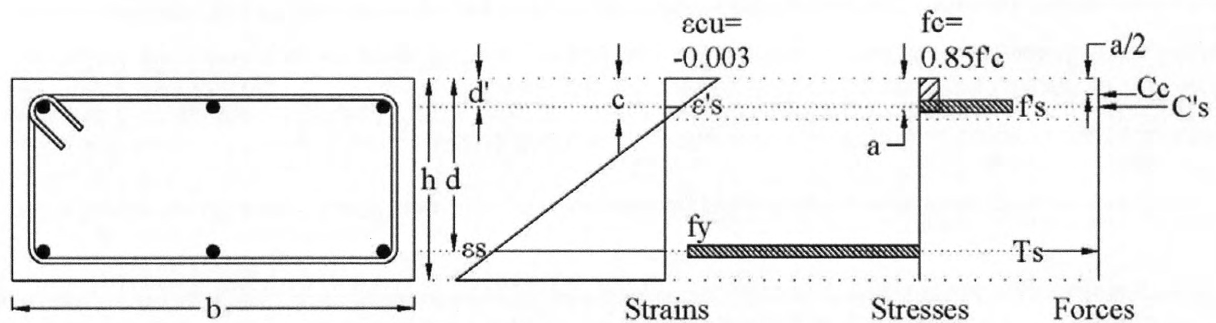
Ultimate - Crushing of Concrete in Compression
