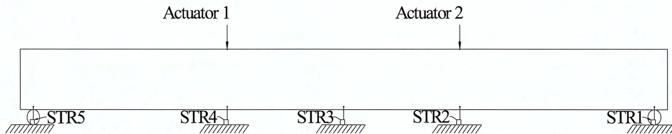
Figure 5-6. STR Locations for the Four-Point Test.
