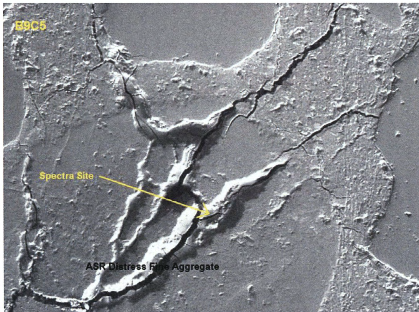
BSE image illustrating highly distress aggregate
