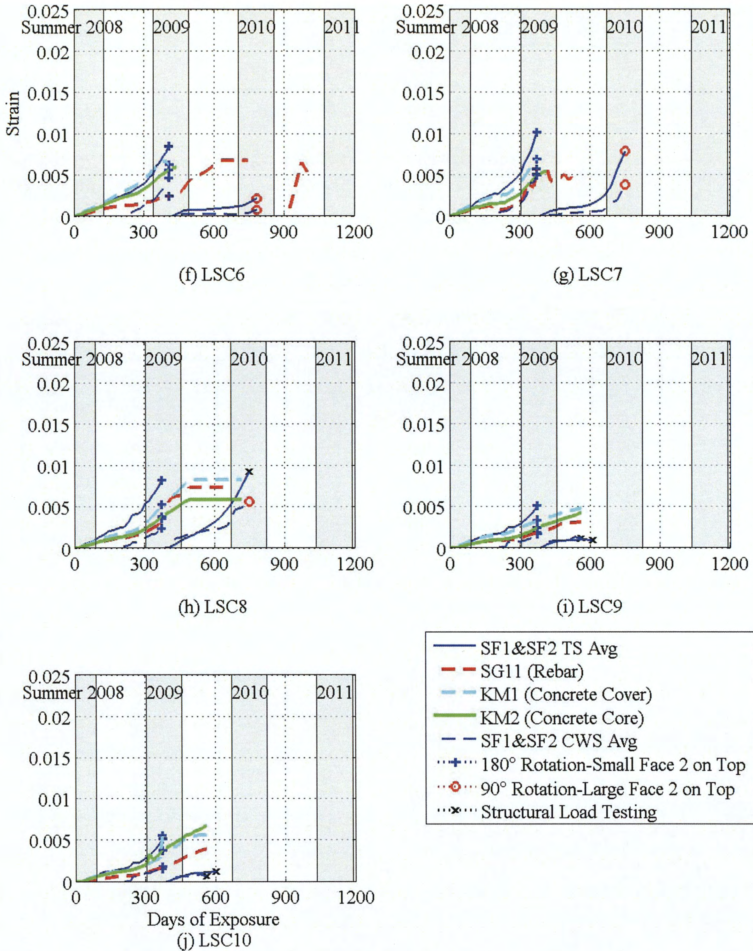
Figure 3-23. Internal and External Strain Measurements on and near the LSC Specimens' Small Face 1 and Small Face 2. (Continued)
