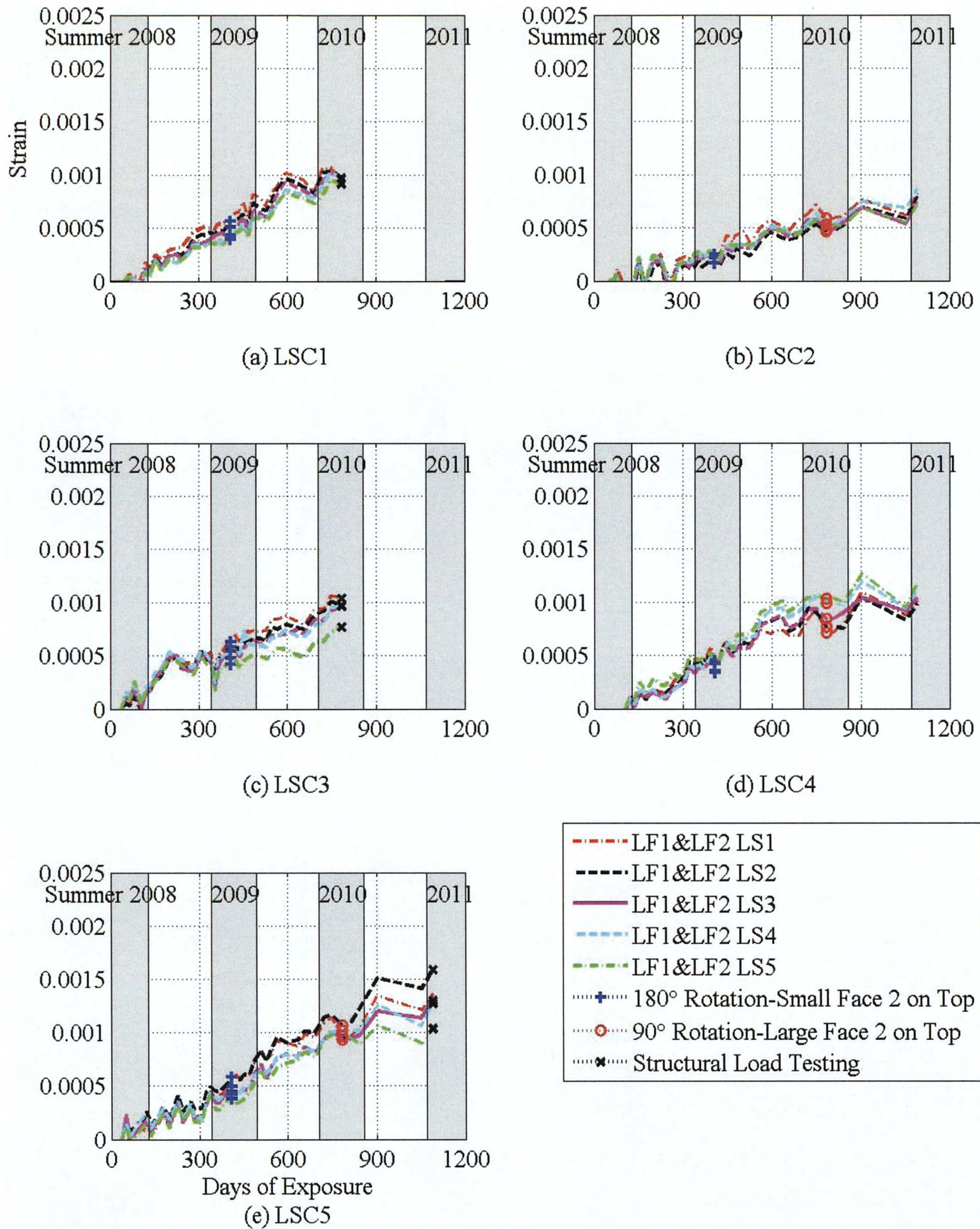
Figure 3-14. Longitudinal Surface Strains on the LSC Specimens' Large Face 1 and Large Face 2.
