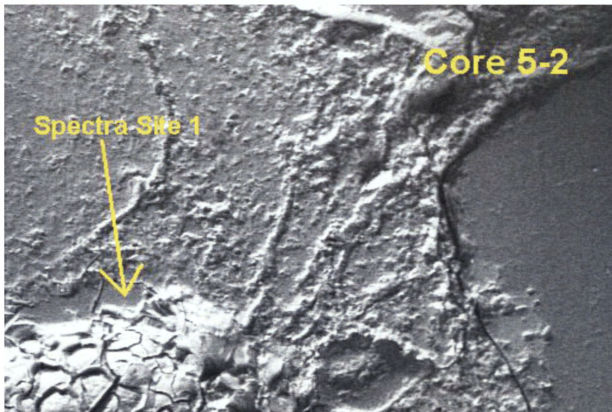
SEM/BS image illustrating accumulation of ASR gel in an air void
