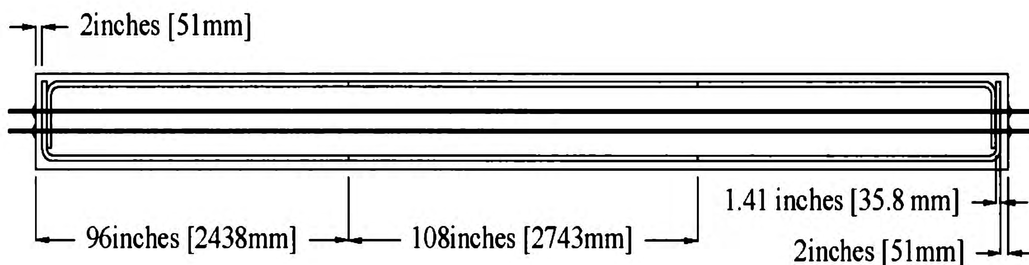
Figure 4-2. Reinforcement Elevation View.
