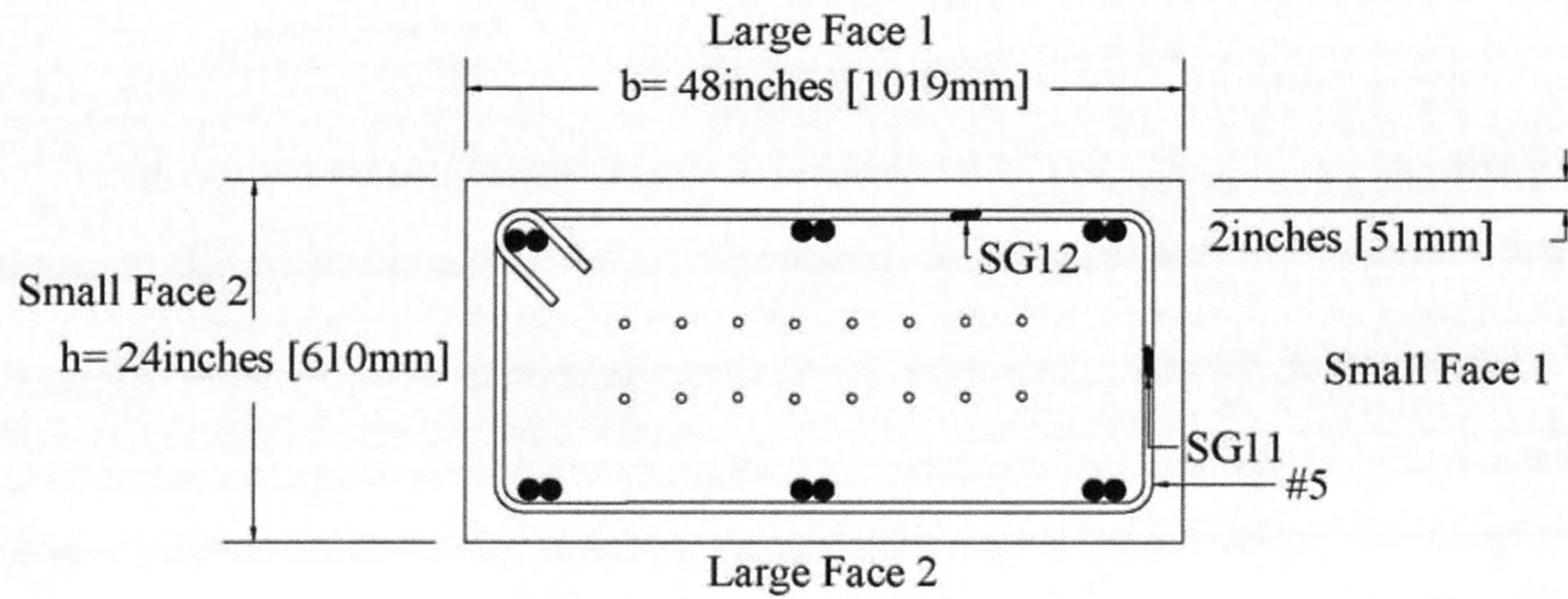
Cross Section with SG11-SG12
