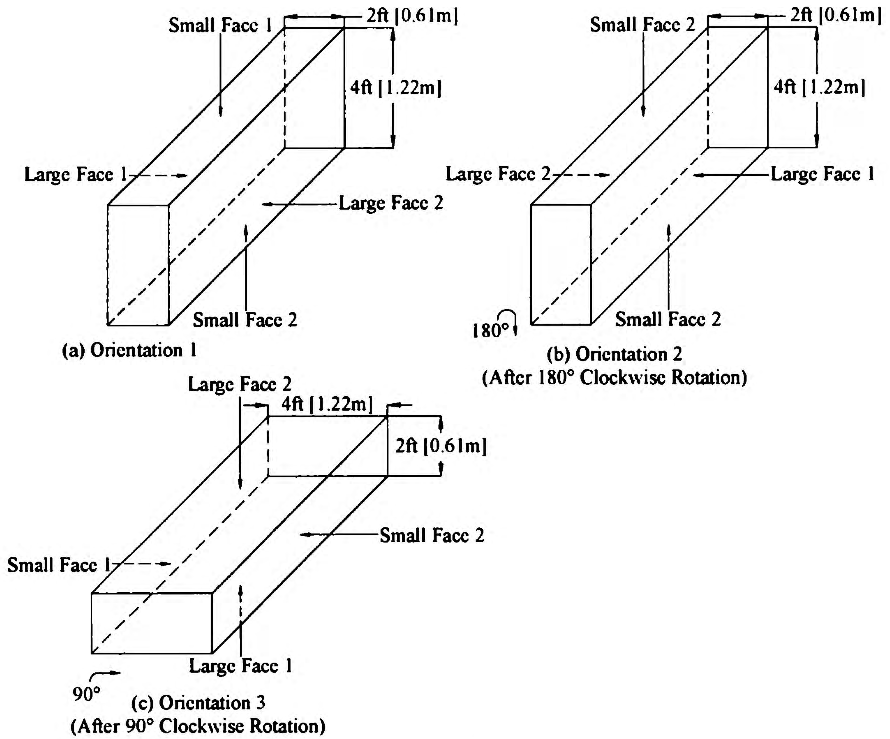
Figure 3-5. Orientations of the LSC Specimens.
