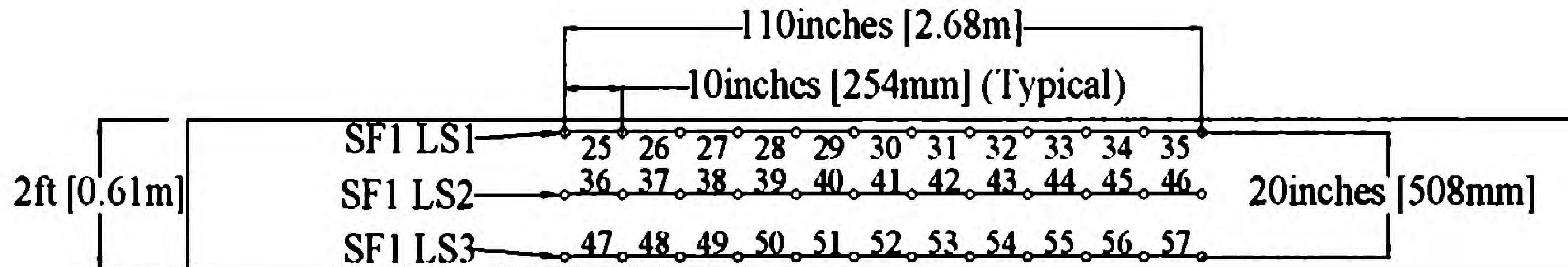
(b) Longitudinal Strain Locations on Small Face 1
