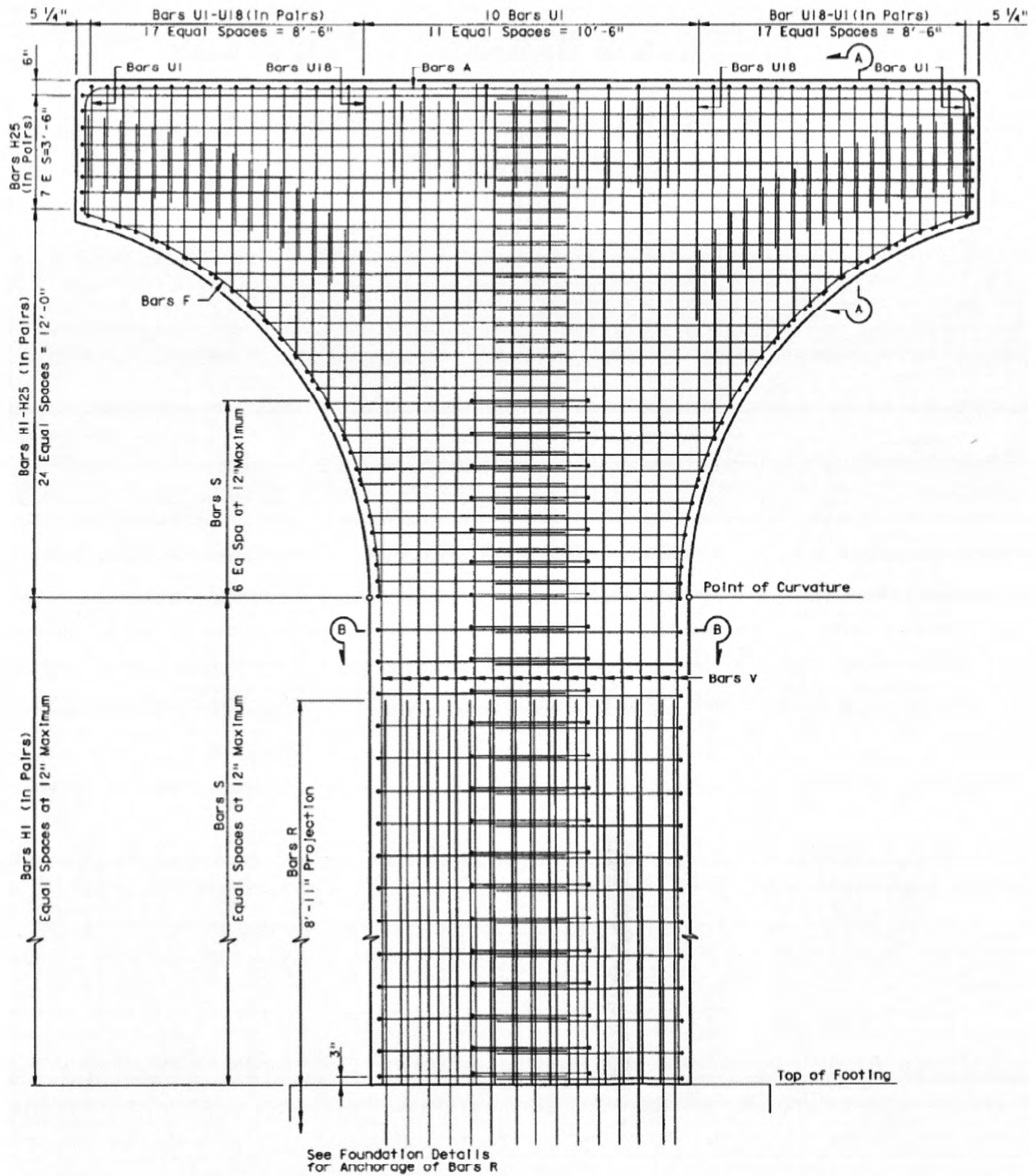
Figure 2-1. Sample TxDOT Column Reinforcement Detail.
