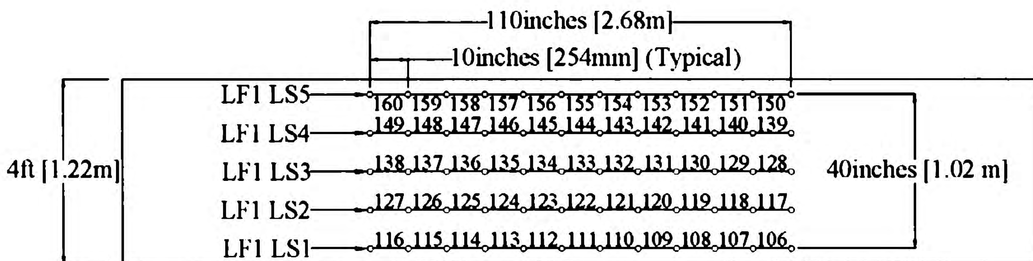
(d) Longitudinal Strain Locations on Large Face 1
