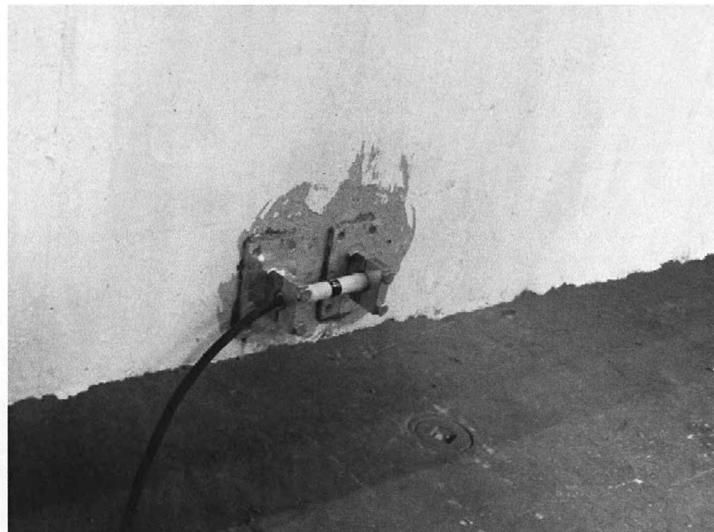
Figure 5-8. KM Gage Installation prior to Testing.
