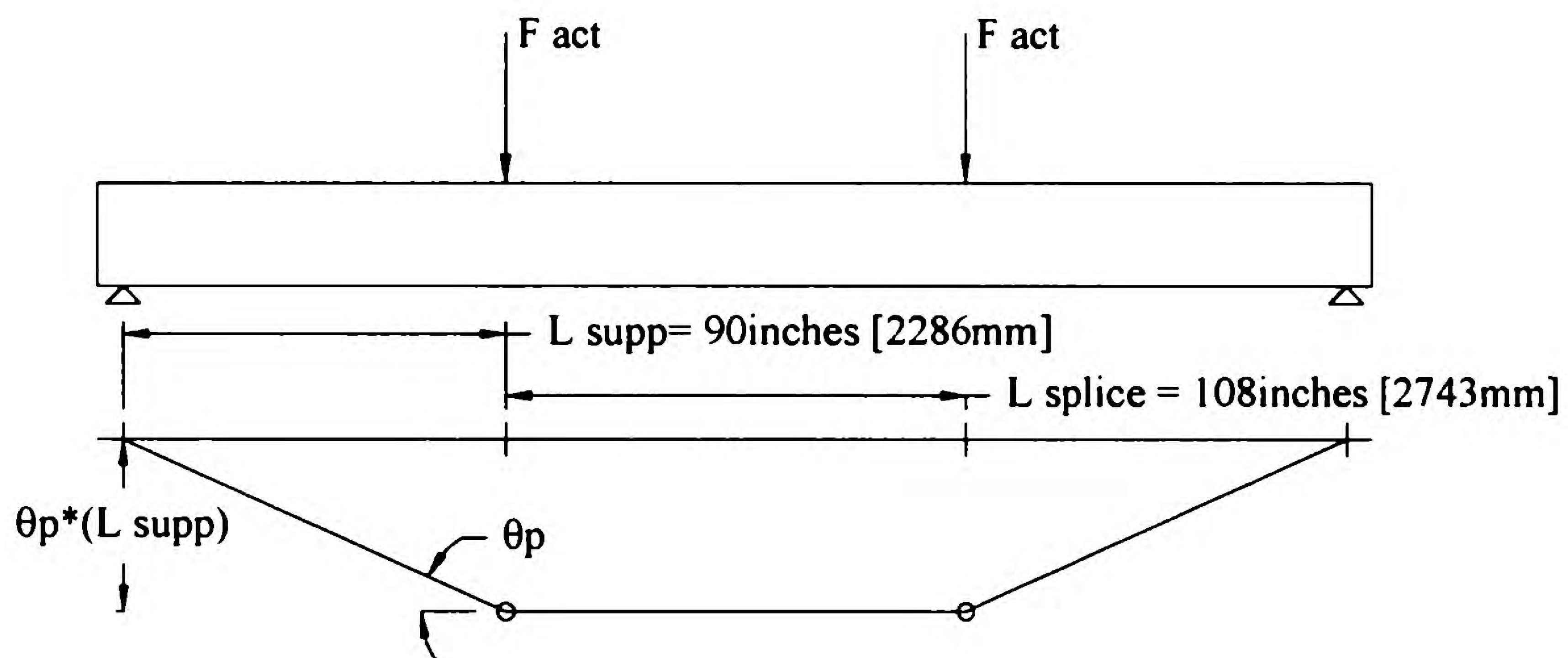
Figure 4-14. Plastic Hinge Rotation for Four-Point Setup.
