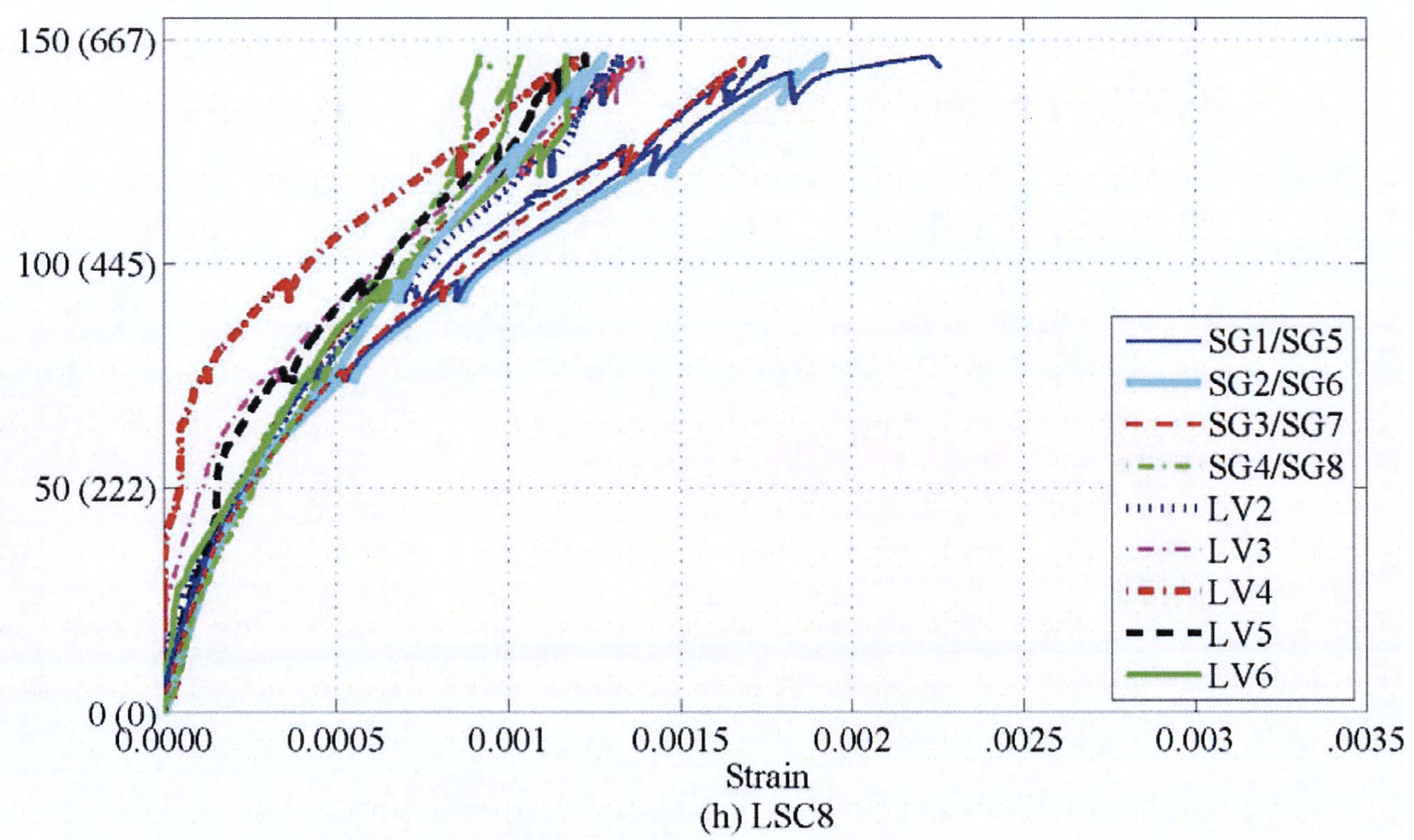
Figure 5-29. Experimental Load vs. Strain during the Four-Point Test: Internal and External Strain Comparison across Splice Length. (Continued)
