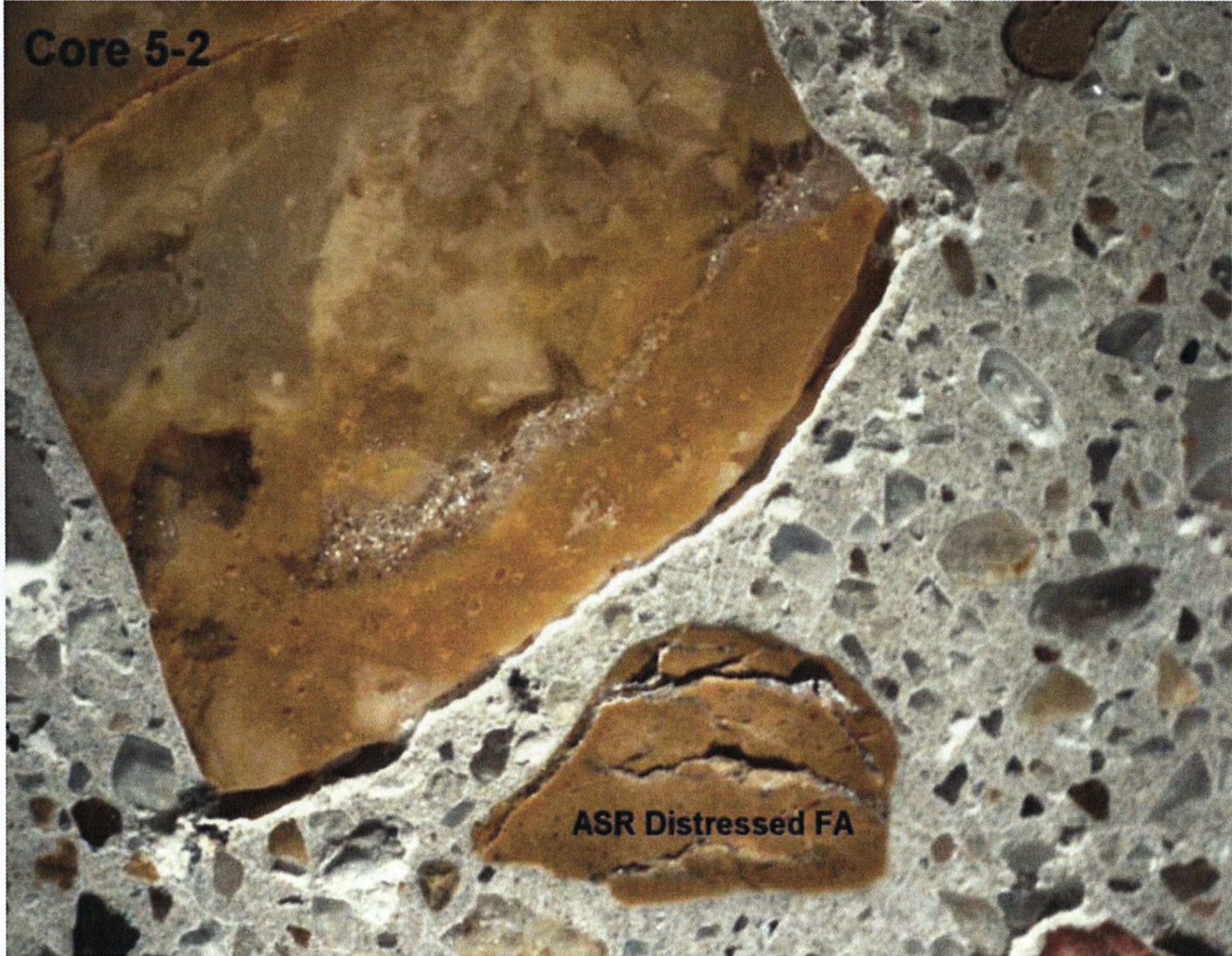
Image illustrating ASR distress in intermediate size aggregate
