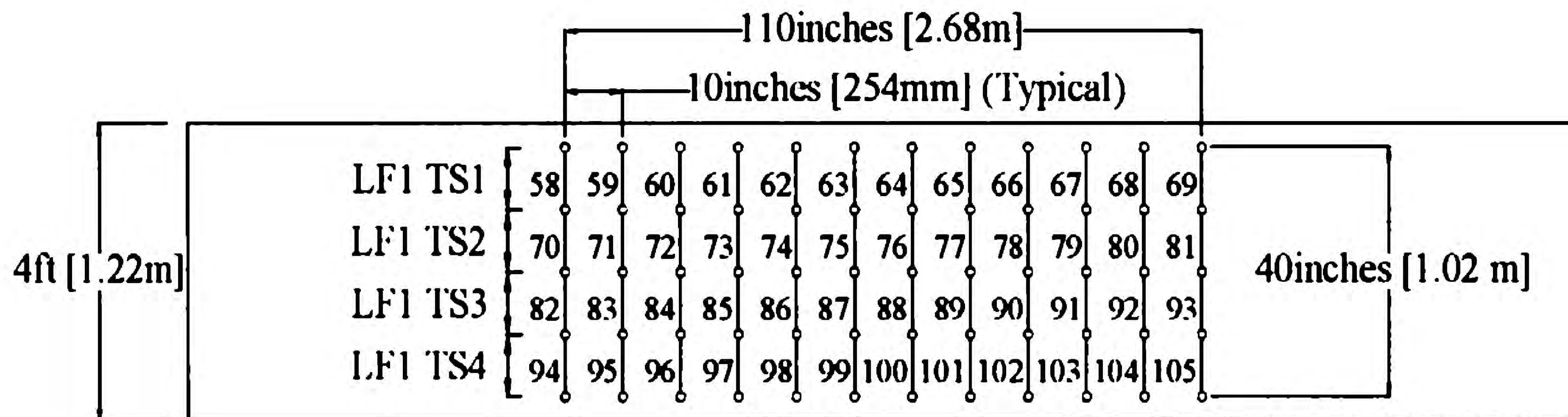
(c) Transverse Strain Locations on Large Face 1
