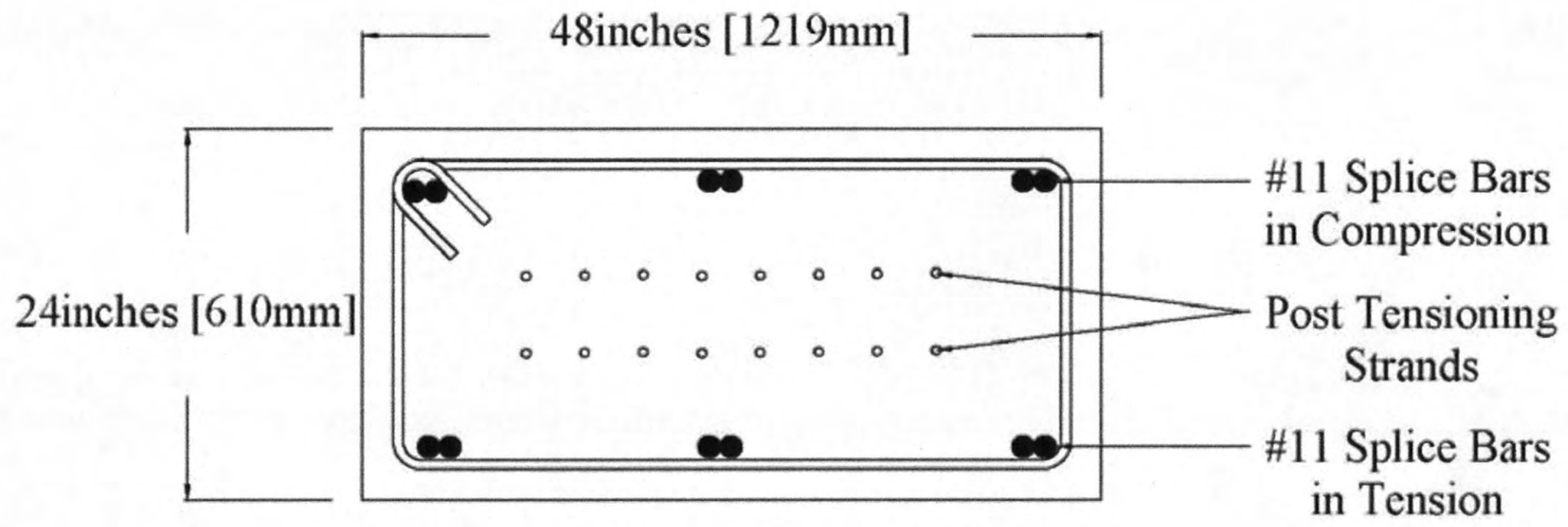
Figure 4-3. Cross Section at Splice Region.
