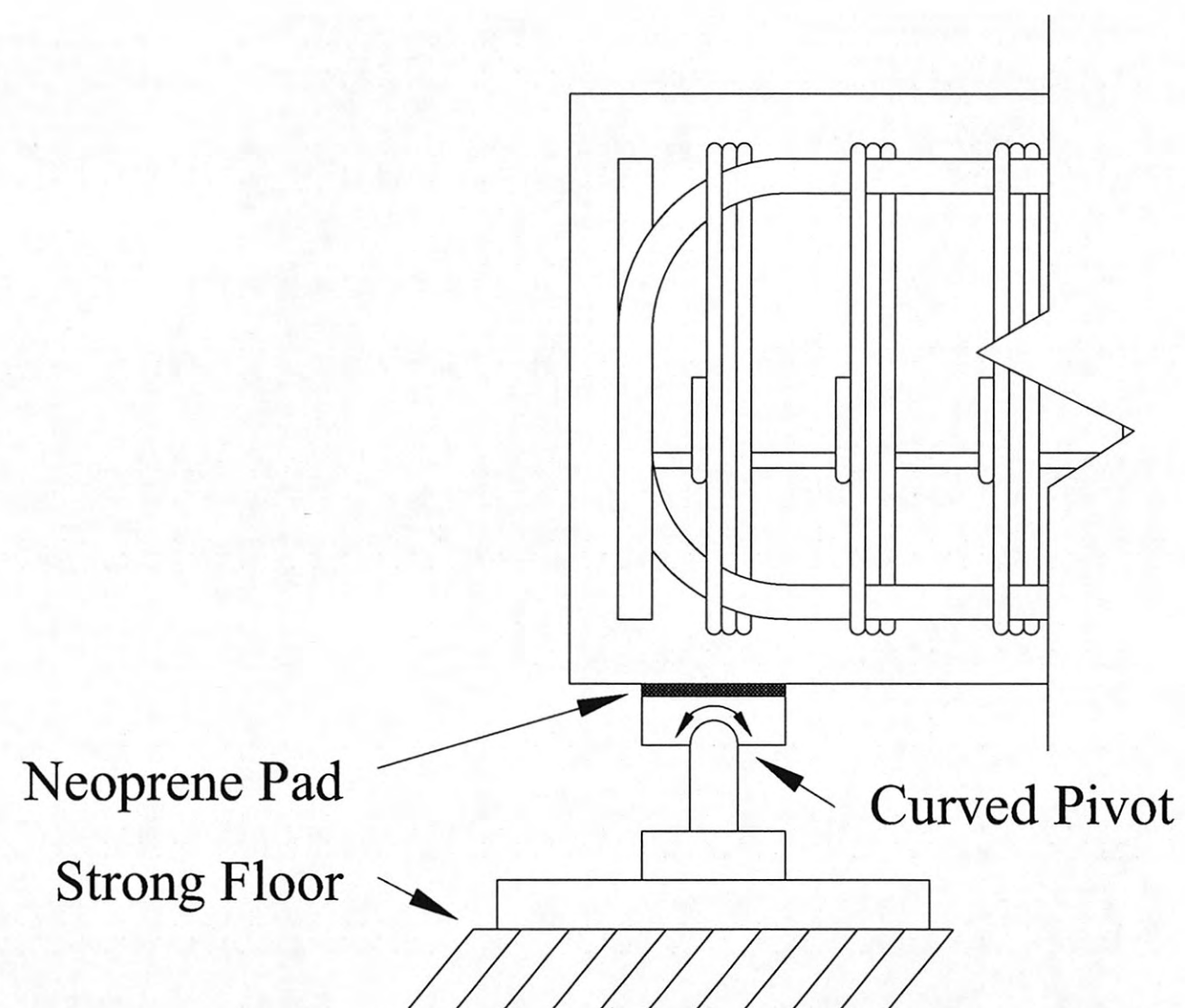
Figure 5-2. "Pinned" Support Setup.
