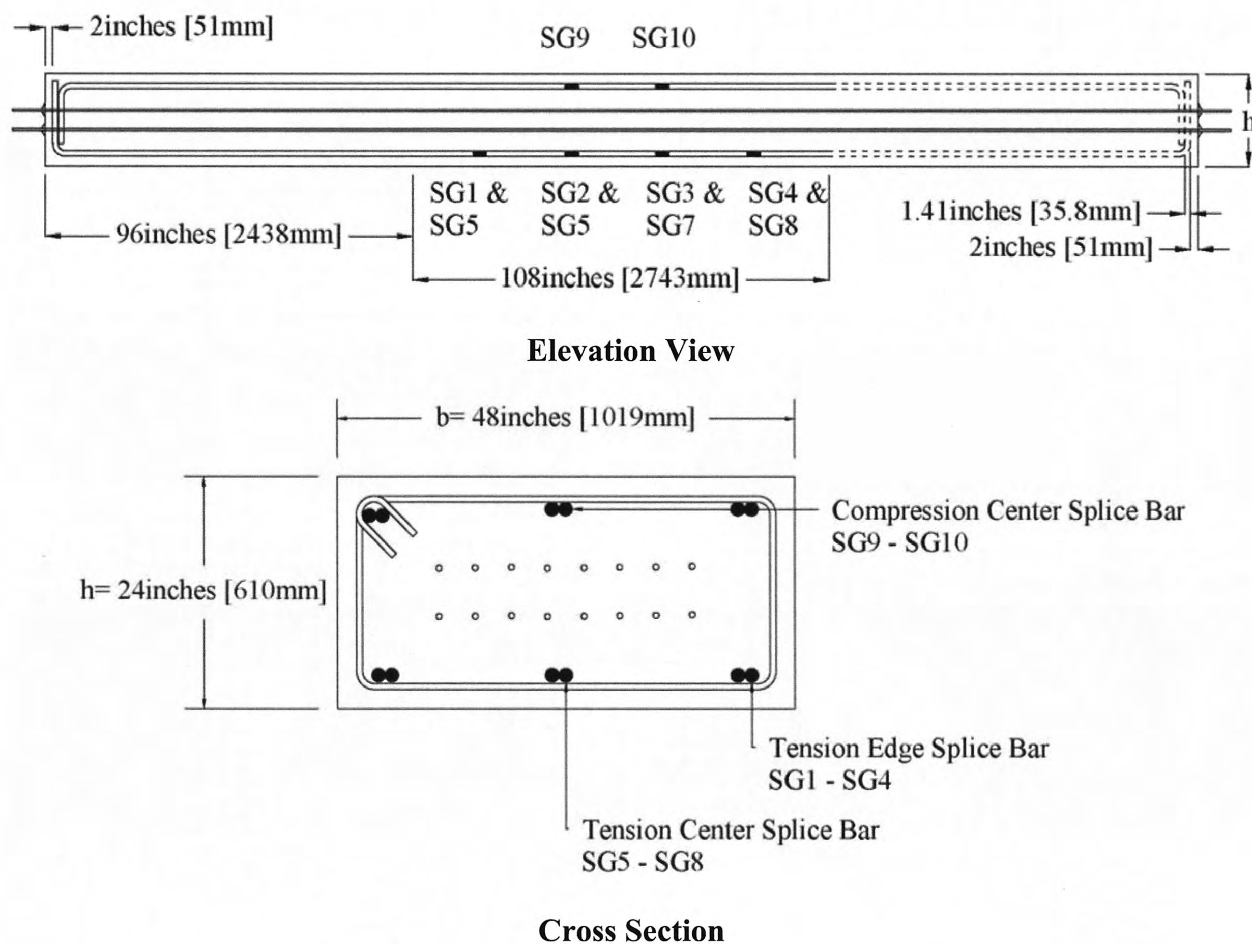
Figure 2-27. Internal Strain Gage Locations on Longitudinal Reinforcement.
