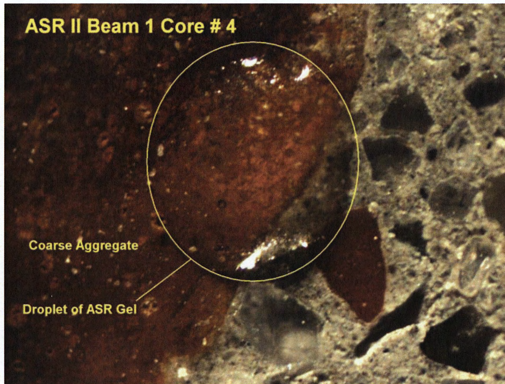
Small droplet of ASR gel which oozed out of aggregate after cutting and polishing
