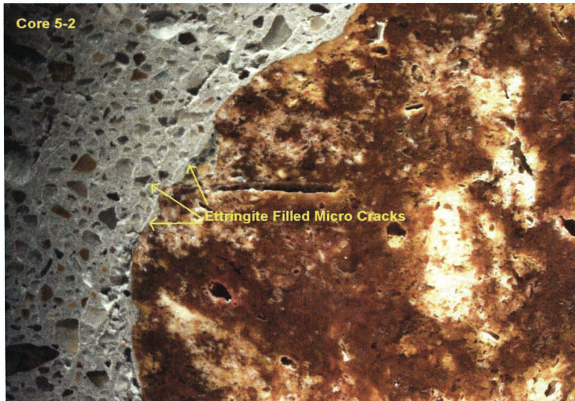
Image illustrating fine network of ettringite-filled micro cracks
