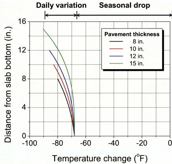
(c) Thermal loading
