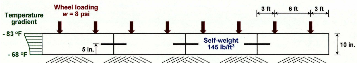
Figure 4.11: Combined traffic loading, self-weight, and temperature gradient
