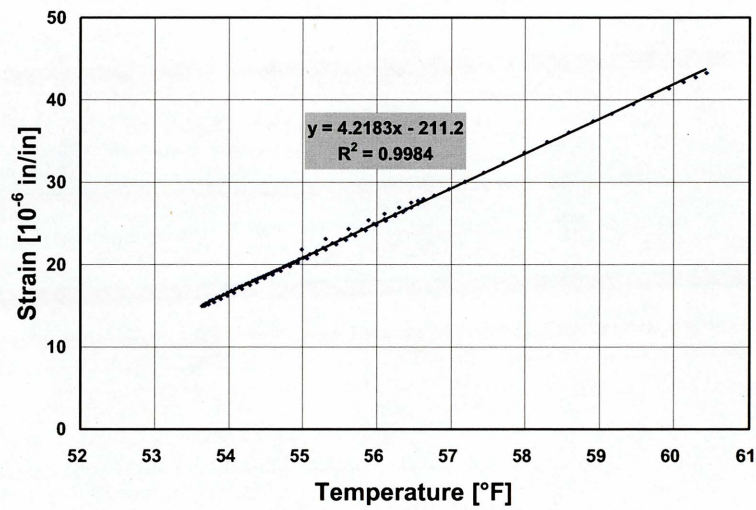
Figure 2.13: Measured coefficient of thermal expansion of concrete
