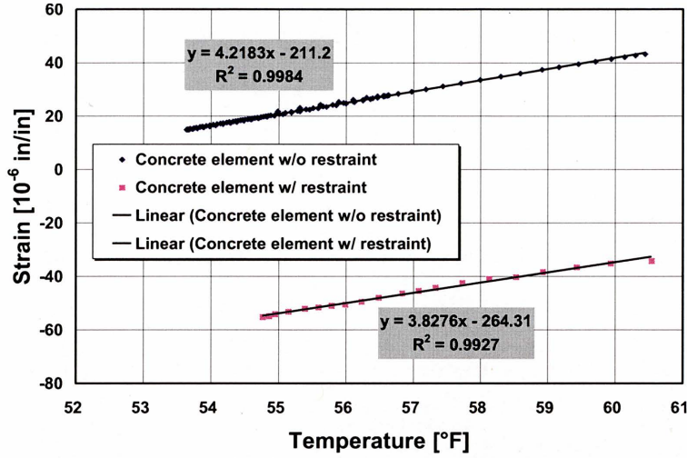
Figure 2.8: Concrete strain vs. concrete temperature
