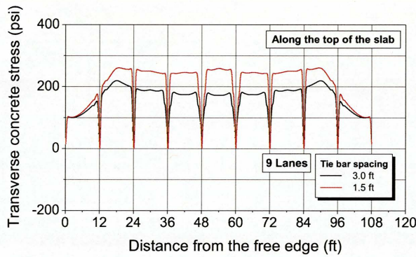
(c) Concrete stress along the top of the slab in nine-lane pavement
