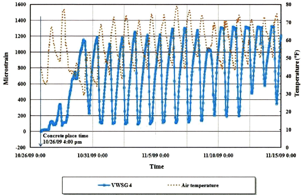
Figure 2.21: Strain of the gage at the longitudinal construction joint
