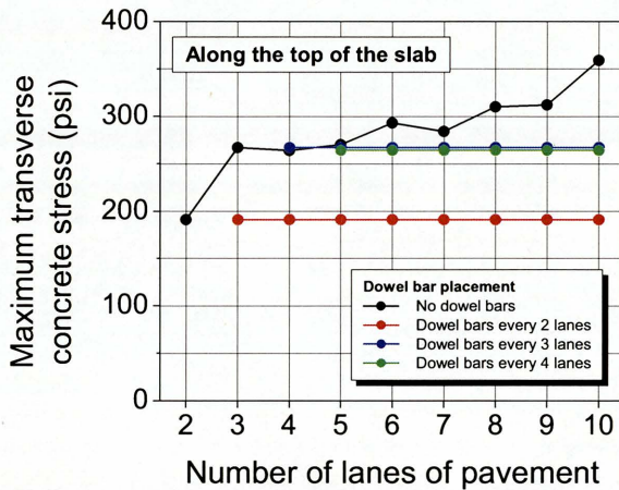
(c) Maximum concrete stress at the top of the slab
