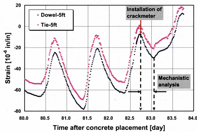
(b) At 5 ft from the LCJ
