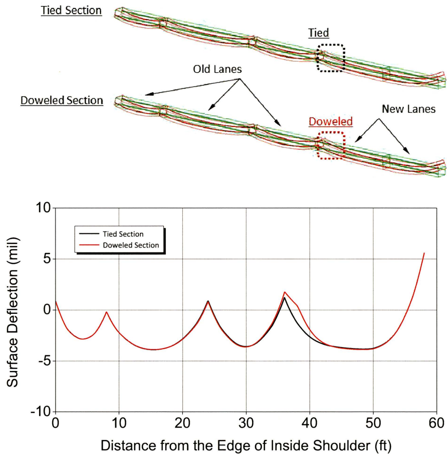
Figure 3.10: Deformed shape and surface deflection
