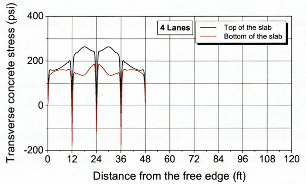
(b) Four-lane pavement
