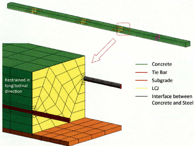
(a) Finite element mesh discretization of the tied and doweled sections
