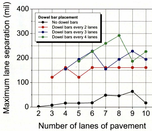
(a) Maximum lane separation
