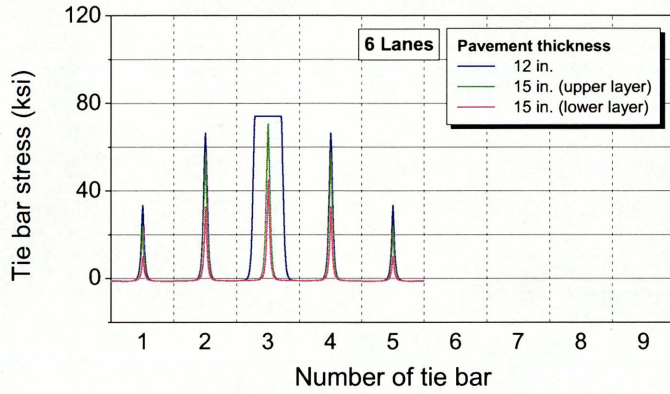
(a) Tie bar stress in six-lane pavement
