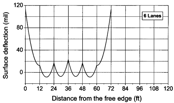
(c) Six-lane pavement
