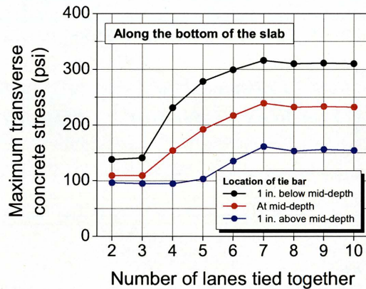
(f) Maximum concrete stress at the bottom of the slab
