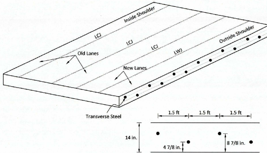
(b) Layout of transverse steels
