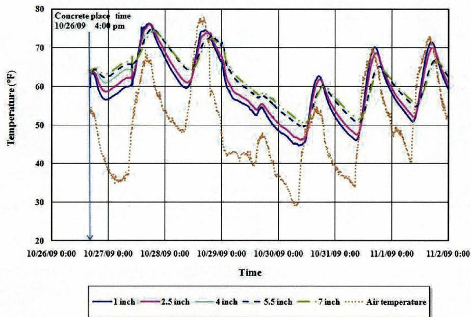
Figure 2.18: Temperature of different depths varied with time through the first week
