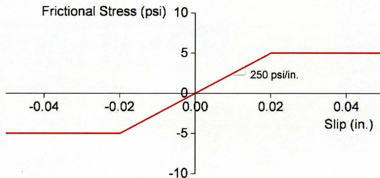
Figure 3.9: Friction-slip behavior between concrete and subgrade
