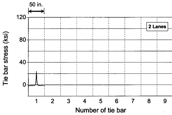
(a) Two-lane pavement
