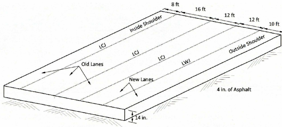
(a) Geometric configuration of the test section
