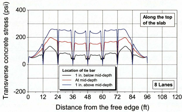
(c) Concrete stress along the top of the slab in eight-lane pavement
