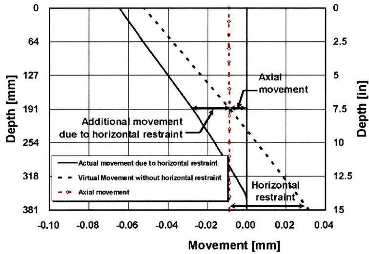
(b) Movement of concrete at construction joint in transverse direction
