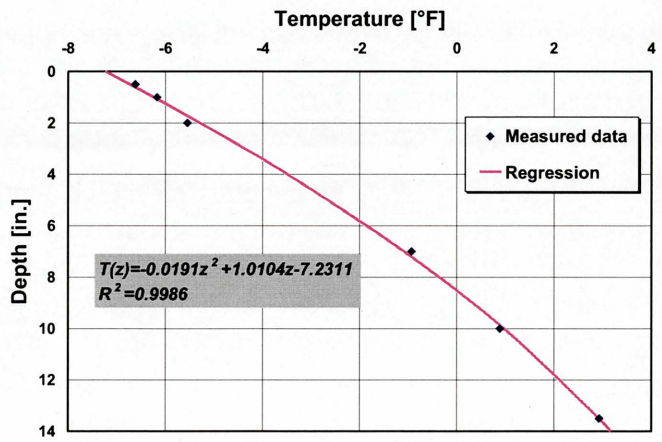
(b) Temperature gradient
