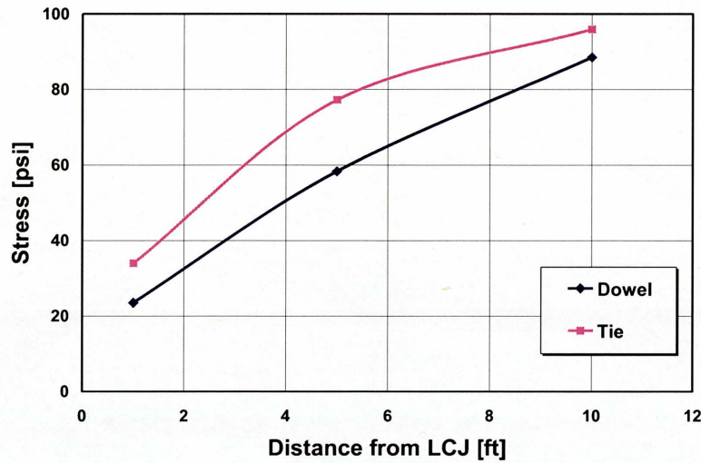
Figure 2.17: Transverse concrete stress
