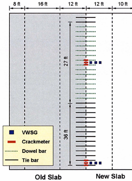
Figure 2.3: Field instrumentation
