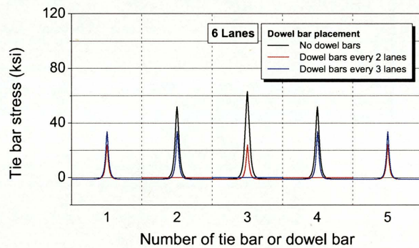
(b) Tie bar stress
