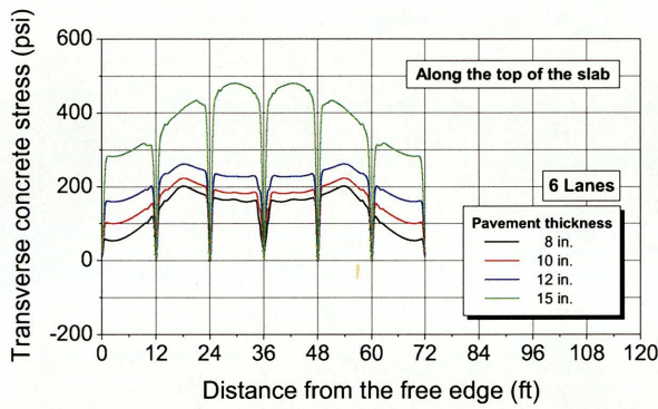
(c) Concrete stress along the top of the slab in six-lane pavement
