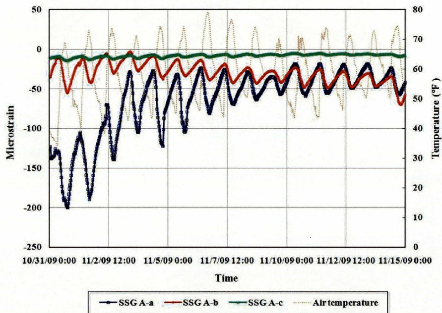
Figure 2.23: Strain of tie bar at A location
