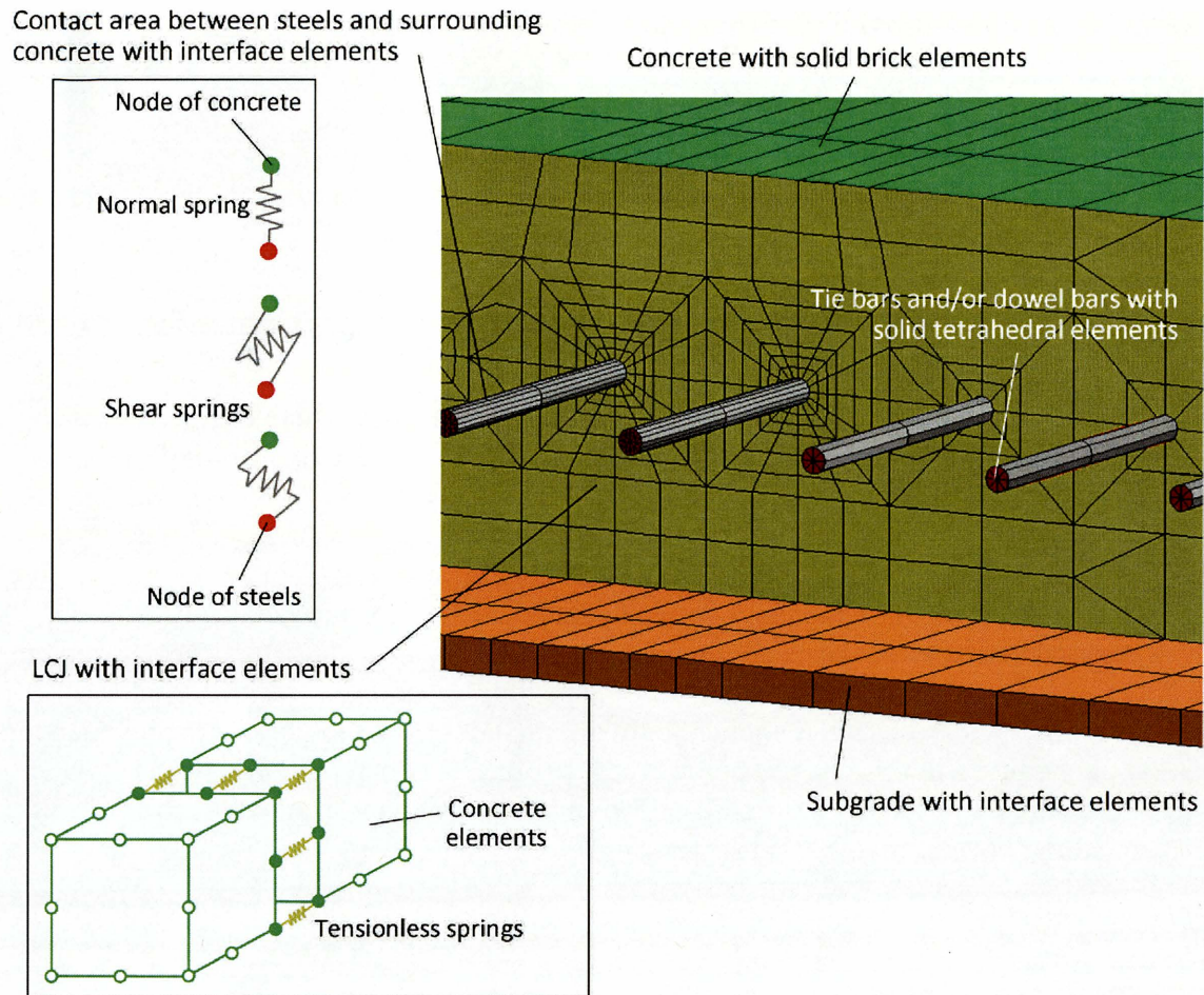
Figure 3.4: Three-dimensional finite element modeling of a concrete pavement
