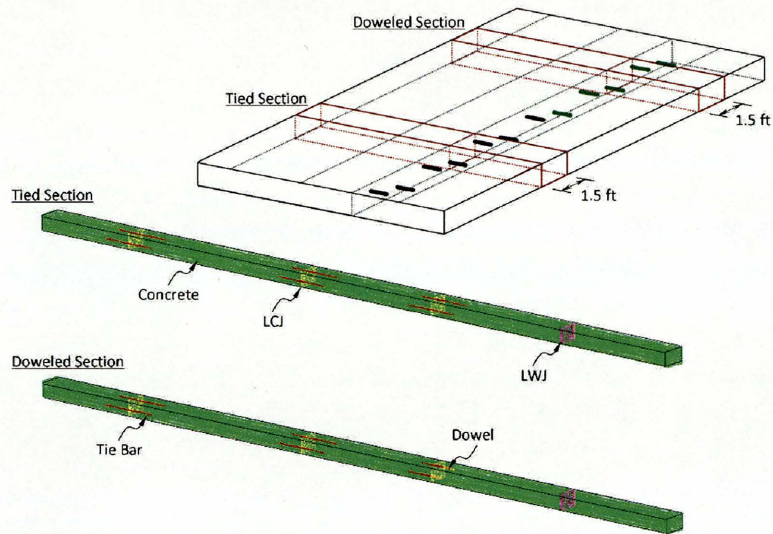
(a) Finite element mesh discretization of the tied and doweled sections
