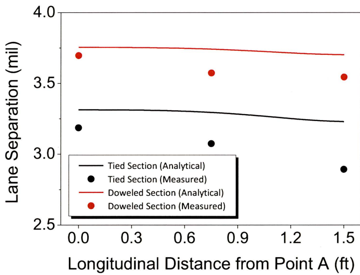
Figure 3.11: Transverse displacement across the LCJ between the existing and new slabs
