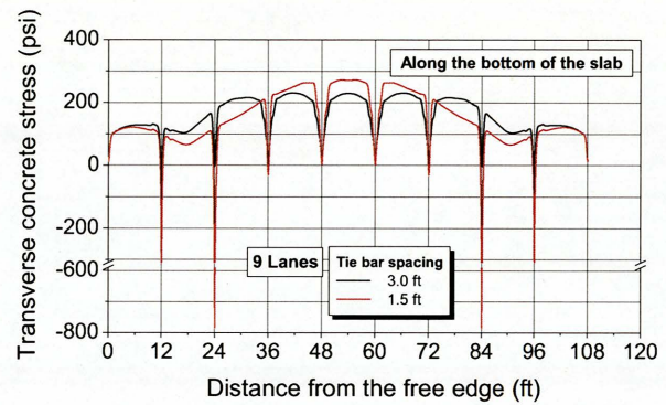
(d) Concrete stress along the bottom of the slab in nine-lane pavement
