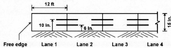
15 inch-thick pavement
