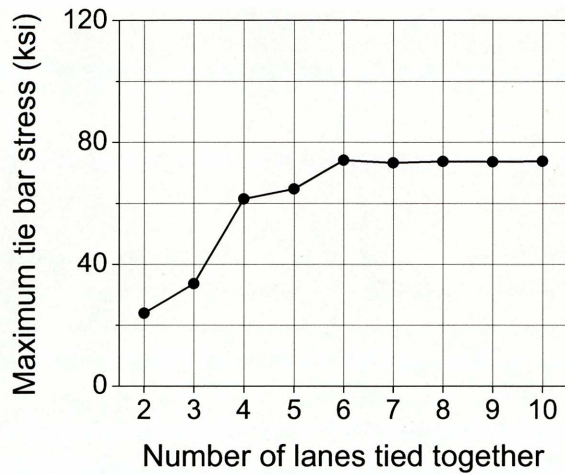
(a) Maximum tie bar stress
