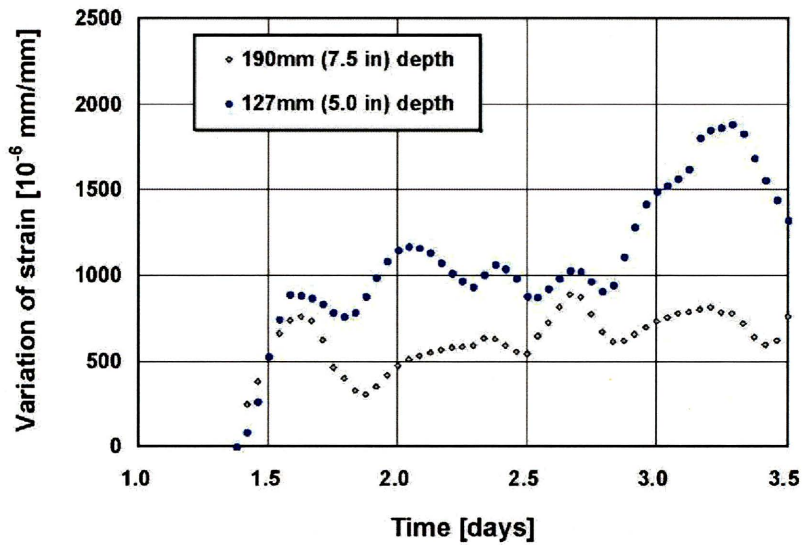
Figure 2.27: Effect of tie bar depth on tie bar strain
