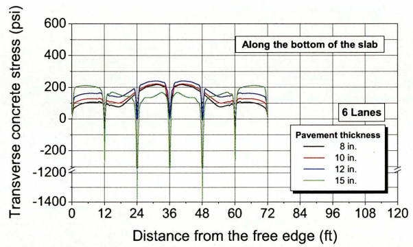
(d) Concrete stress along the bottom of the slab in six-lane pavement
