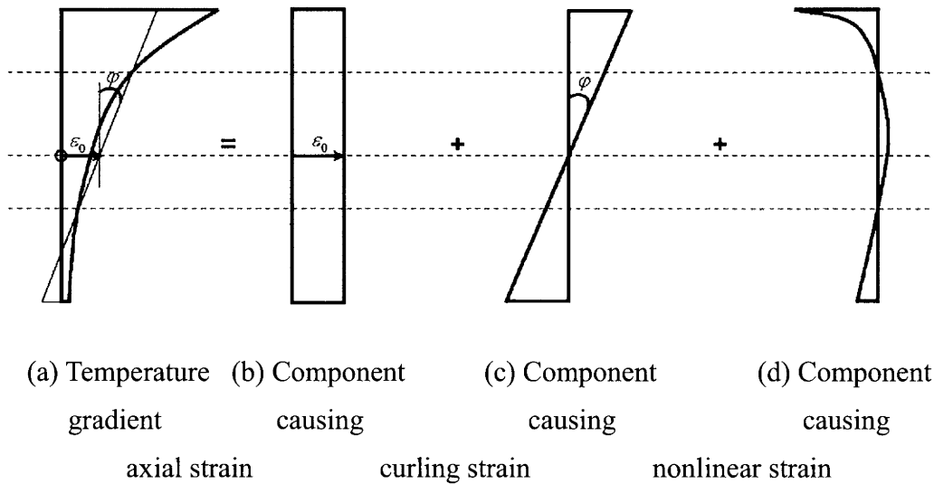
Figure 3.1: Decomposition of nonlinear temperature effects
