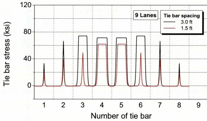
(a) Tie bar stress in nine-lane pavement
