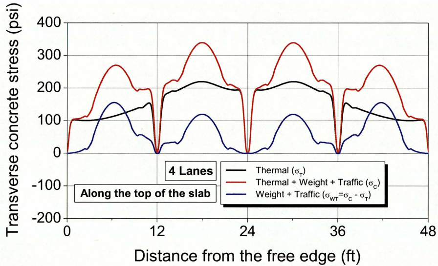
(b) Concrete stress along the top of the slab in four-lane pavement
