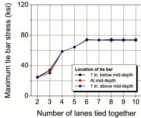
(b) Maximum tie bar stress
