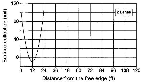
(a) Two-lane pavement
