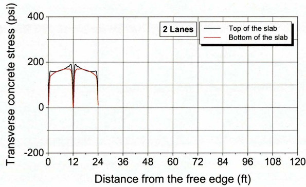
(a) Two-lane pavement
