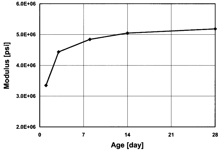
Figure 2.14: Measured elastic modulus of concrete
