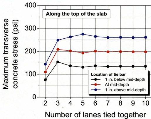
(e) Maximum concrete stress at the top of the slab
