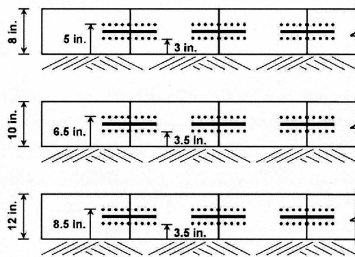
(b) Three levels of tie bar location
