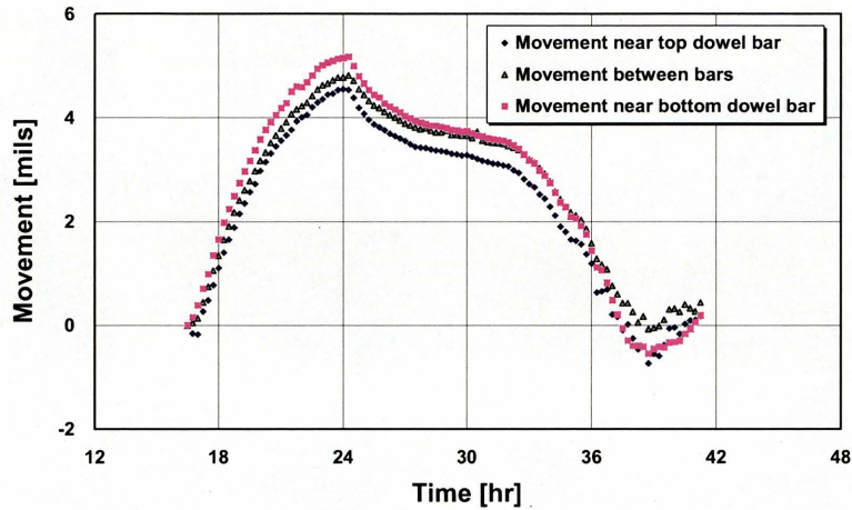
(a) Doweled section
