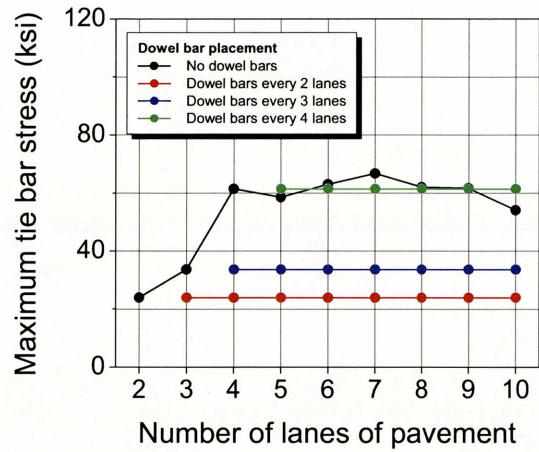
(b) Maximum tie bar stress
