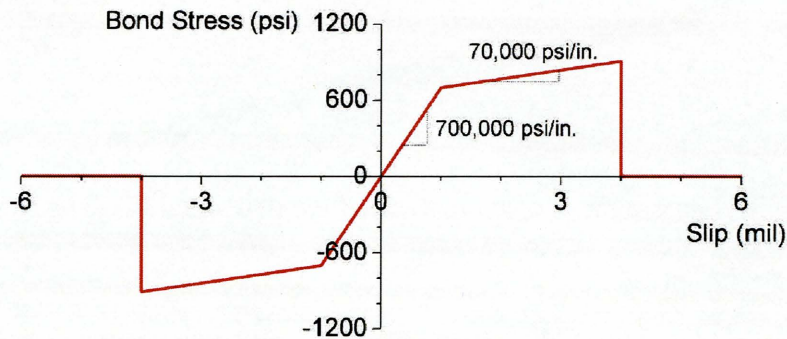
Figure 3.8: Bond-slip behavior between tie bars and surrounding concrete
