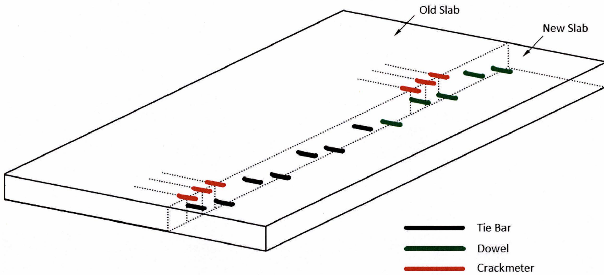
(b) Location of crackmeters
