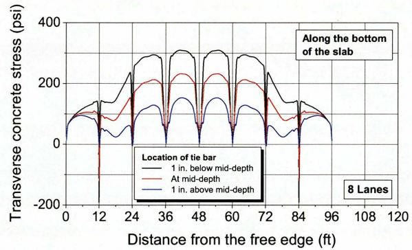
(d) Concrete stress along the bottom of the slab in eight-lane pavement
