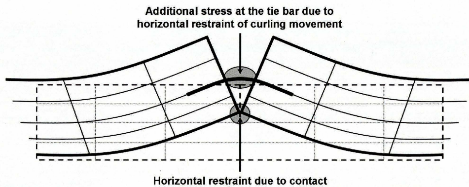
Figure 3.5: Restraining effect at the bottom of longitudinal construction joint
