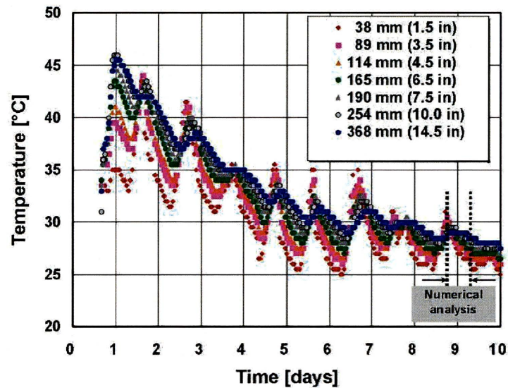
Figure 2.24: Measured concrete temperature
