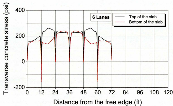
(c) Six-lane pavement
