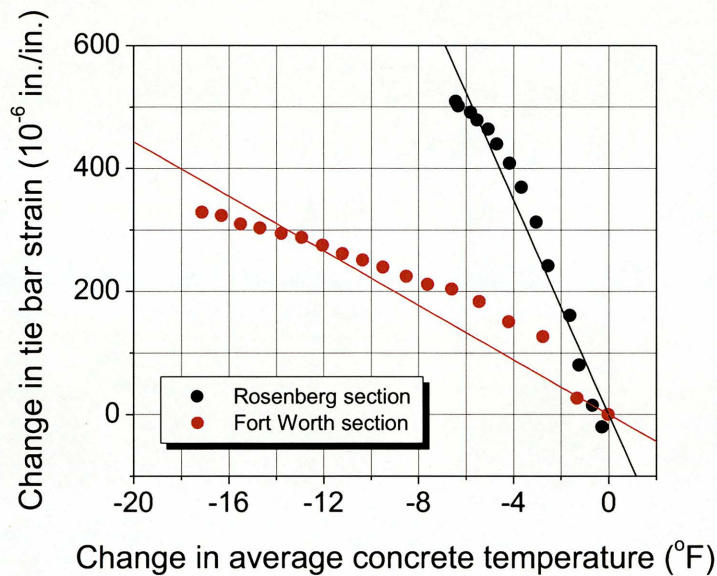
Figure 2.31: Change in average concrete temperature vs. change in tie bar strain
