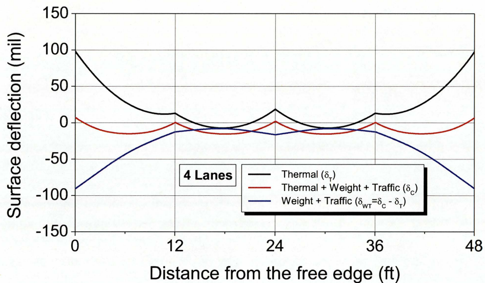
(a) Surface deflection in four-lane pavement
