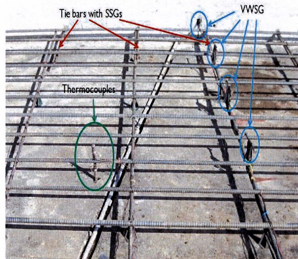
(b) Field layout of the instrumentations in the second-placed section
