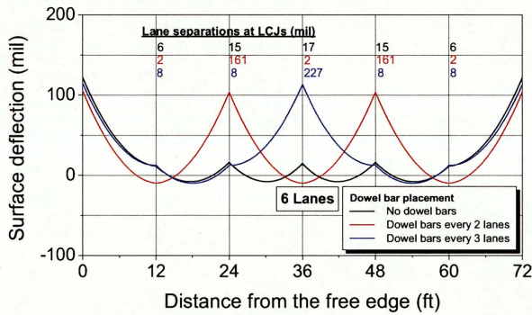
(a) Surface deflection and lane separation
