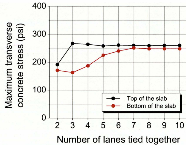
(b) Maximum transverse concrete stresses at the top and bottom of the slab
