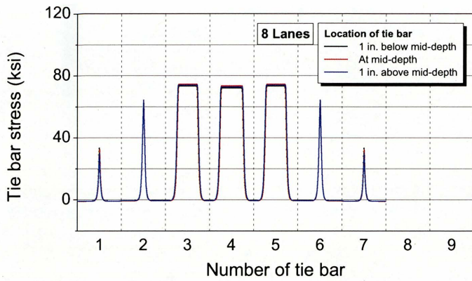
(a) Tie bar stress in eight-lane pavement
