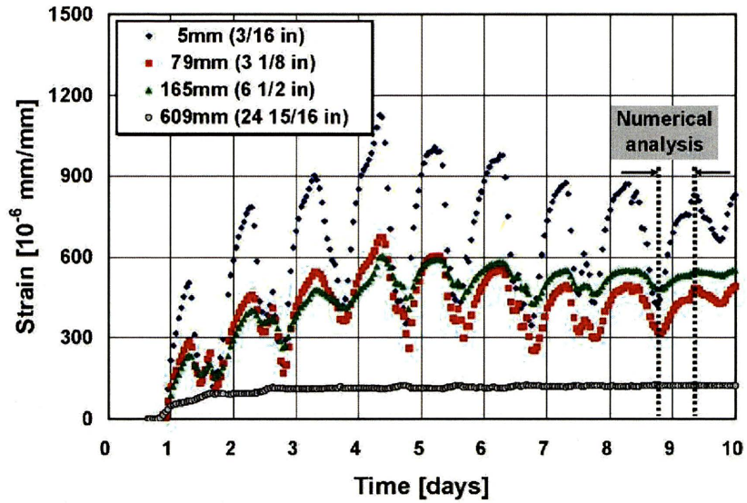
Figure 2.25: Measured steel strain
