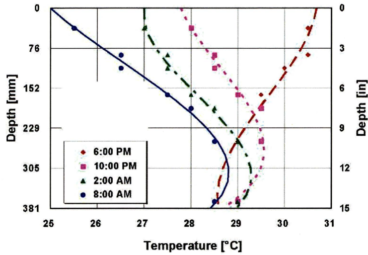
(a) Measured temperature profile at concrete slab from 8\frac{3}{4} to 9\frac{1}{3} days
