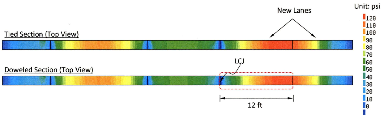
Figure 3.12: Transverse concrete stress at a depth of 1 in.
