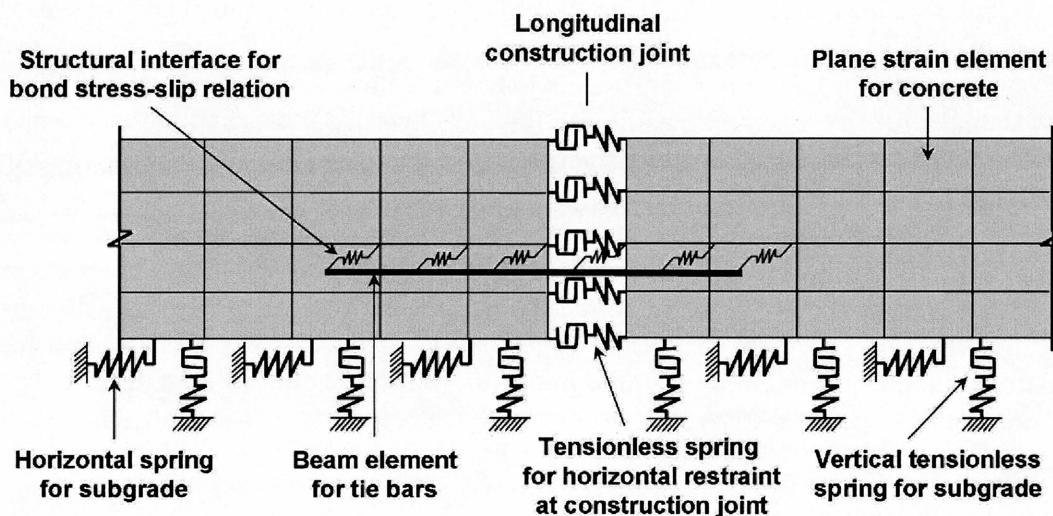
Figure 3.14: Two-dimensional finite element modeling of a concrete pavement
