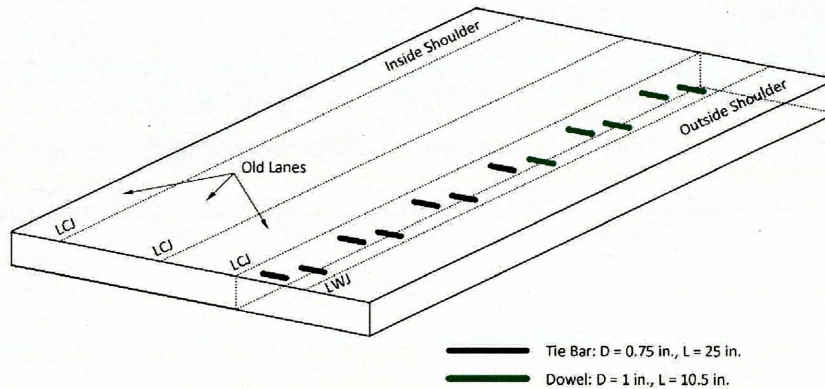
(c) Layout of tie bars and dowel bars
