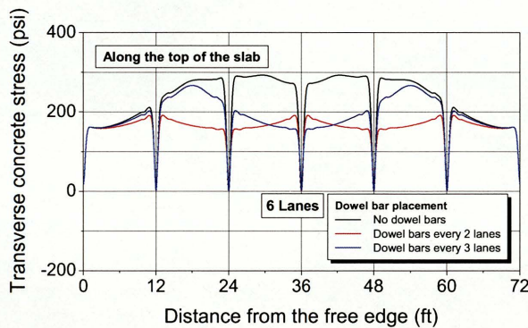
(c) Concrete stress along the top of the slab
