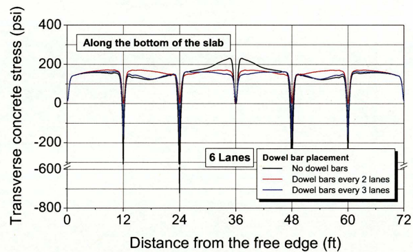
(d) Concrete stress along the bottom of the slab
