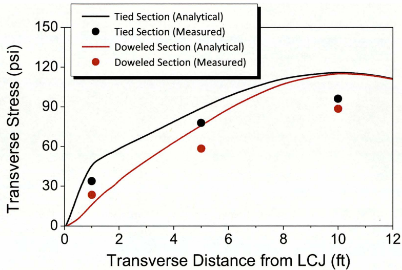
Figure 3.13: Transverse concrete stress in the outermost driving lane
