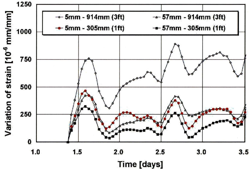
Figure 2.26: Effect of tie bar spacing on tie bar strain at different distances from LCJ
