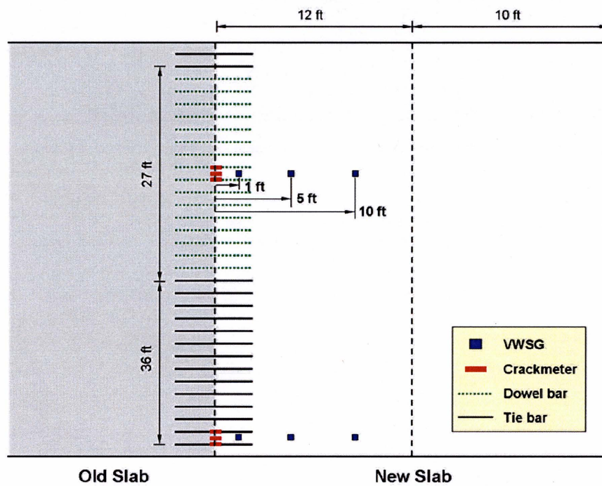
(b) Location of VWSGs
