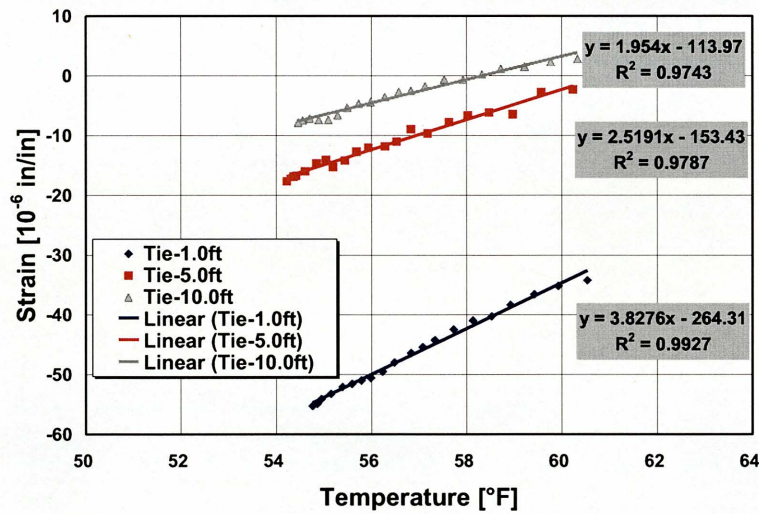
(b) Tied section
