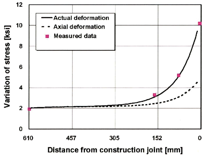
(a) Distribution of tie bar stress
