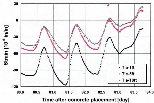
(b) Tied section
