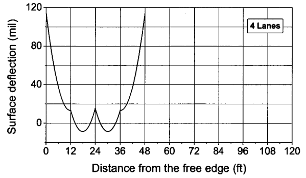
(b) Four-lane pavement
