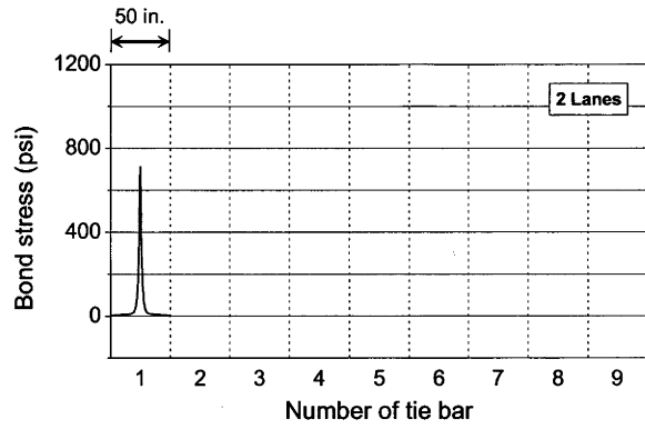
(a) Two-lane pavement
