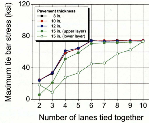
(b) Maximum tie bar stress
